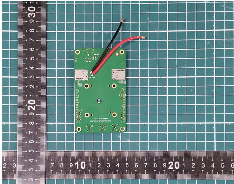
Picture 1: Radiated Spurious Emissions Test setup
