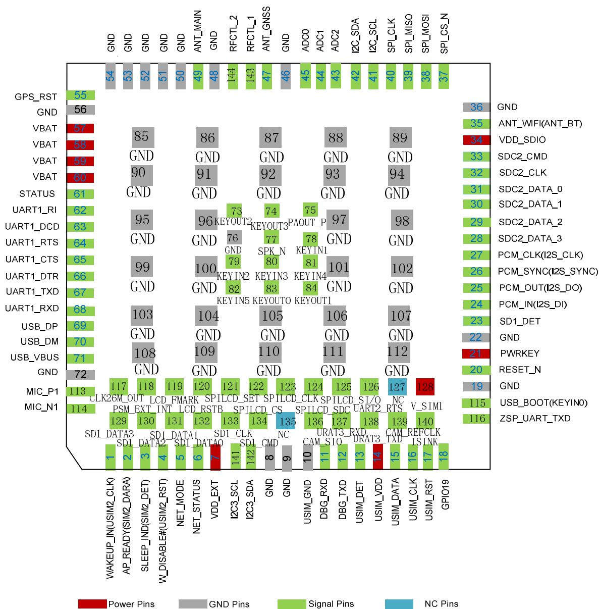
Figure 1 Module serial number pin diagram
