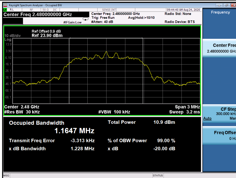
20 dB Bandwidth 2DH5 2480
