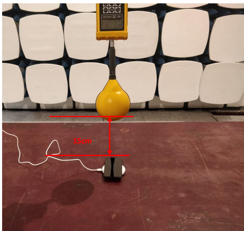
Test Position E-Exposure photo from top surface(15cm)
