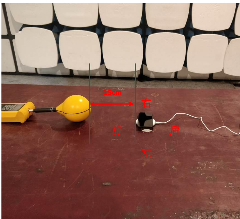
Test Position B-Exposure photo from side edge surface- Front
