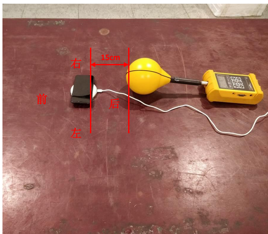
Test Position D-Exposure photo from side edge surface- Rear
