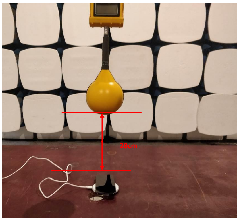
Test Position E-Exposure photo from top surface(20cm)
