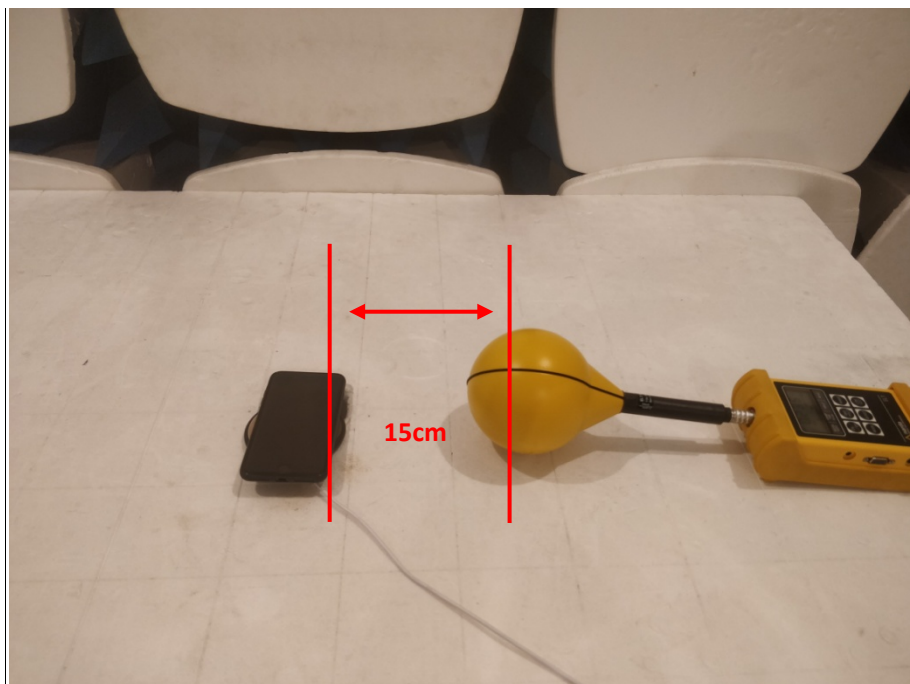
Test Position B-Exposure photo from side edge surface-Right
