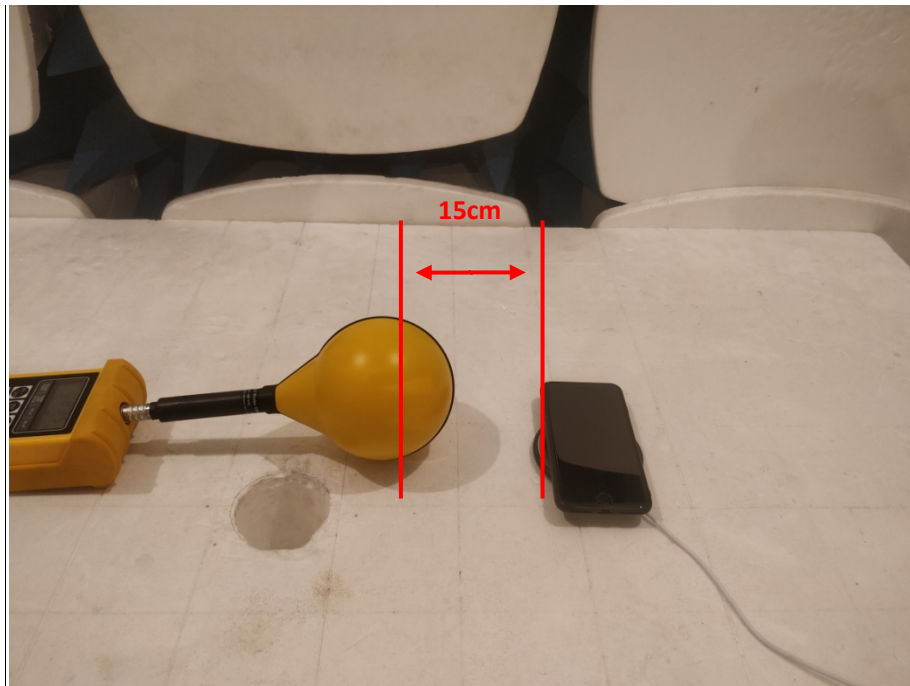
Test Position A-Exposure photo from side edge surface-Left
