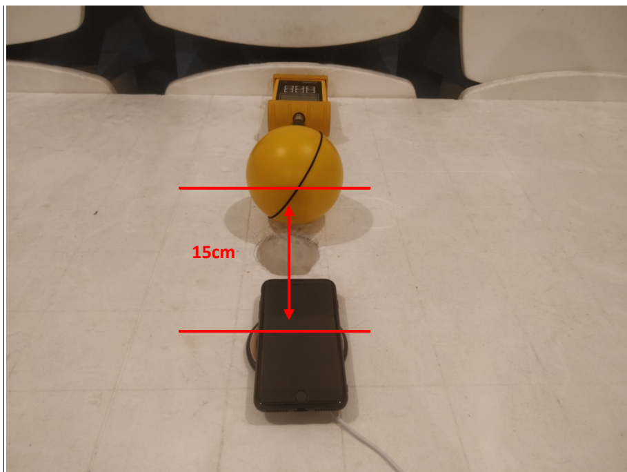
Test Position D-Exposure photo from side edge surface-Rear
