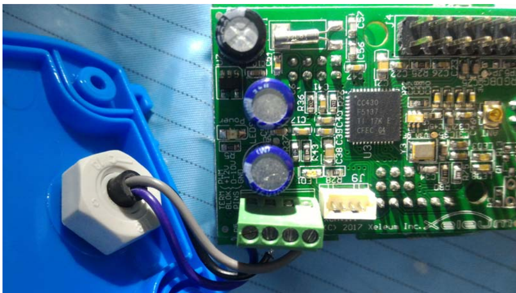
EUT – Main IC Chip View
