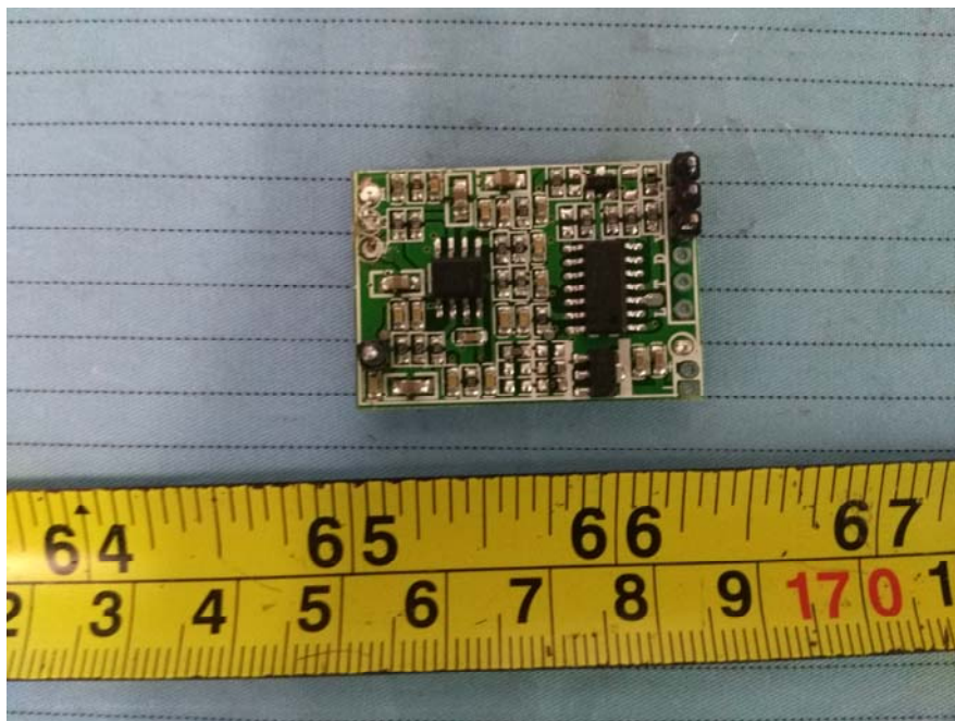
EUT – 5.8GHz Module Main Board 1 Top View
