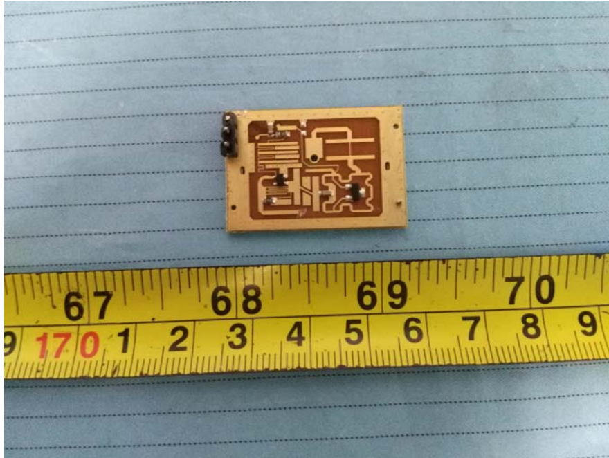
EUT – 5.8GHz Module Main Board 2 Top Cover off View
