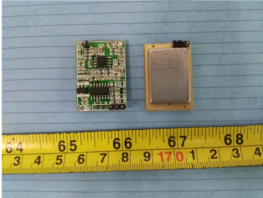
EUT – 5.8 GHz Module Cover off View
