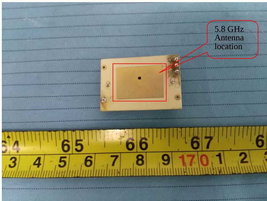
EUT – 5.8GHz Module Main Board 2 Bottom View
