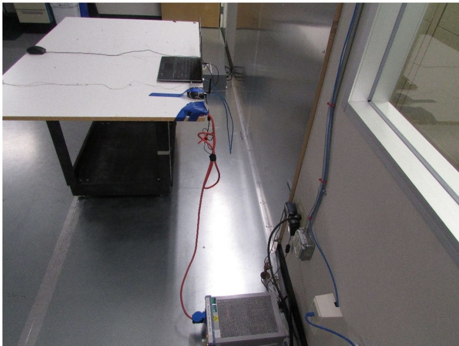
Figure 8: Conducted Emissions
