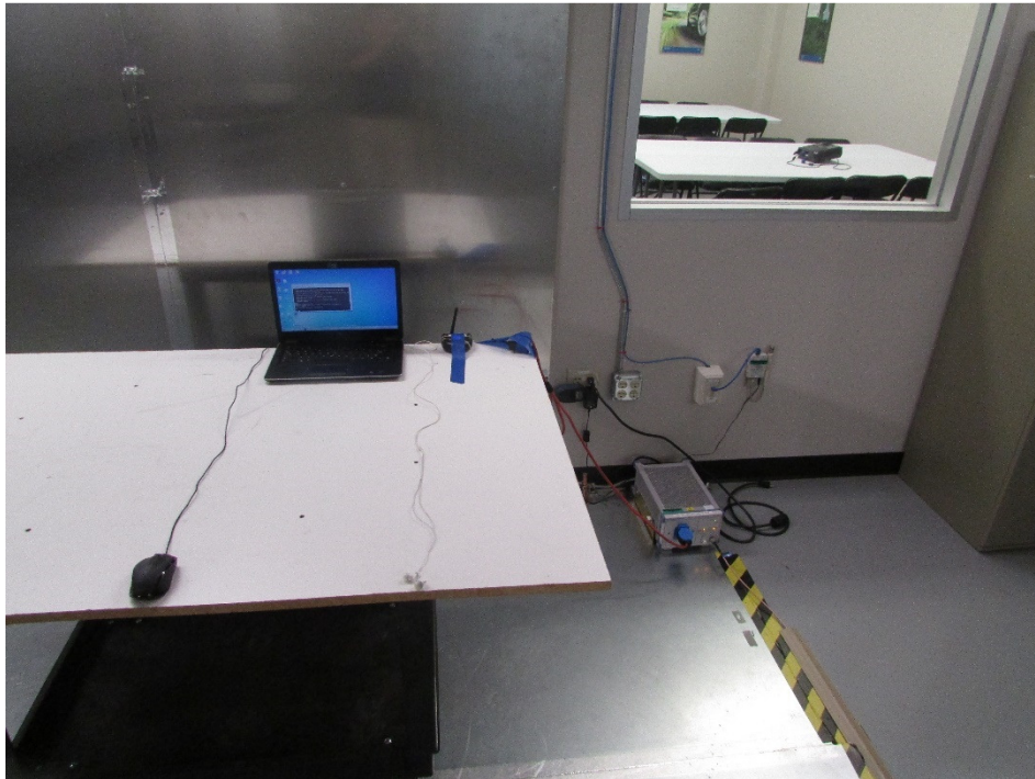
Figure 7: Conducted Emissions
