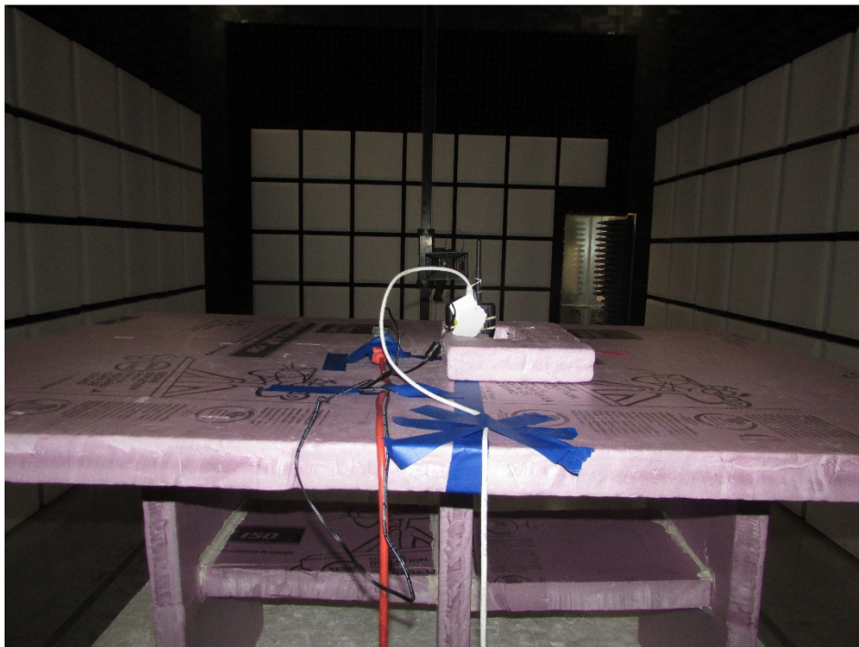
Figure 6: Radiated Emissions – Back – Above 1GHz – ZPOS
