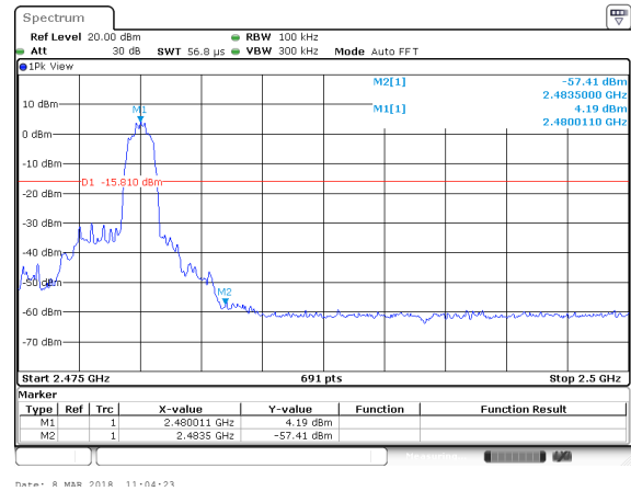
\pi /4-DQPSK: Band Edge-High Channel (Hopping Mode)
