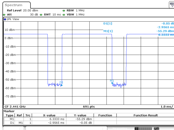
Package Transfer Time Plot CH39-DH5
