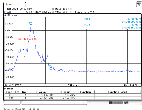
GFSK: Band Edge-High Channel (Hopping Mode)
