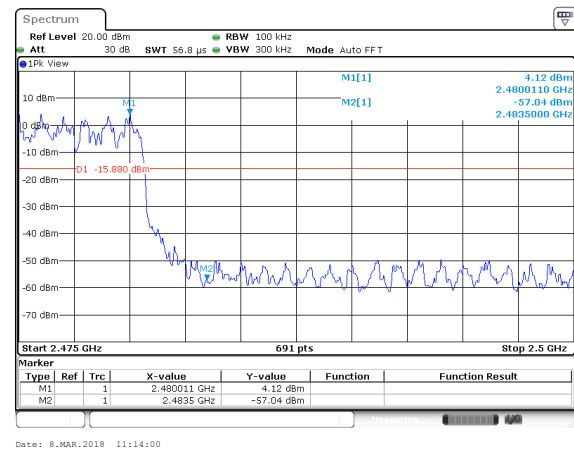
8-DPSK: Band Edge-High Channel (Hopping Mode)
