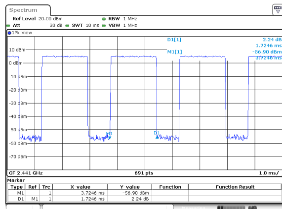
Package Transfer Time Plot CH39-2DH3
