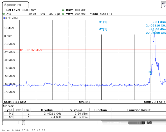
8-DPSK: Band Edge-Low Channel (Hopping Mode)
