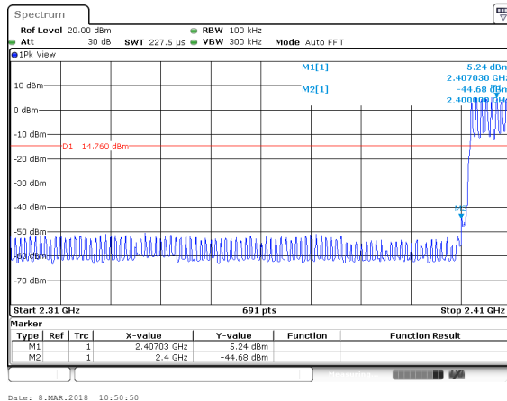
GFSK: Band Edge-Low Channel (Hopping Mode)
