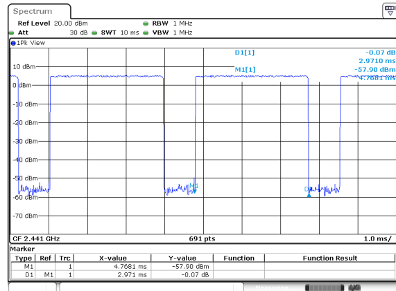
Package Transfer Time Plot CH39-2DH5
