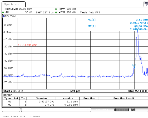
\pi /4-DQPSK: Band Edge-Low Channel (Hopping Mode)
