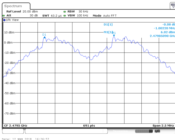
(1Mbps) Channel Separation plot on channel 77-78
