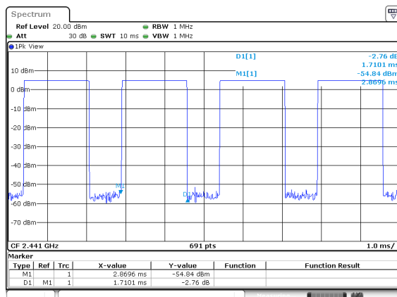
Package Transfer Time Plot CH39-DH3
