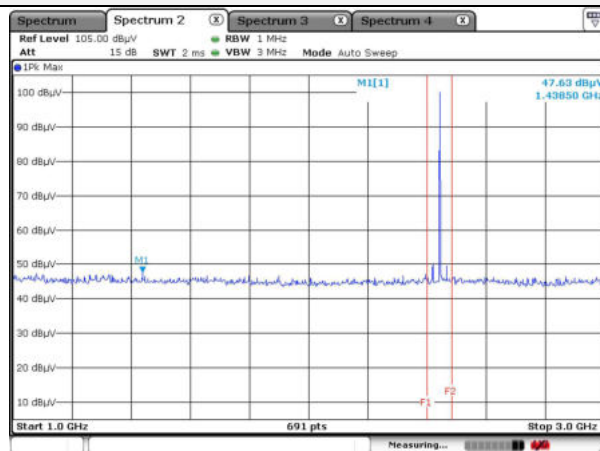
Horizontal // Peak for 1 to 3
