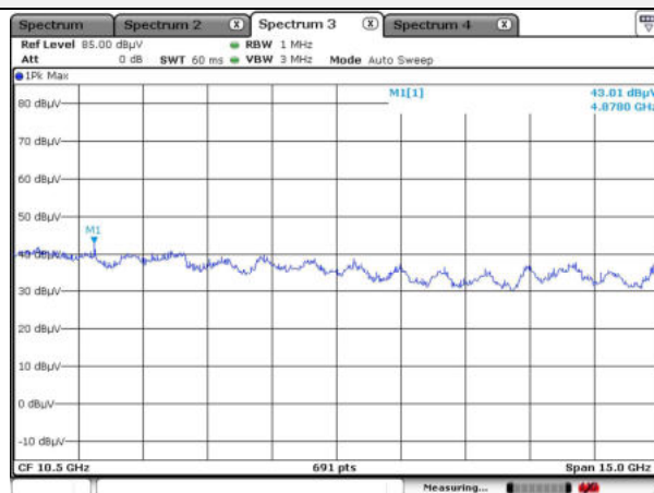
Horizontal // Peak for 3 to 18
