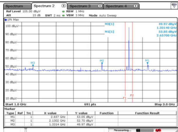
Vertical // Peak for 1 to 3
