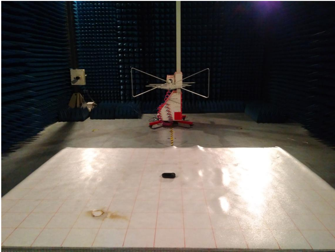
Radiated Emission
