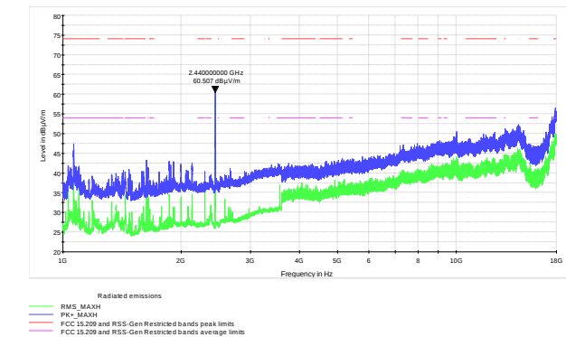
Figure 8.4-10: Radiated spurious emissions above 1 GHz for mid channel
