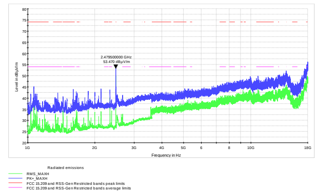
Figure 8.4-11: Radiated spurious emissions above 1 GHz for high channel
