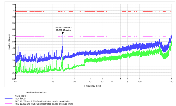
Figure 8.4-9: Radiated spurious emissions above 1 GHz for low channel
