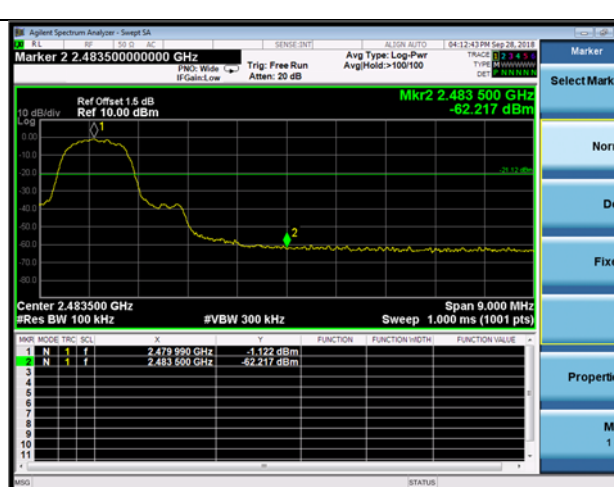
DQPSK,2480MHz,2DH5,Plot 1,Band Edge
