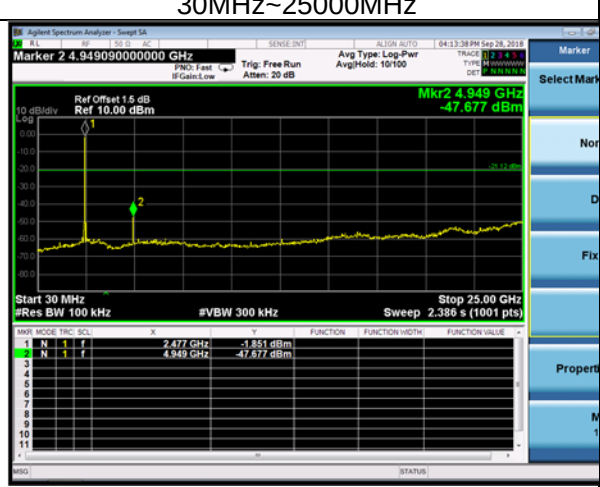
DQPSK,2480MHz,2DH5,Plot 2, 30MHz~25000MHz
