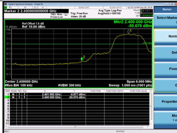
DQPSK,2402MHz,2DH5,Plot 1,Band Edge
