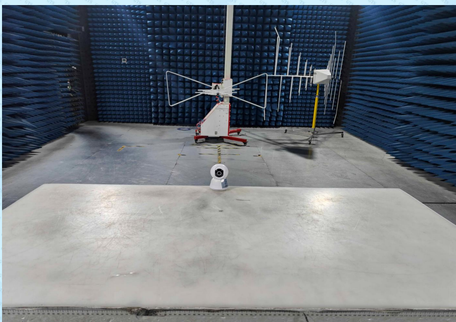
Radiated Emission Below 1GHz Test Setup
