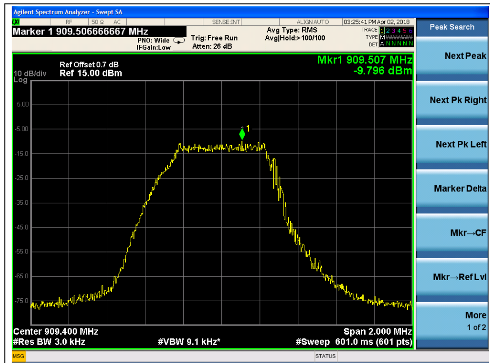
(500 kHz BW, Mid Channel, 909.4MHz)
