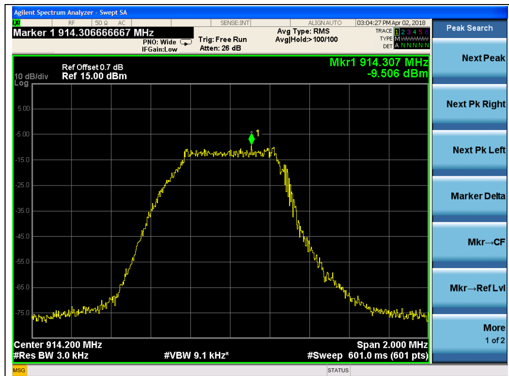
(500 kHz BW, High Channel, 914.2MHz)
