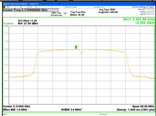
W53_11n40_Higher_Power Spectrum Density
