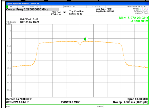
W53_11n40_Lower_Power Spectrum Density
