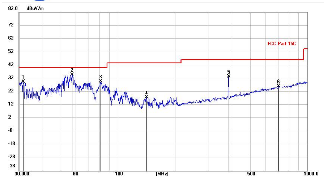
(802.11b _2472MHz, Antenna Vertical, 30MHz to 1GHz)
