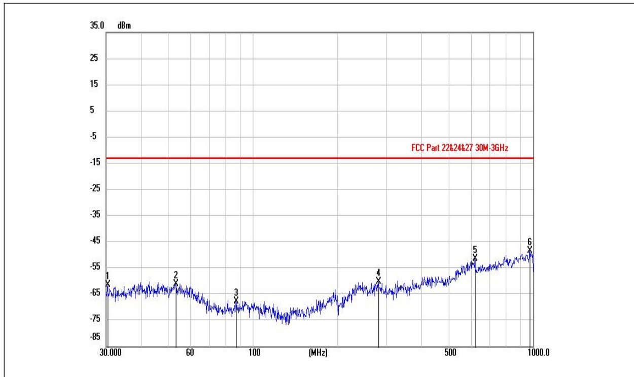
(1xEVDO Rev A BC 1 _ CH 600 _ 30MHz to 1GHz _ Horizontal)
