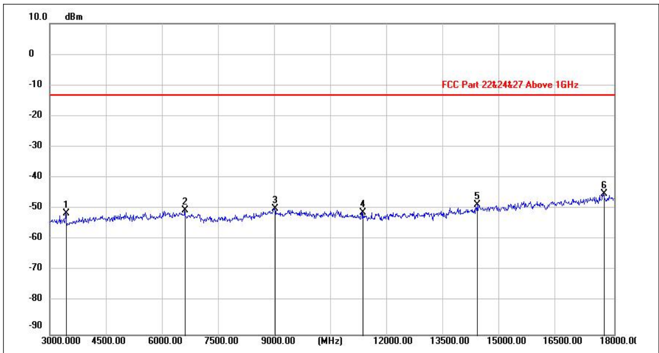
(WCDMA Band IV_ 3GHz to 18GH _ Low Channel z _ Vertical)
