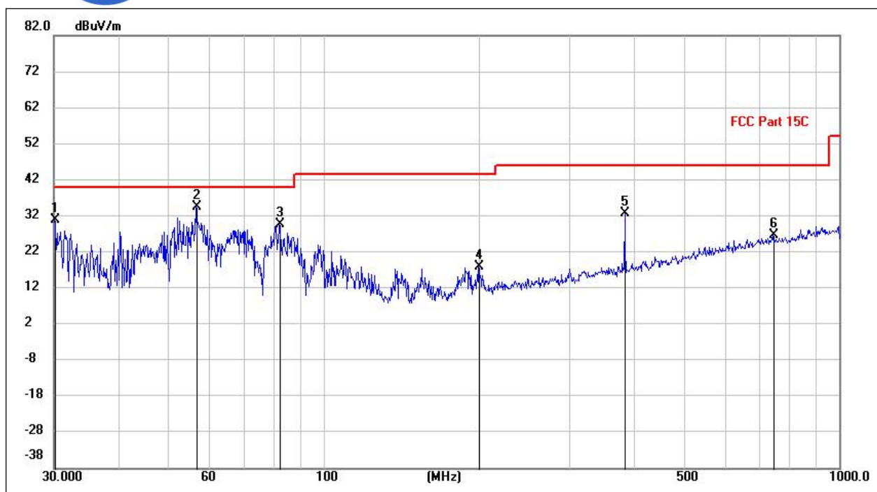
(802.11n _5785MHz, Antenna Vertical, 30MHz to 1GHz)
