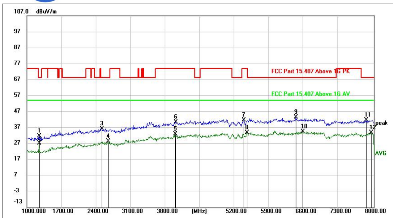
(802.11n_5240MHz, Antenna Vertical, 1GHz to 8GHz)
