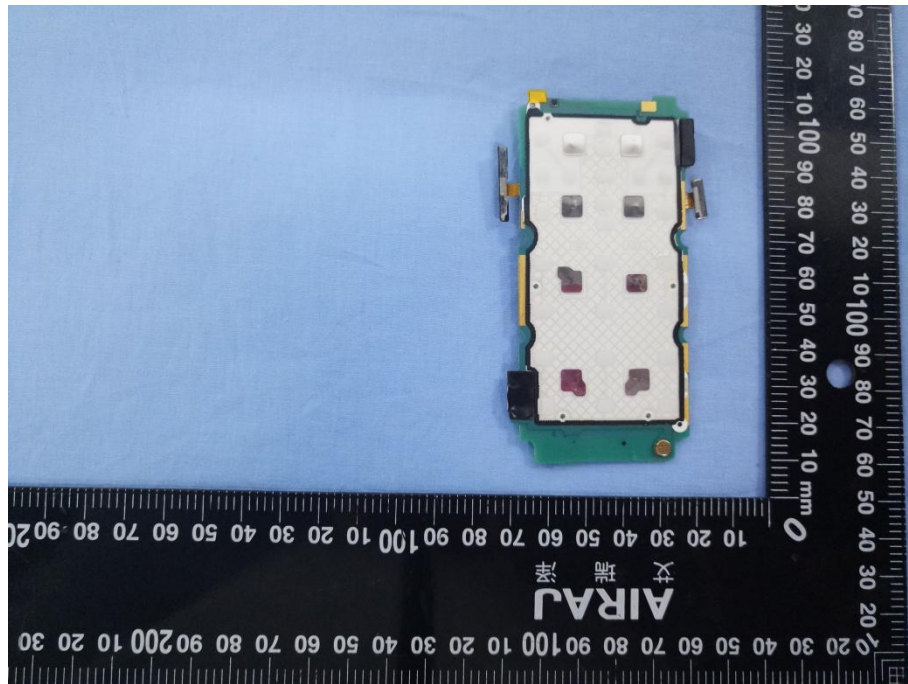
4. Subboard top view
