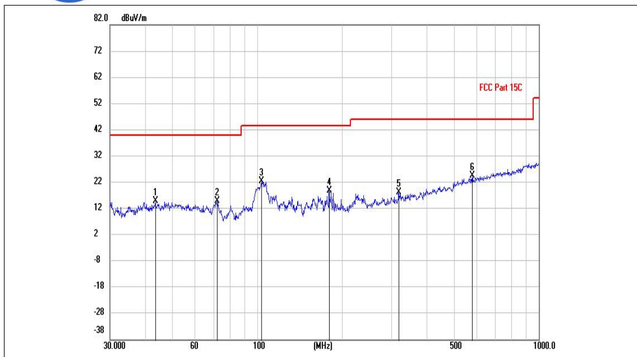
(802.11g _2462MHz, Antenna Horizontal, 30MHz to 1GHz)
