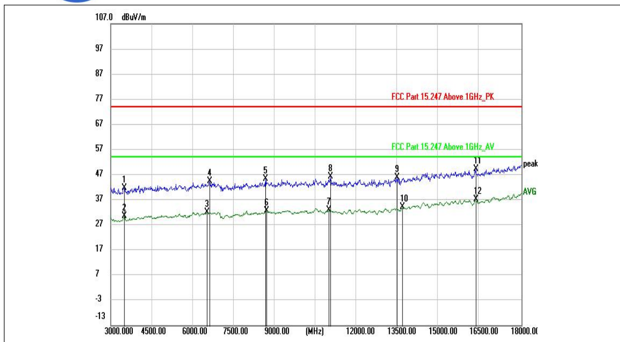
(802.11n_20M_2467MHz, Antenna Vertical, 3GHz to 18GHz)
