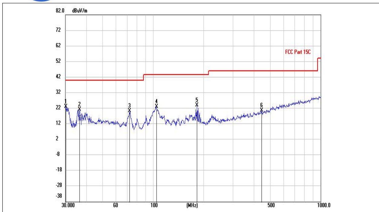
(802.11g _2437MHz, Antenna Horizontal, 30MHz to 1GHz)
