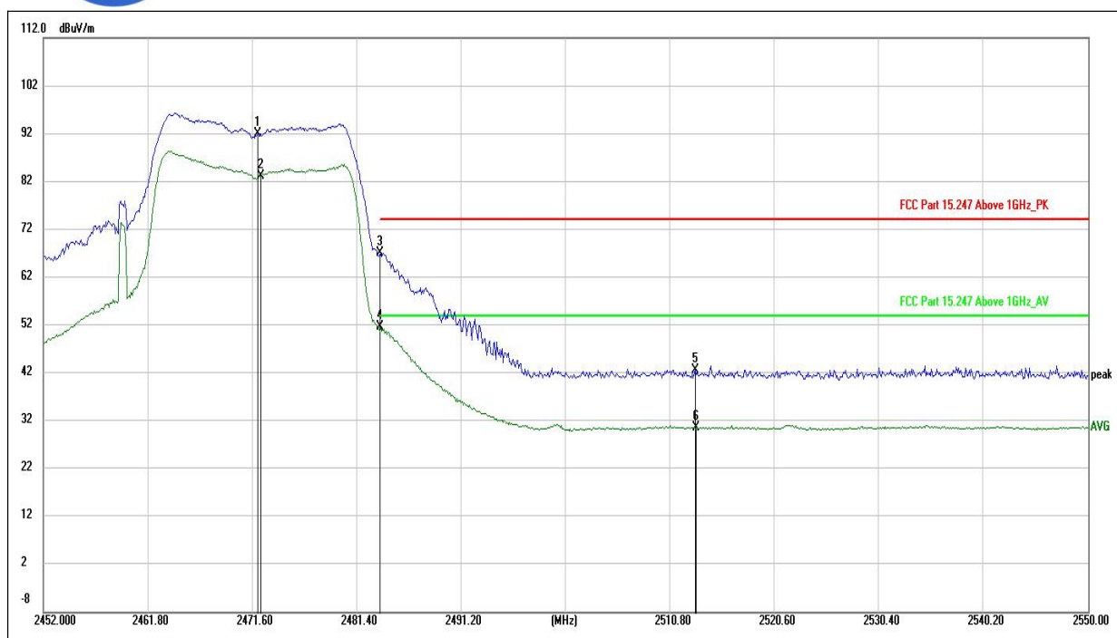
(802.11n_20M_2472MHz, Antenna Horizontal)
