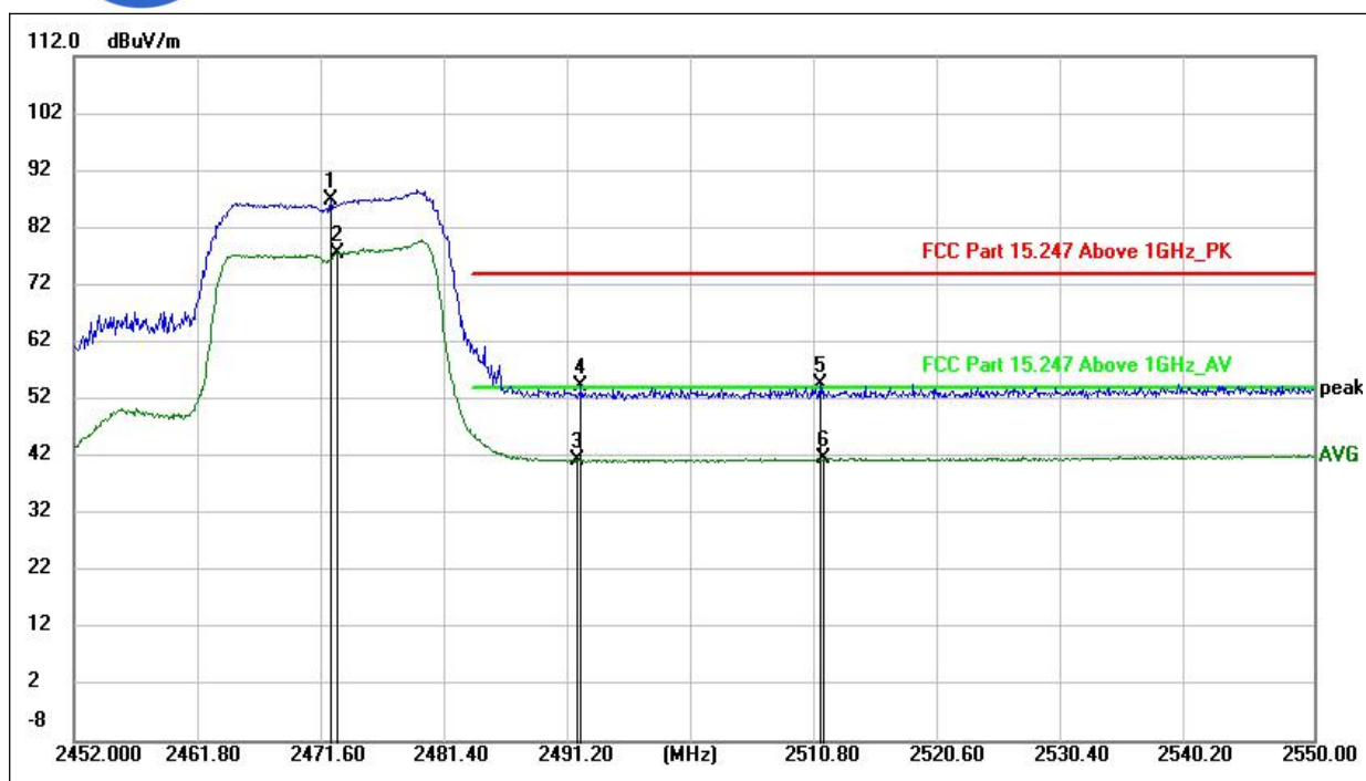
(802.11g _2472MHz, Antenna Vertical)
