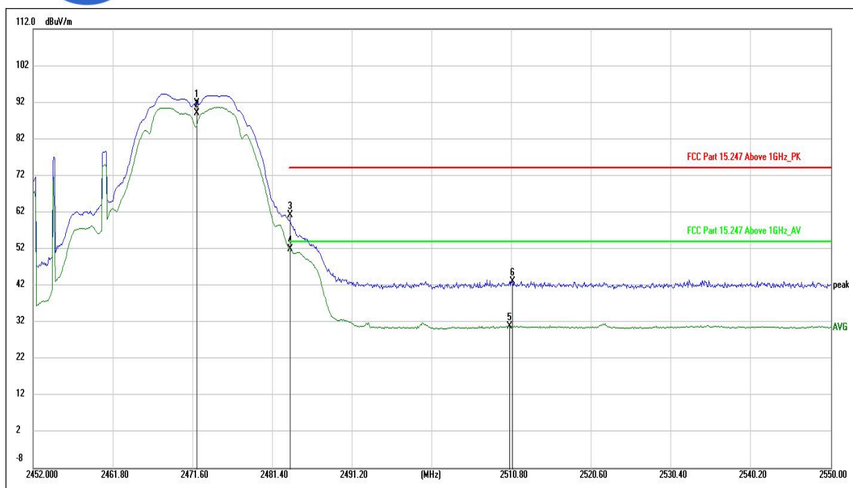
(802.11b_2472MHz, Antenna Horizontal)
