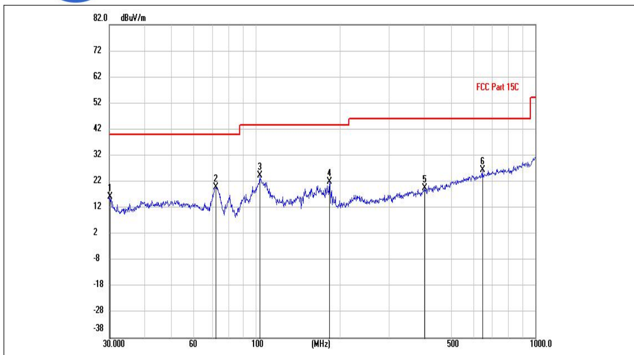
(802.11b_2437MHz, Antenna Horizontal, 30MHz to 1GHz)
