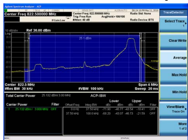
LTE Band 26 QPSK 1RB 3MHz CH High
