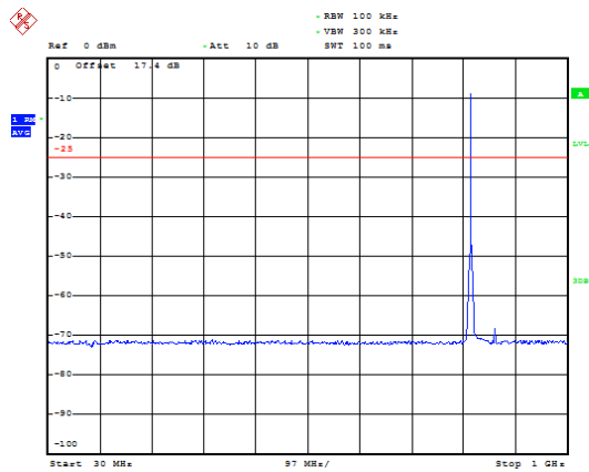
LTE Band 26 1.4MHz CH Middle 30MHz~1GHz
