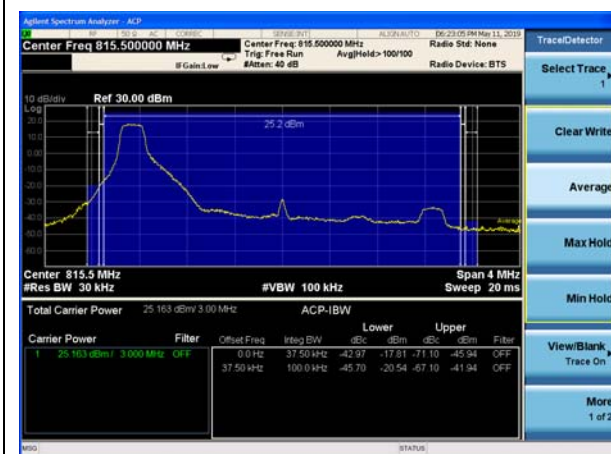
LTE Band 26 QPSK 1RB 3MHz CH Low
