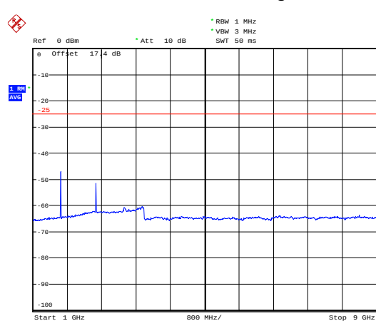
LTE Band 26 1.4MHz CH High 1GHz~9GHz
