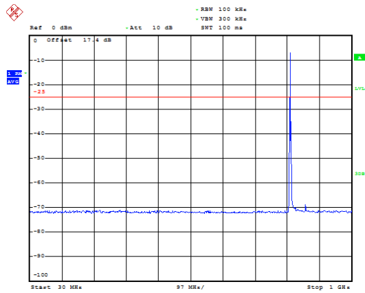
LTE Band 26 1.4MHz CH Low 30MHz~1GHz
