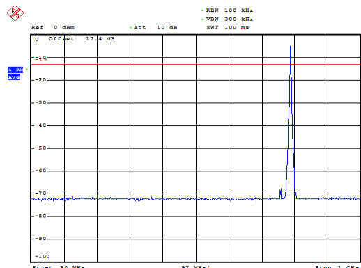
LTE Band 14 5MHz CH- Middle 30MHz~1GHz
