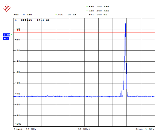
LTE Band 14 5MHz CH-High 30MHz~1GHz
