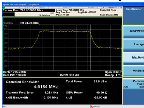
LTE Band 14 QPSK 5MHz CH-High
