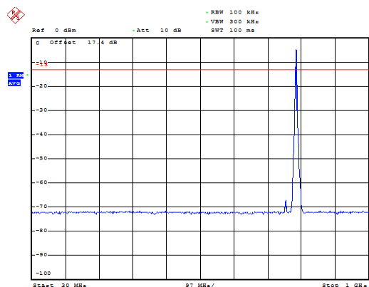
LTE Band 14 5MHz CH-Low 30MHz~1GHz
