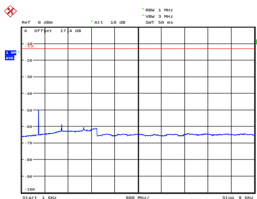
LTE Band 14 5MHz CH-Low 1GHz~9GHz
