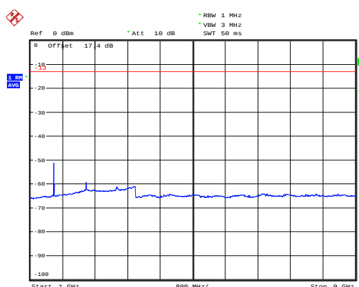
LTE Band 14 5MHz CH- Middle 1GHz~9GHz
