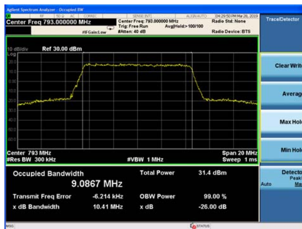
LTE Band 14 QPSK 10MHz CH-Middle
