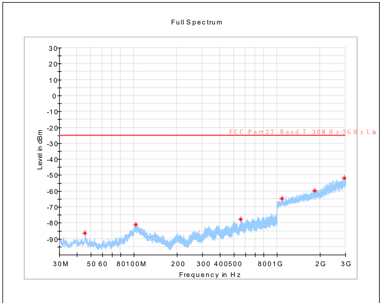
(LTE Band 7 _ QPSK_ Low Channel _ 30MHz to 3GHz _ Vertical)
