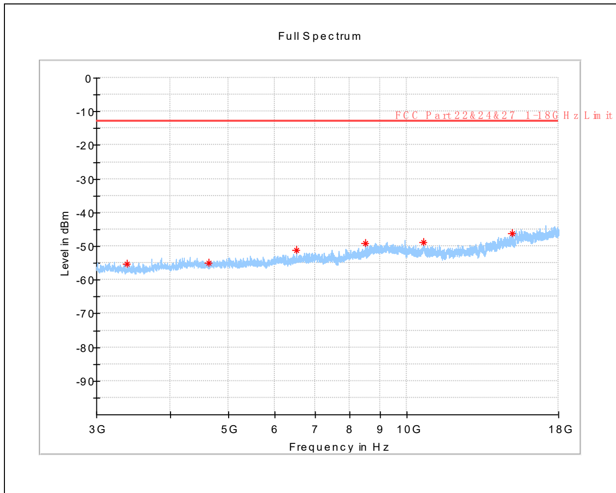
(LTE Band 66 _ QPSK_ High Channel _ 3GHz to 18GHz _ Vertical)
