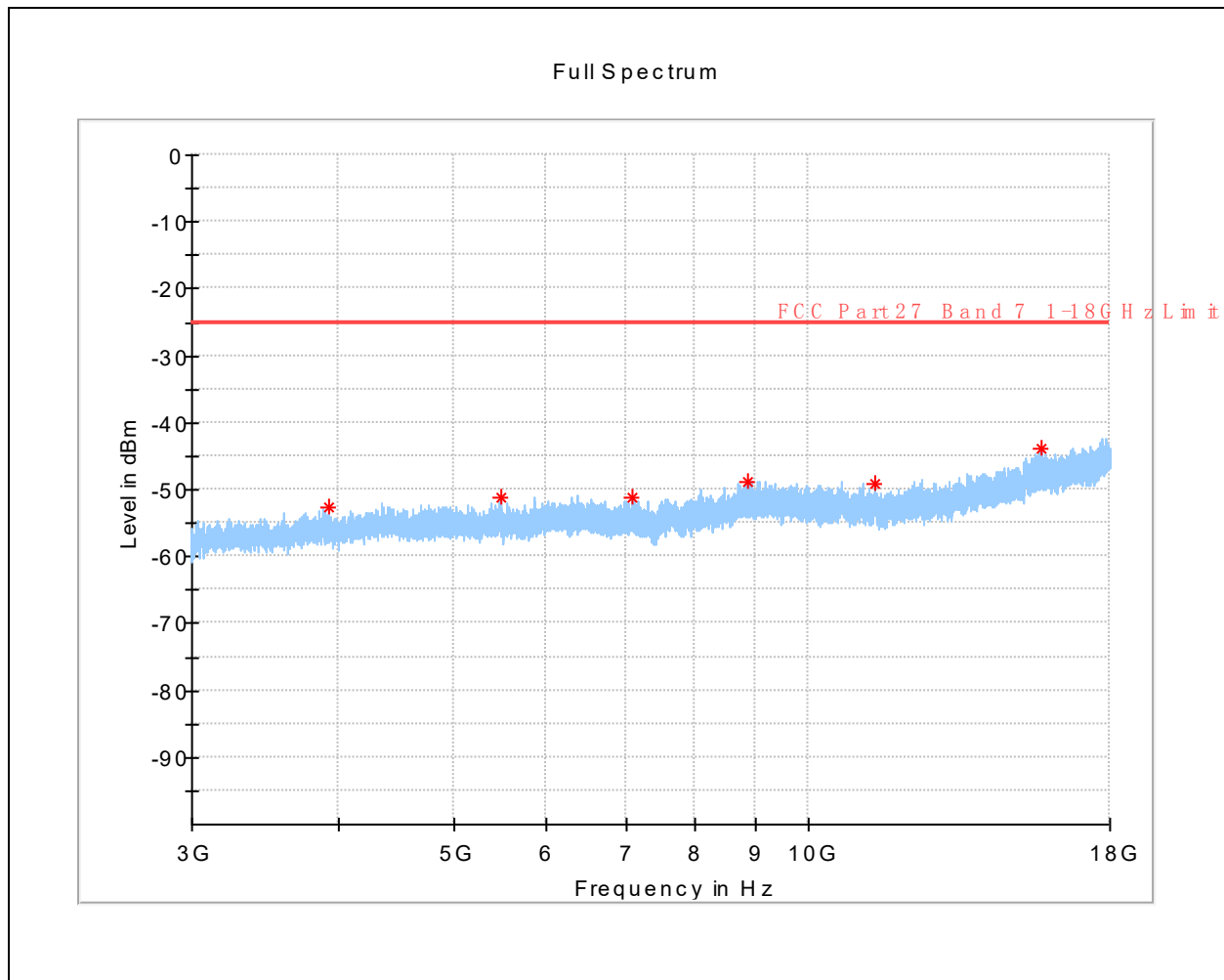
(LTE Band 7 _QPSK_ High Channel _ 3GHz to 18GHz _ Horizontal)
