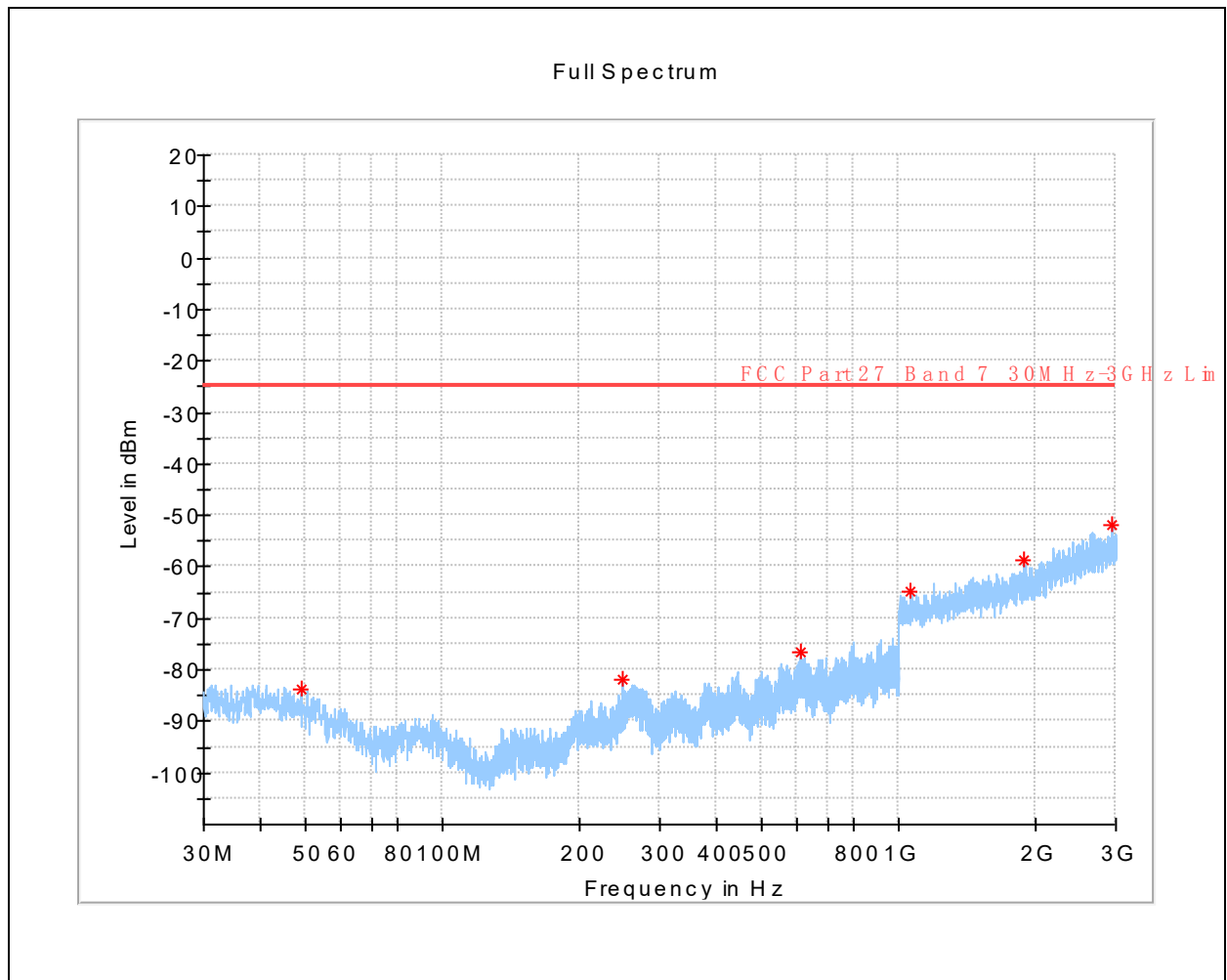
(LTE Band 7 _QPSK_ Low Channel _ 30MHz to 3GHz _ Horizontal)
