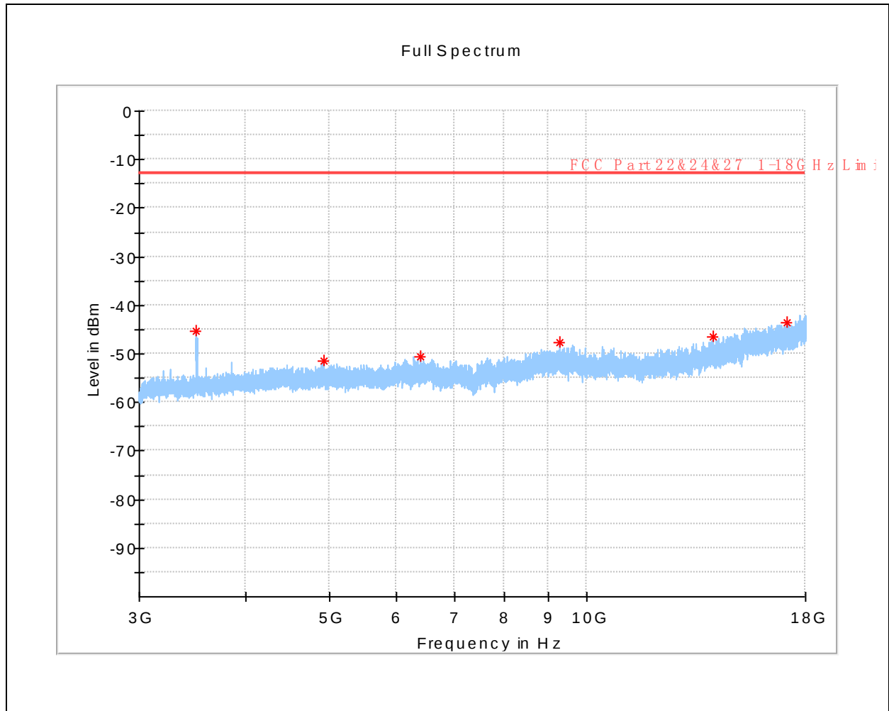
(LTE Band 4 _QPSK_ High Channel _ 3GHz to 18GHz _ Horizontal)
