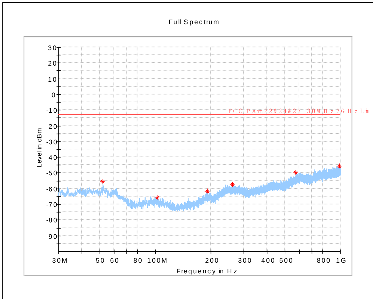
(WCDMA Band V _ Low Channel _ 30MHz to 1GHz _ Horizontal)
