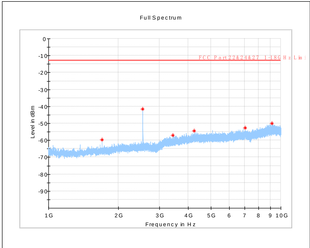
(GSM 850MHz _ High Channel _ 1GHz to 10GHz _ Vertical)
