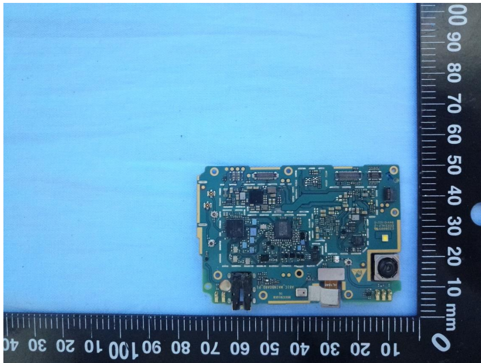
7、main board bottom view
