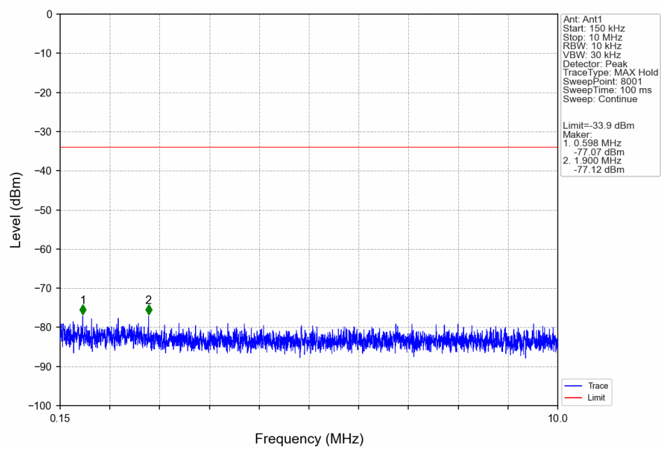
1M_MCH_2440MHz_Ant1_NTNV
