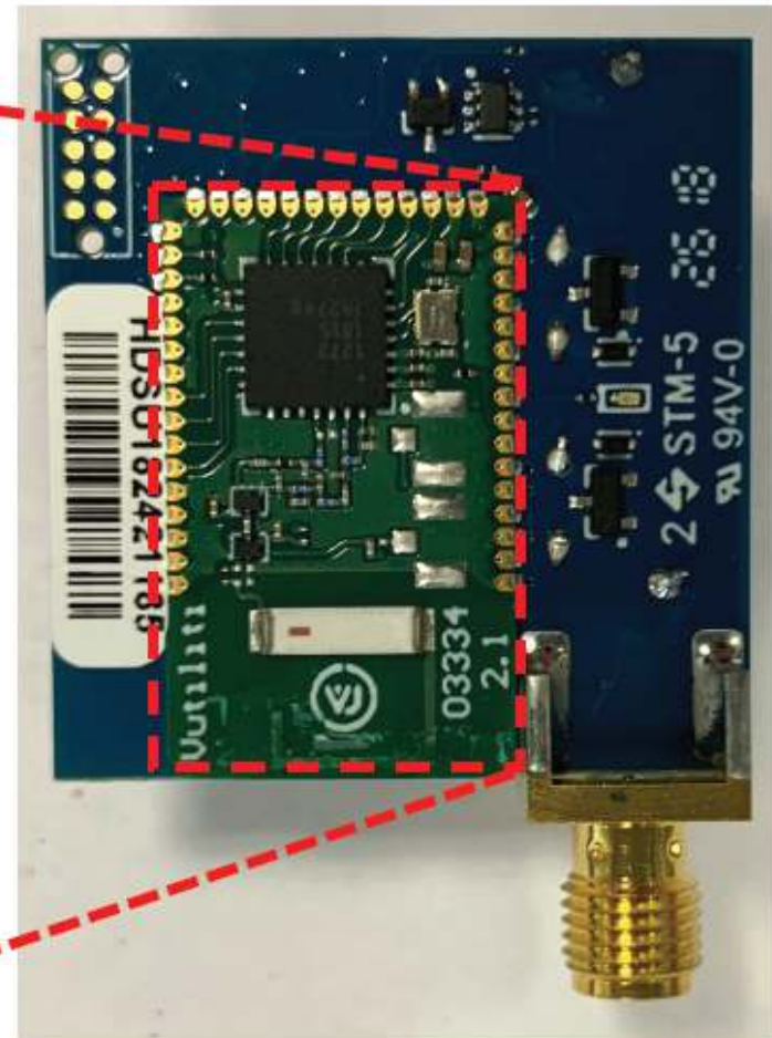
Host Carrier & Module Board: Top
