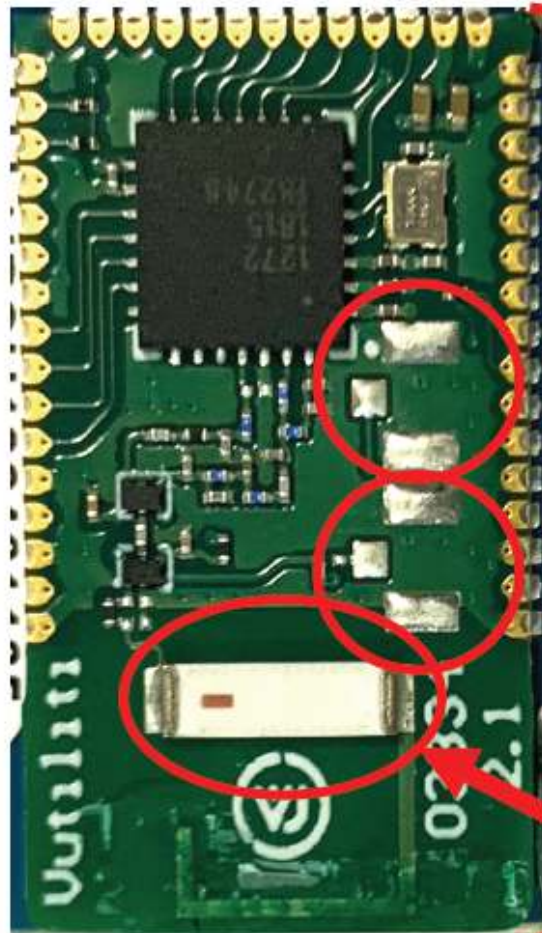
FCC Module Board: Top
