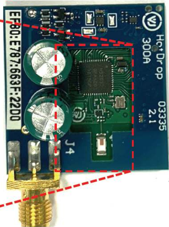
Host Carrier& Module: Bottom
