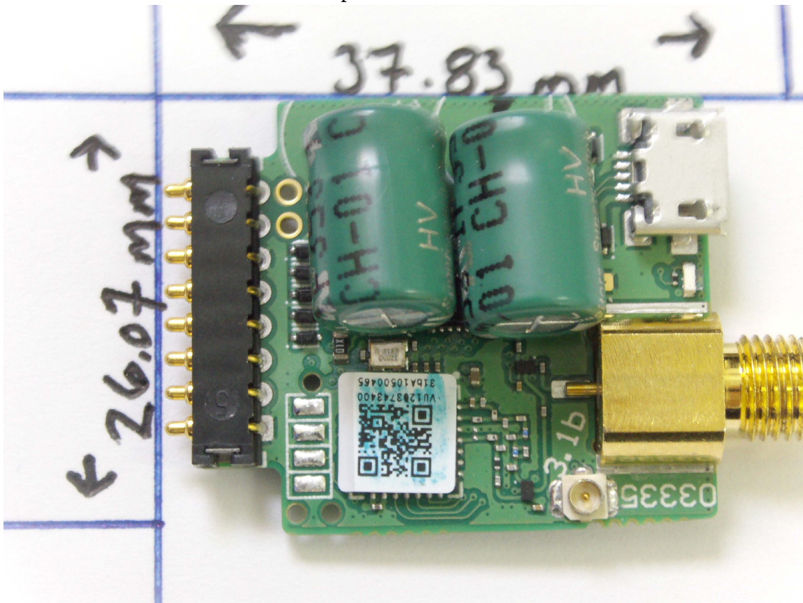
Top Side of module
