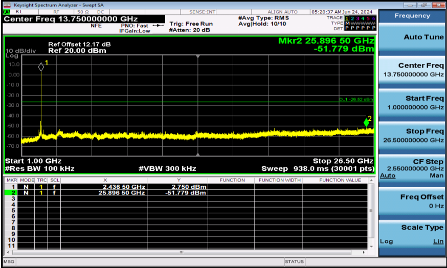
11B-Ant1-2437-1000~26500-PASS
