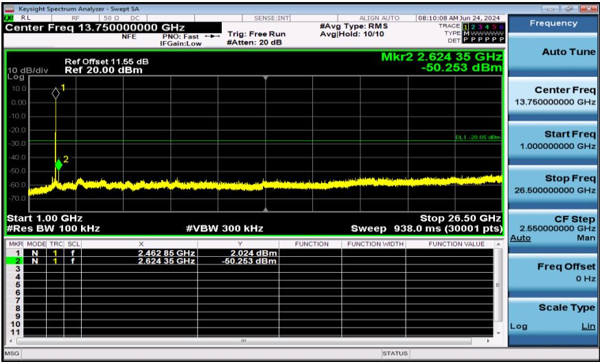
11B-Ant2-2462-1000~26500-PASS
