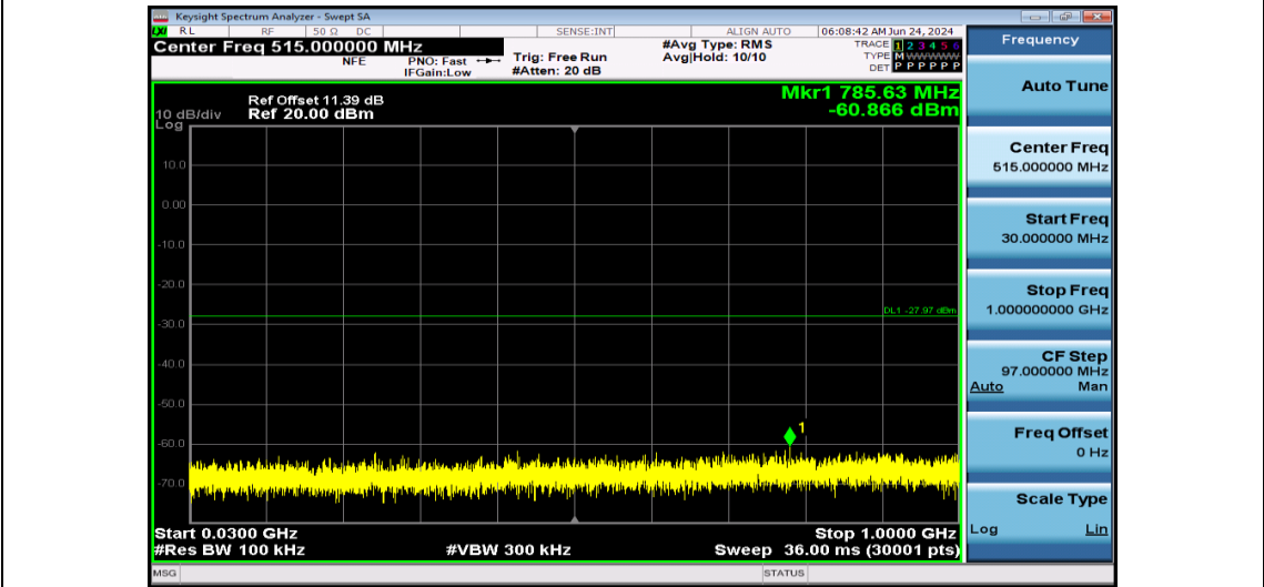
11B-Ant2-2412-30~1000-PASS
