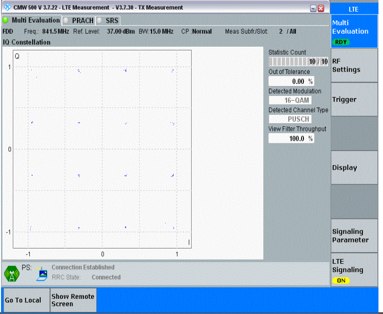
Band26(824-849)-15MHz-16QAM-26965-1RB#0-PASS
