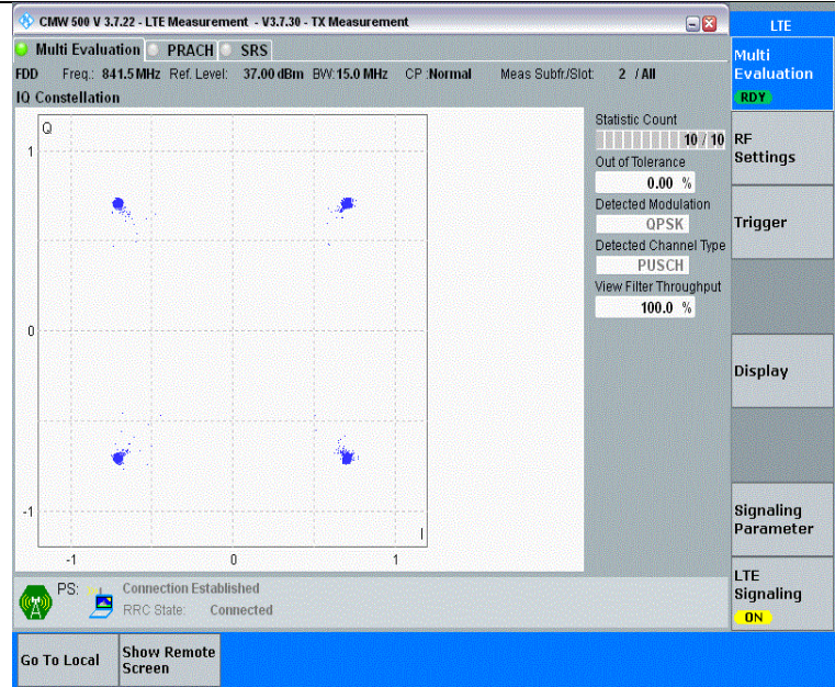
Band26(824-849)-15MHz-QPSK-26965-75RB#0-PASS
