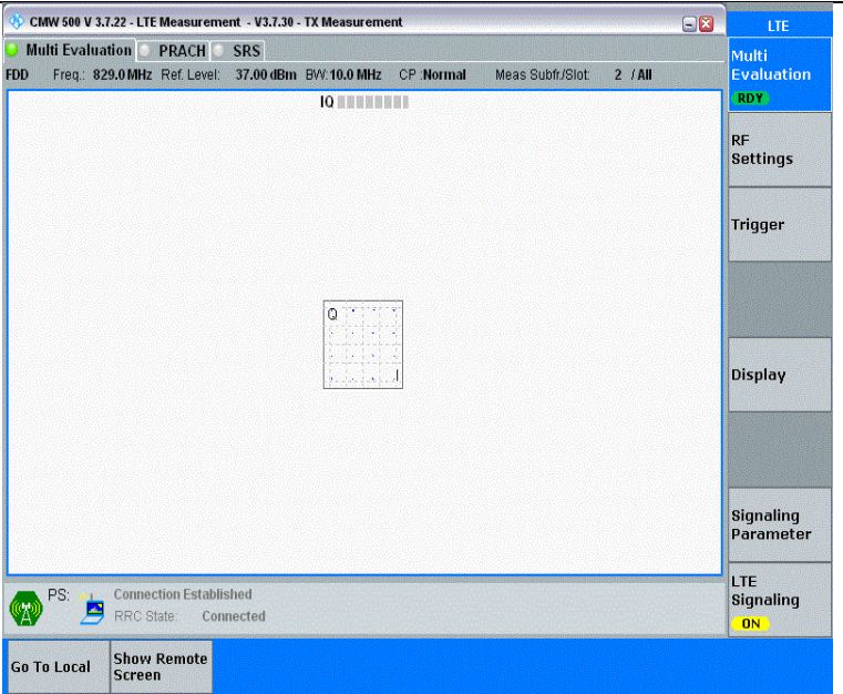
Band26(824-849)-10MHz-16QAM-26840-1RB#0-PASS
