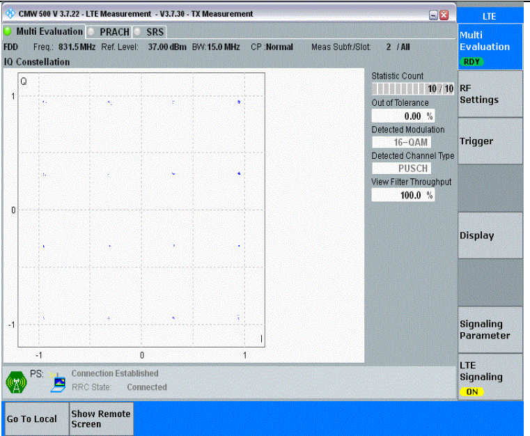
Band26(824-849)-15MHz-16QAM-26865-1RB#0-PASS
