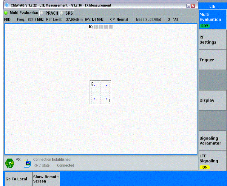
Band26(824-849)-1.4MHz-QPSK-26797-6RB#0-PASS
