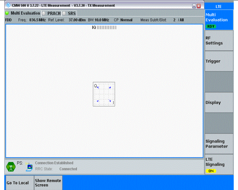
Band26(824-849)-10MHz-QPSK-26915-50RB#0-PASS
