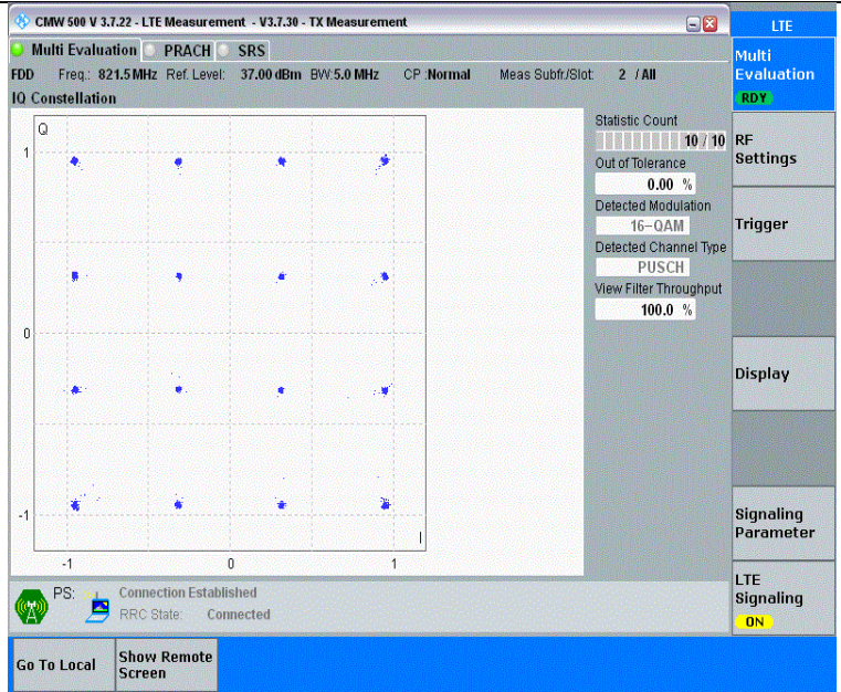
Band26(814-824)-5MHz-16QAM-26765-25RB#0-PASS
