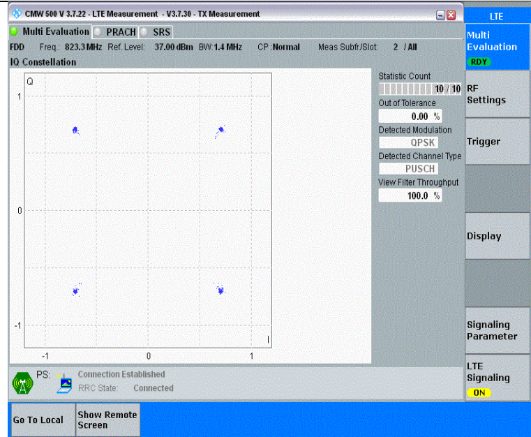
Band26(814-824)-1.4MHz-QPSK-26783-6RB#0-PASS
