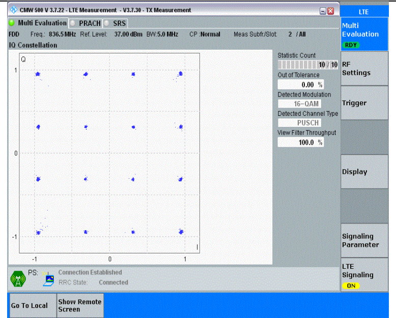
Band26(824-849)-5MHz-16QAM-26915-25RB#0-PASS
