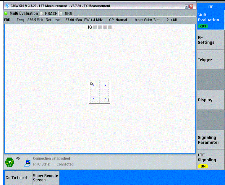
Band26(824-849)-1.4MHz-QPSK-26915-6RB#0-PASS
