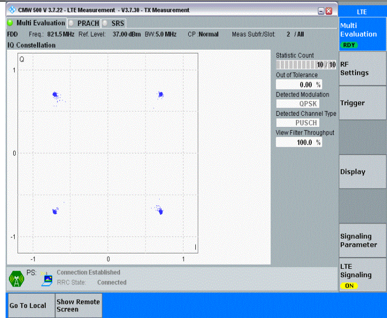
Band26(814-824)-5MHz-QPSK-26765-25RB#0-PASS
