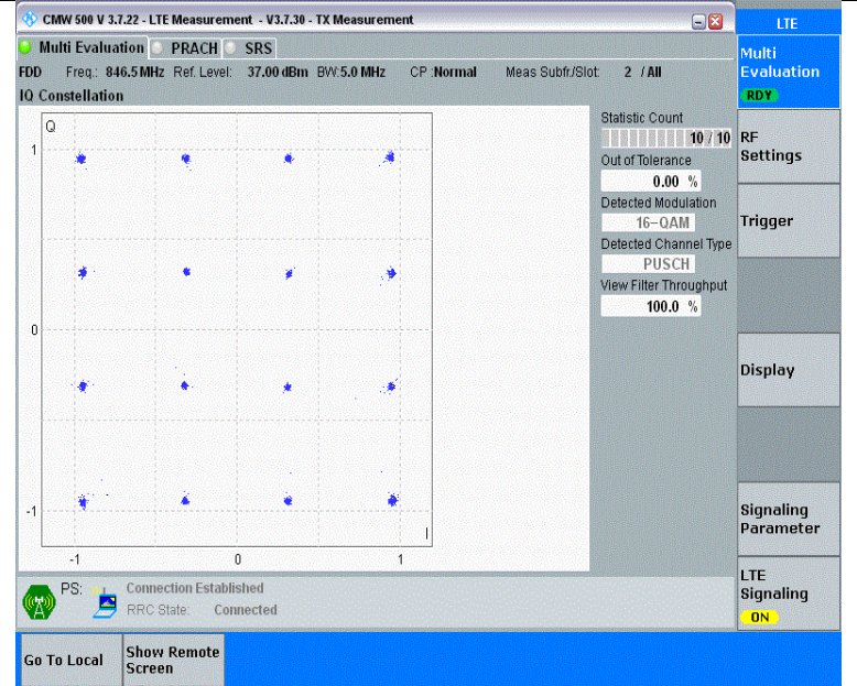
Band26(824-849)-5MHz-16QAM-27015-25RB#0-PASS
