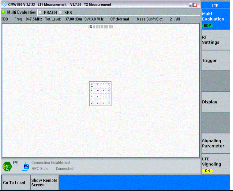
Band26(824-849)-3MHz-16QAM-27025-15RB#0-PASS
