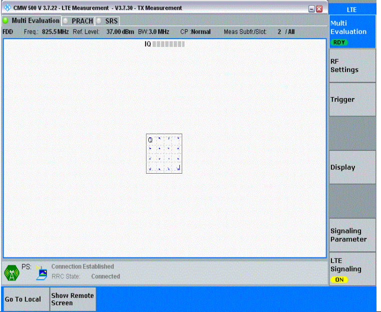
Band26(824-849)-3MHz-16QAM-26805-15RB#0-PASS
