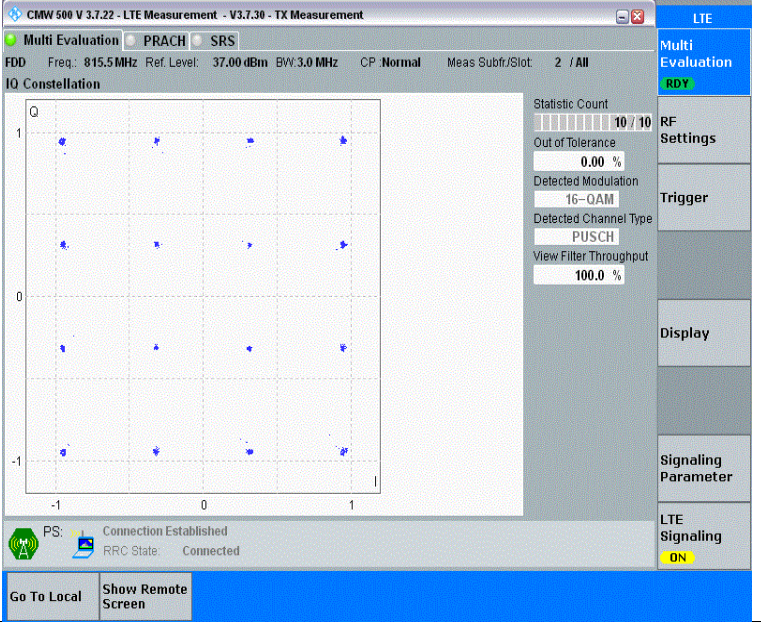
Band26(814-824)-3MHz-16QAM-26705-15RB#0-PASS
