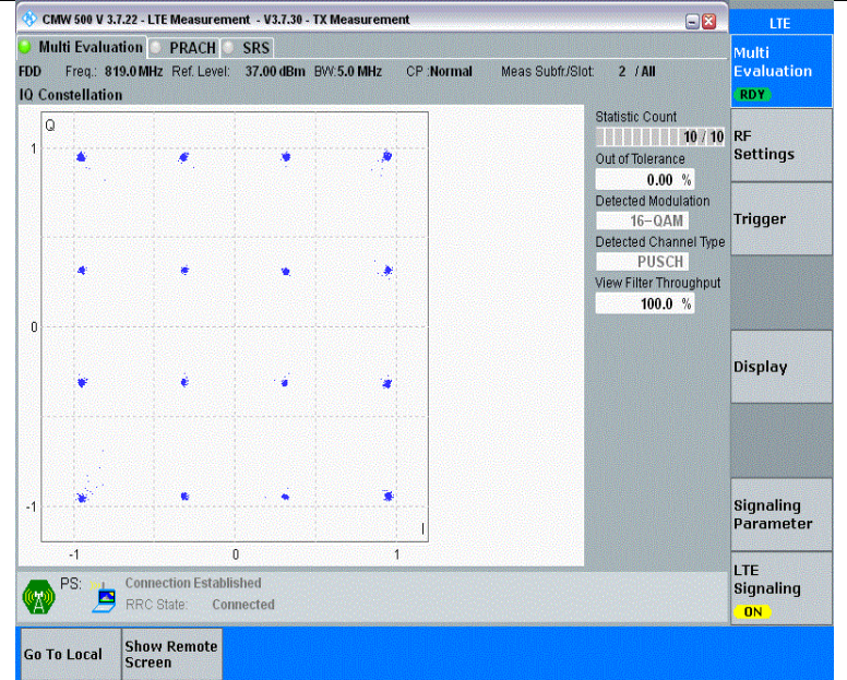
Band26(814-824)-5MHz-16QAM-26740-25RB#0-PASS
