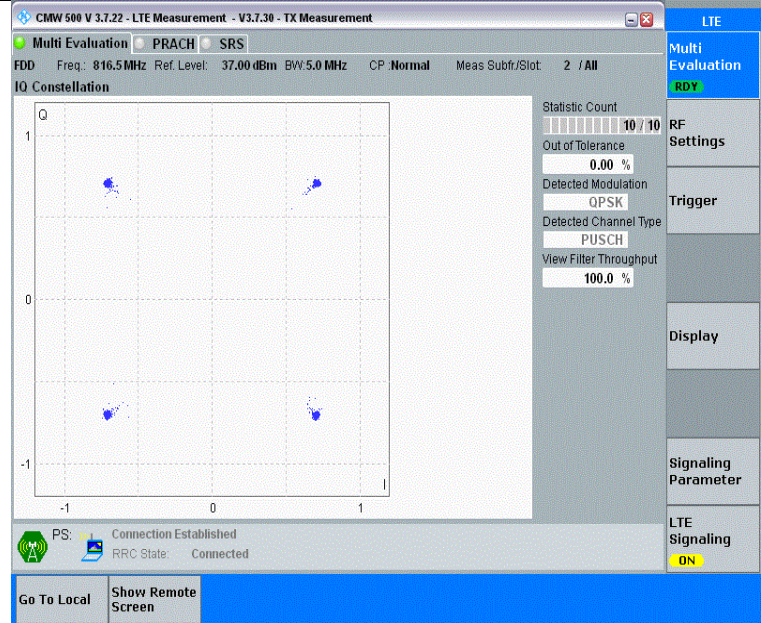
Band26(814-824)-5MHz-QPSK-26715-25RB#0-PASS
