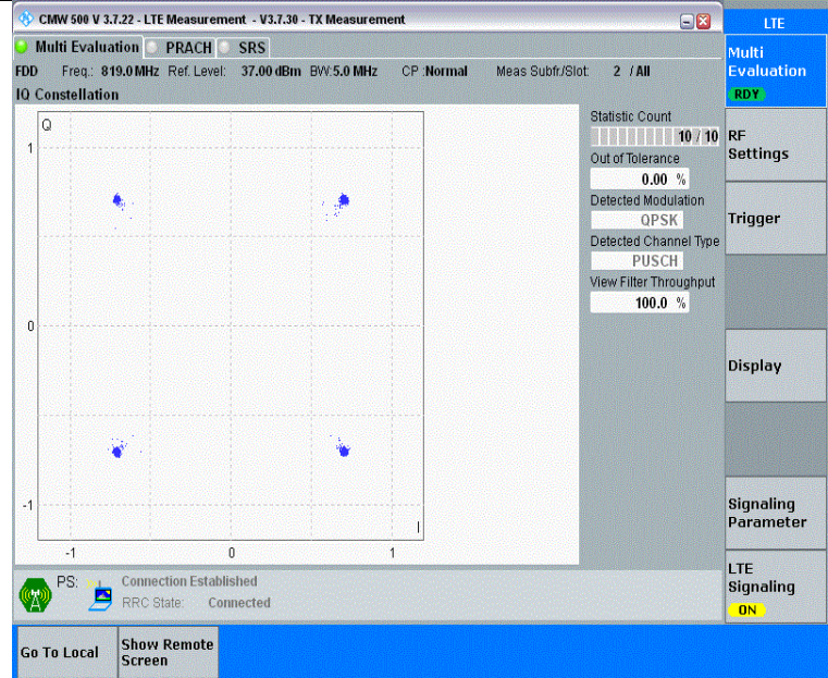
Band26(814-824)-5MHz-QPSK-26740-25RB#0-PASS
