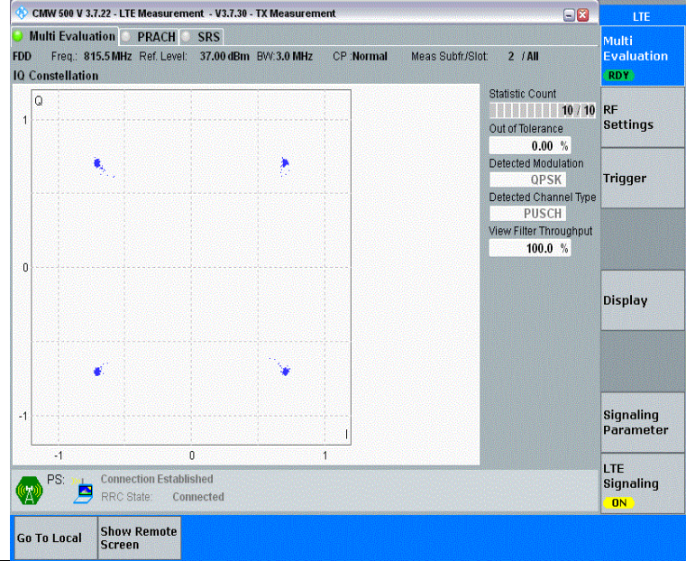
Band26(814-824)-3MHz-QPSK-26705-15RB#0-PASS
