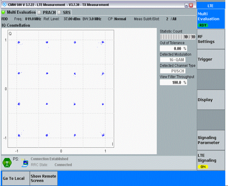
Band26(814-824)-3MHz-16QAM-26740-15RB#0-PASS
