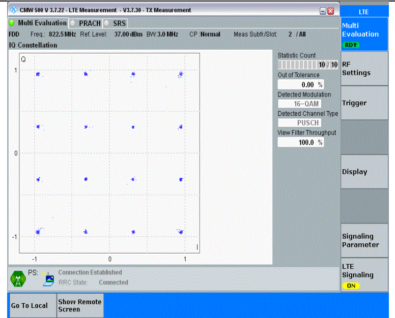
Band26(814-824)-3MHz-16QAM-26775-15RB#0-PASS
