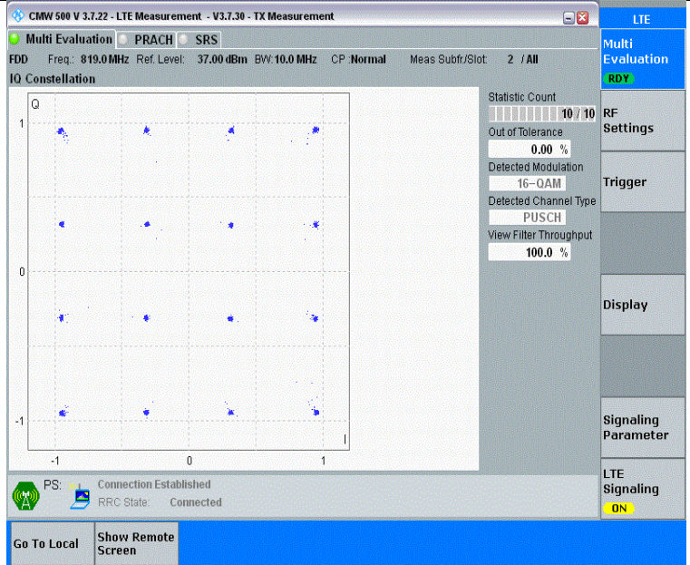
Band26(814-824)-10MHz-16QAM-26740-27RB#0-PASS
