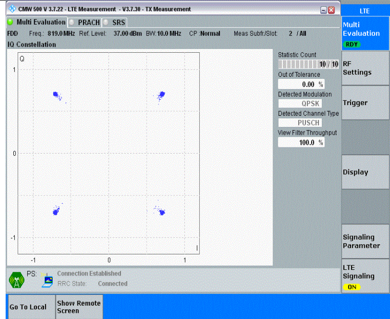
Band26(814-824)-10MHz-QPSK-26740-50RB#0-PASS
