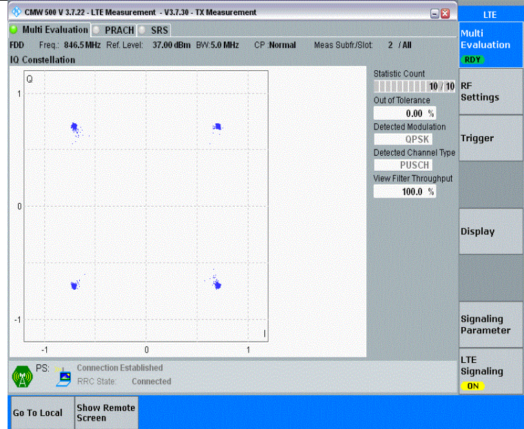
Band26(824-849)-5MHz-QPSK-27015-25RB#0-PASS
