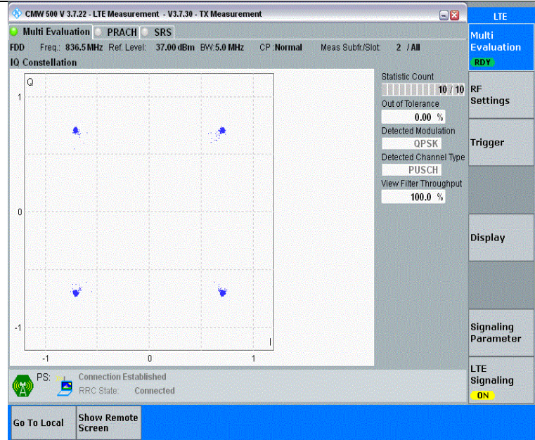
Band26(824-849)-5MHz-QPSK-26915-25RB#0-PASS
