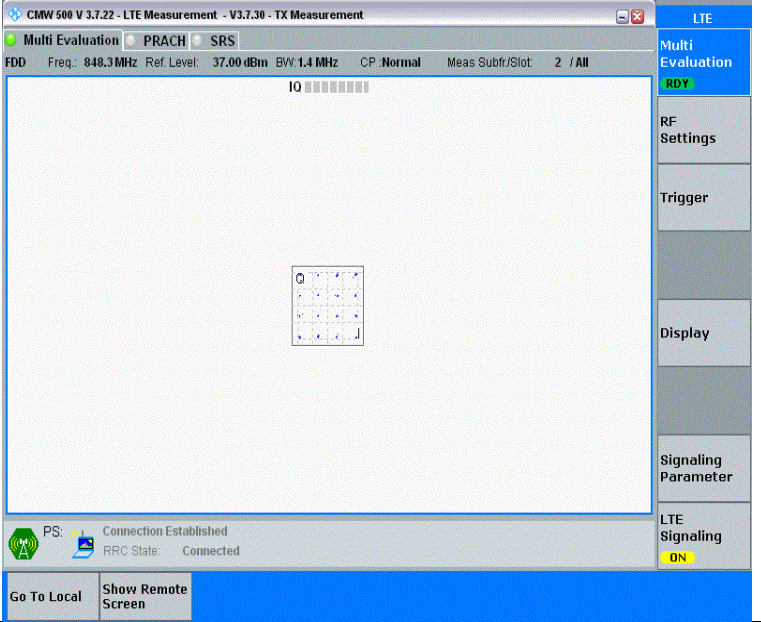
Band26(824-849)-1.4MHz-16QAM-27033-6RB#0-PASS
