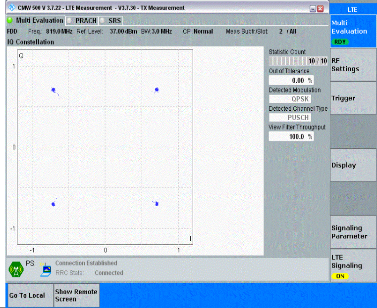
Band26(814-824)-3MHz-QPSK-26740-15RB#0-PASS
