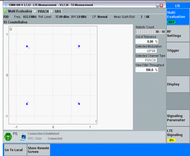
Band26(814-824)-3MHz-QPSK-26775-15RB#0-PASS
