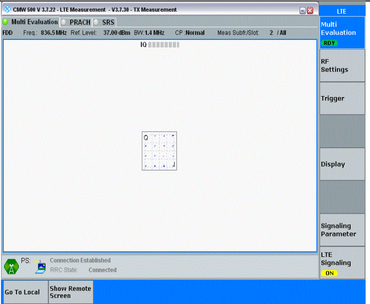
Band26(824-849)-1.4MHz-16QAM-26915-6RB#0-PASS
