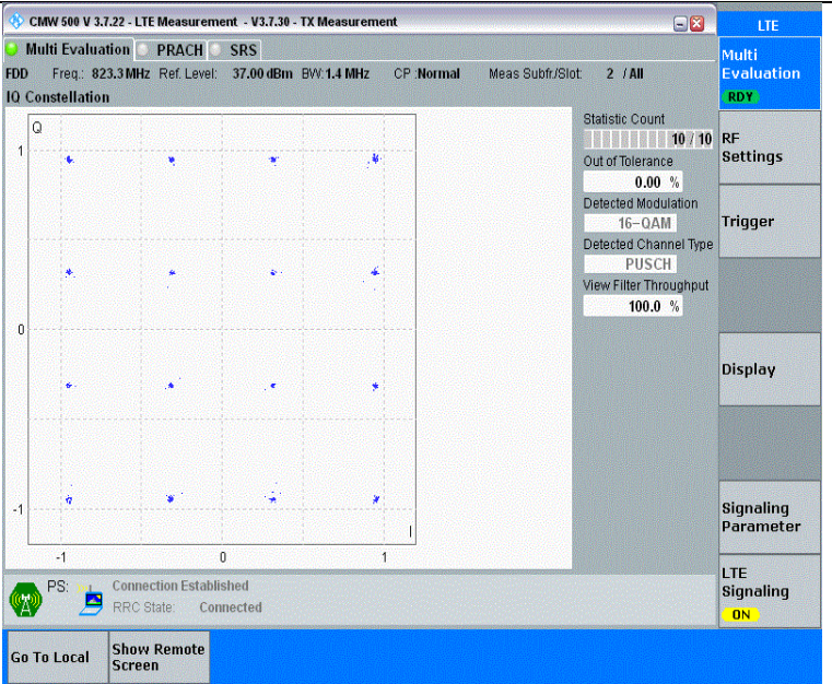
Band26(814-824)-1.4MHz-16QAM-26783-6RB#0-PASS
