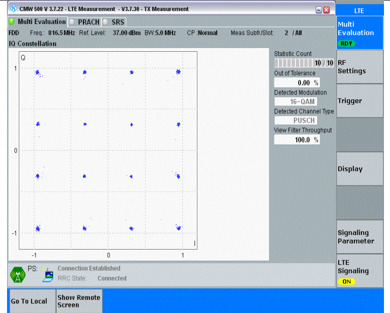
Band26(814-824)-5MHz-16QAM-26715-25RB#0-PASS
