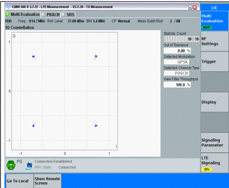
Band26(814-824)-1.4MHz-QPSK-26697-6RB#0-PASS
