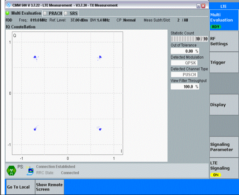
Band26(814-824)-1.4MHz-QPSK-26740-6RB#0-PASS
