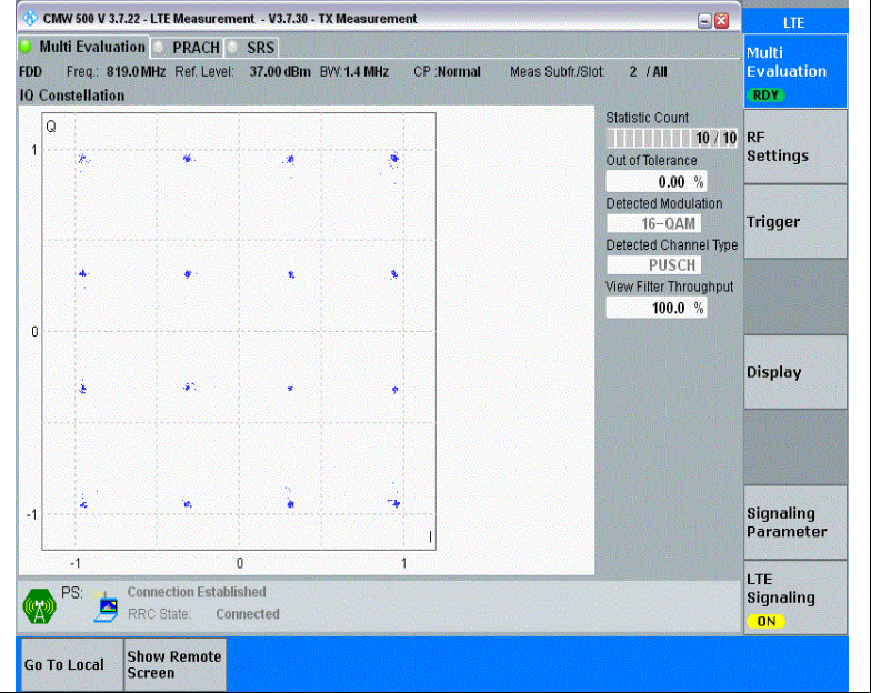
Band26(814-824)-1.4MHz-16QAM-26740-6RB#0-PASS
