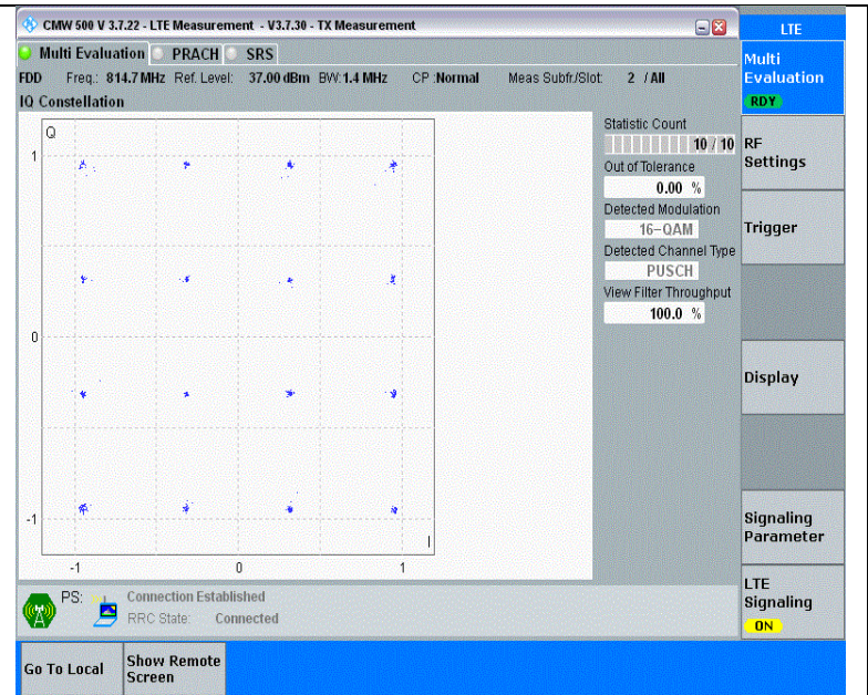
Band26(814-824)-1.4MHz-16QAM-26697-6RB#0-PASS
