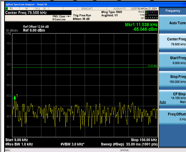
Band26_10MHz_QPSK_26840_50RB#0_0.009~0.15_0.009~0.15
