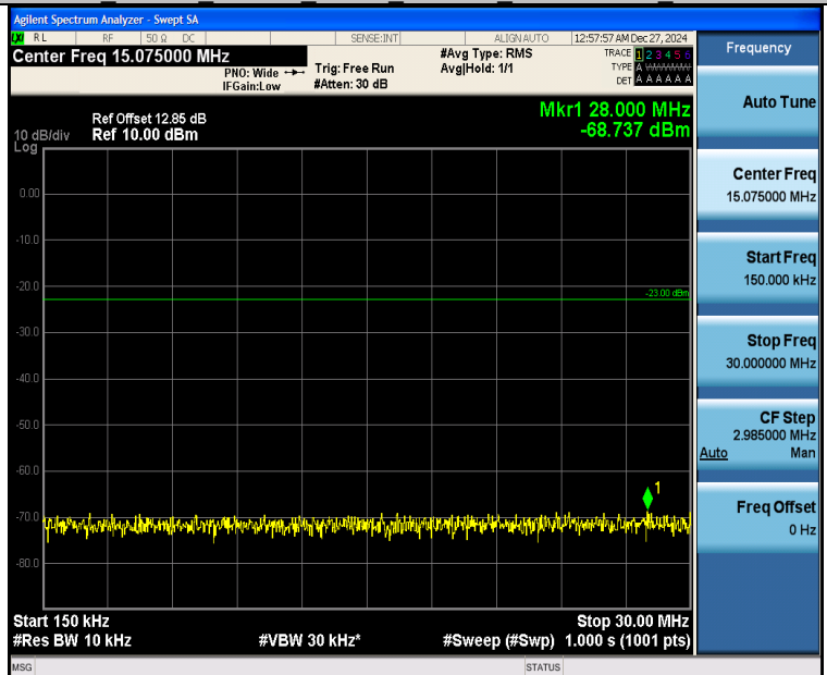
Band26_10MHz_QPSK_26840_50RB#0_0.15~30_0.15~30
