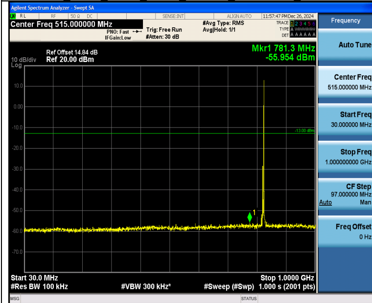
Band26_5MHz_QPSK_26815_1RB#24_30~1000_30~1000
