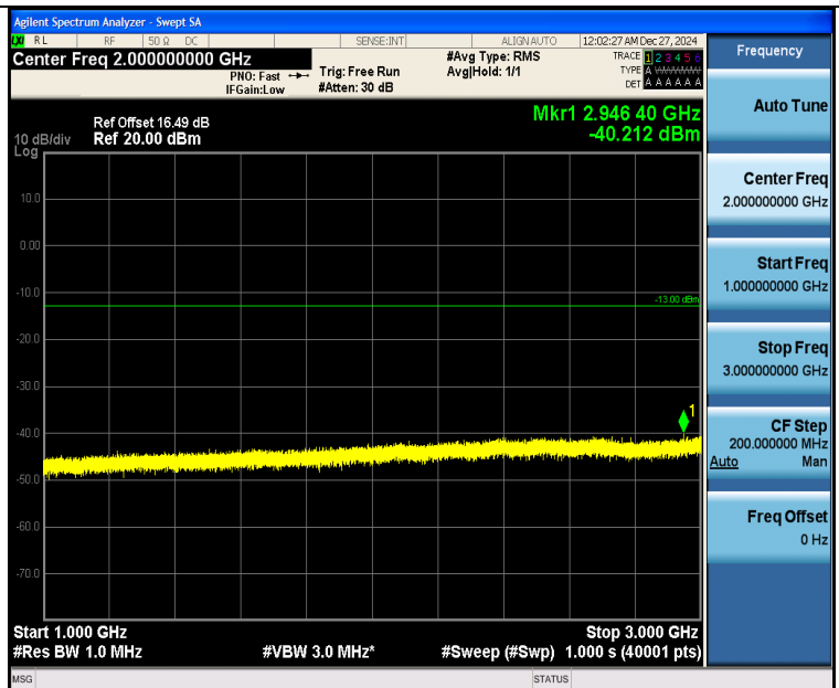
Band26_5MHz_QPSK_26915_1RB#0_1000~3000_1000~3000
