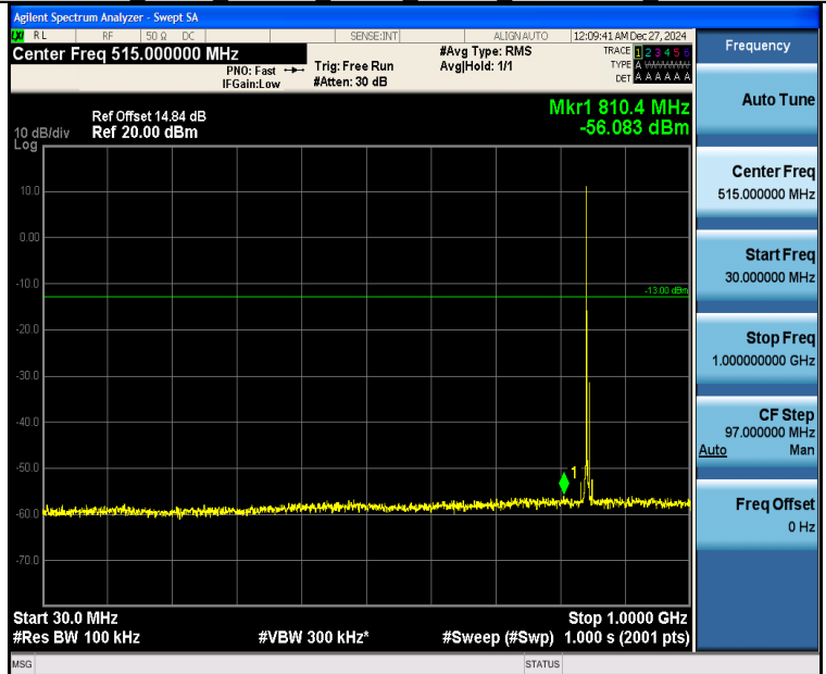
Band26_5MHz_16QAM_27015_1RB#0_30~1000_30~1000
