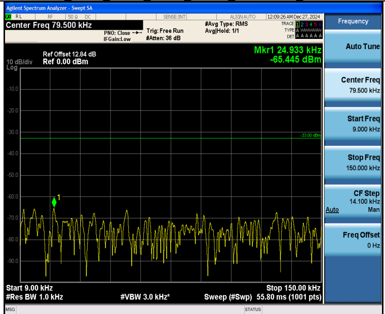
Band26_5MHz_16QAM_27015_1RB#0_0.009~0.15_0.009~0.15
