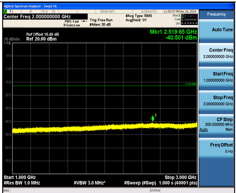
Band26_5MHz_QPSK_26815_1RB#0_1000~3000_1000~3000
