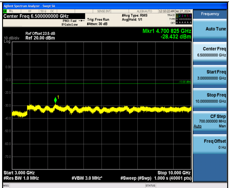
Band26 5MHz 16QAM 27015 1RB#0 3000~10000 3000~10000
