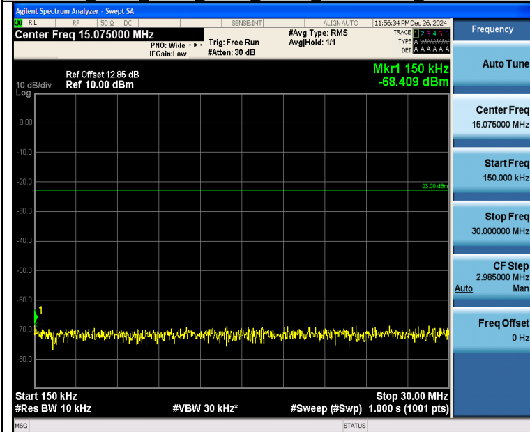
Band26_5MHz_16QAM_26815_1RB#0_0.15~30_0.15~30
