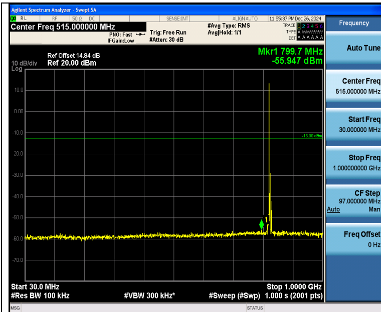
Band26_5MHz_QPSK_26815_1RB#0_30~1000_30~1000
