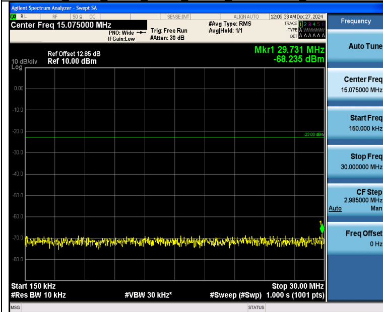
Band26_5MHz_16QAM_27015_1RB#0_0.15~30_0.15~30
