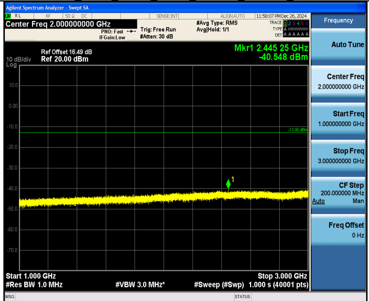
Band26_5MHz_QPSK_26815_1RB#24_1000~3000_1000~3000
