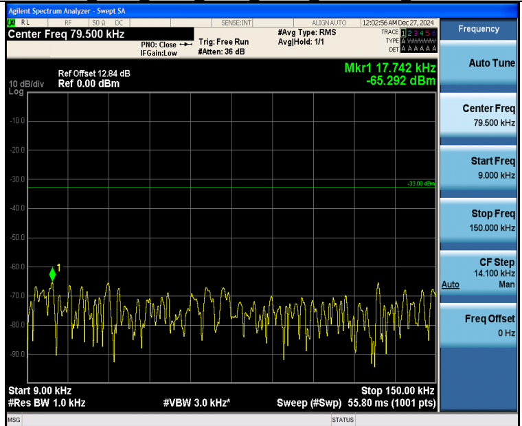
Band26_5MHz_16QAM_26915_1RB#0_0.009~0.15_0.009~0.15
