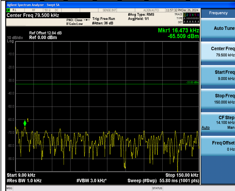
Band26 5MHz QPSK 26815 1RB#24 0.009~0.15 0.009~0.15
