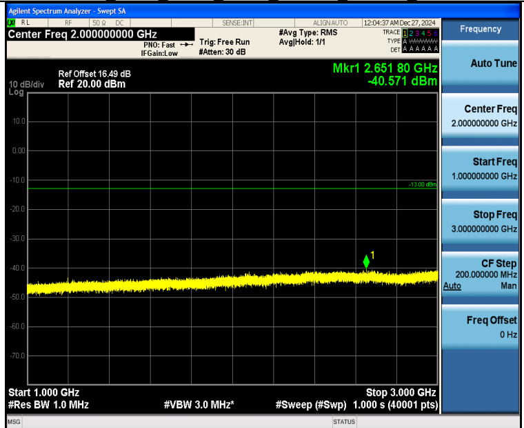
Band26_5MHz_QPSK_26915_1RB#24_1000~3000_1000~3000
