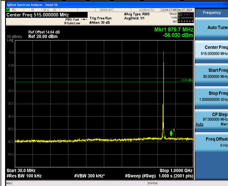
Band26_5MHz_QPSK_26915_1RB#24_30~1000_30~1000
