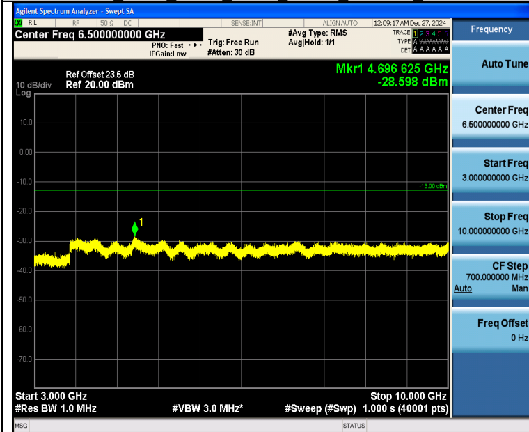
Band26_5MHz_QPSK_27015_1RB#0_3000~10000_3000~10000
