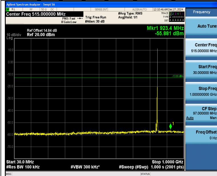
Band26_5MHz_QPSK_27015_1RB#24_30~1000_30~1000
