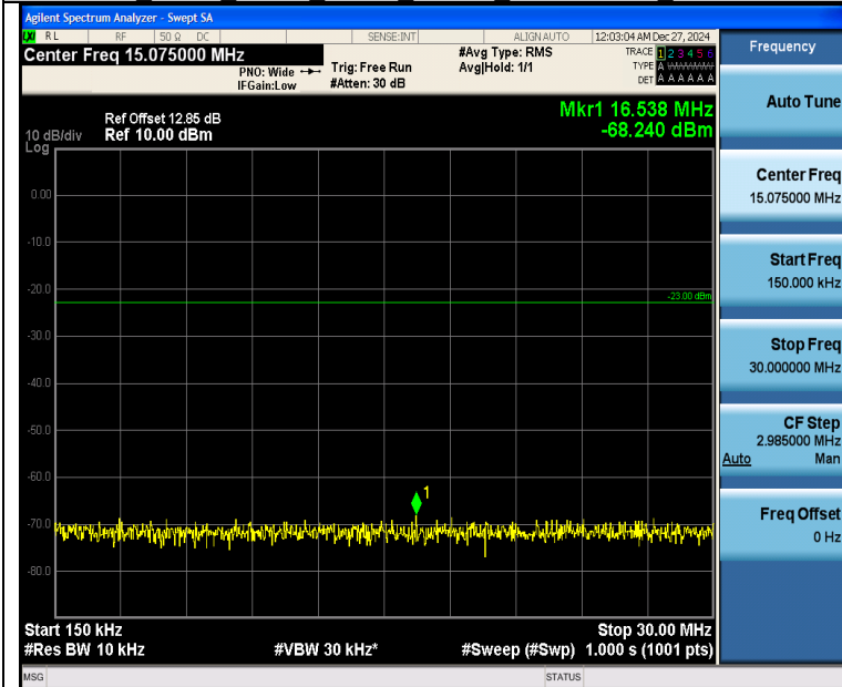
Band26_5MHz_16QAM_26915_1RB#0_0.15~30_0.15~30
