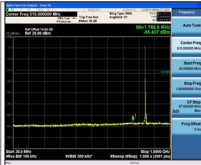
Band26_5MHz_QPSK_27015_1RB#0_30~1000_30~1000
