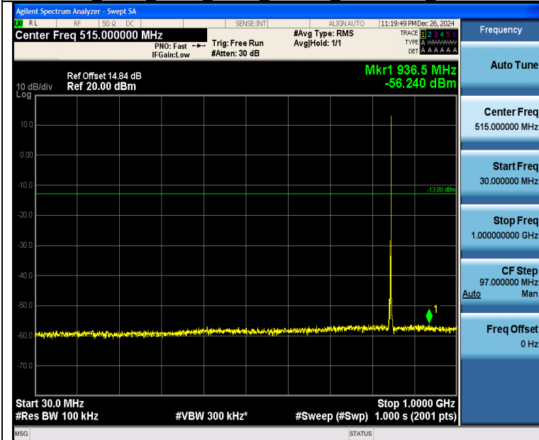
Band26_3MHz_QPSK_27025_1RB#14_30~1000_30~1000
