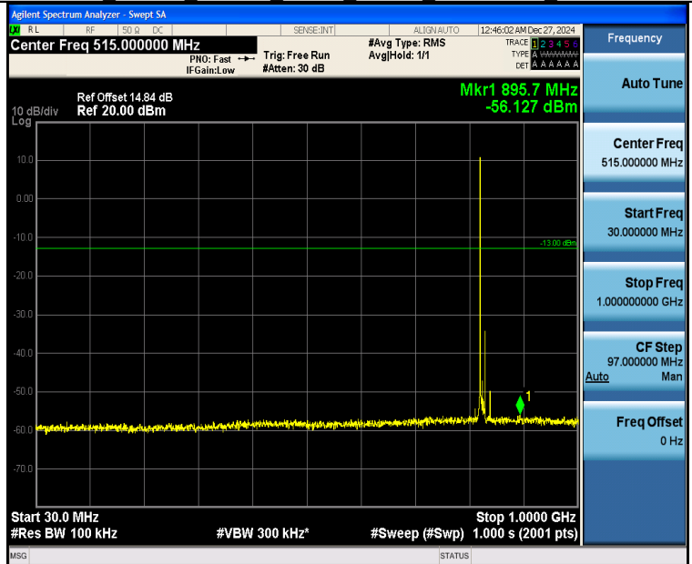
Band26 10MHz 16QAM 26840 1RB#0 30~1000 30~1000
