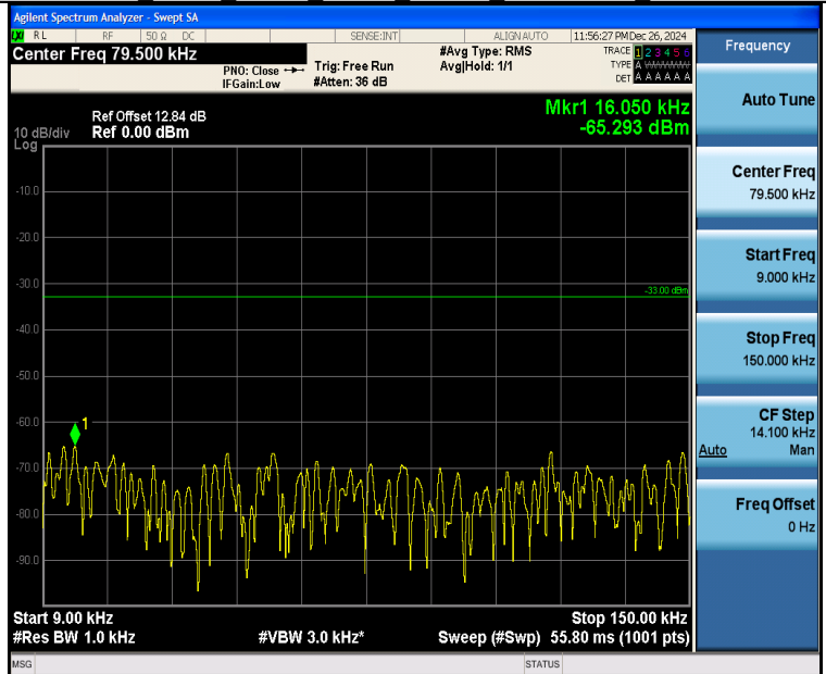
Band26_5MHz_16QAM_26815_1RB#0_0.009~0.15_0.009~0.15
