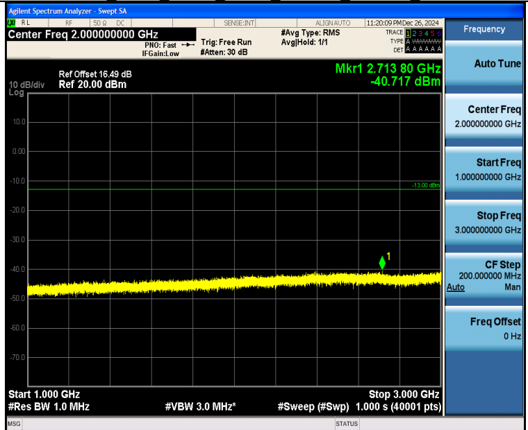
Band26_3MHz_QPSK_27025_1RB#14_1000~3000_1000~3000
