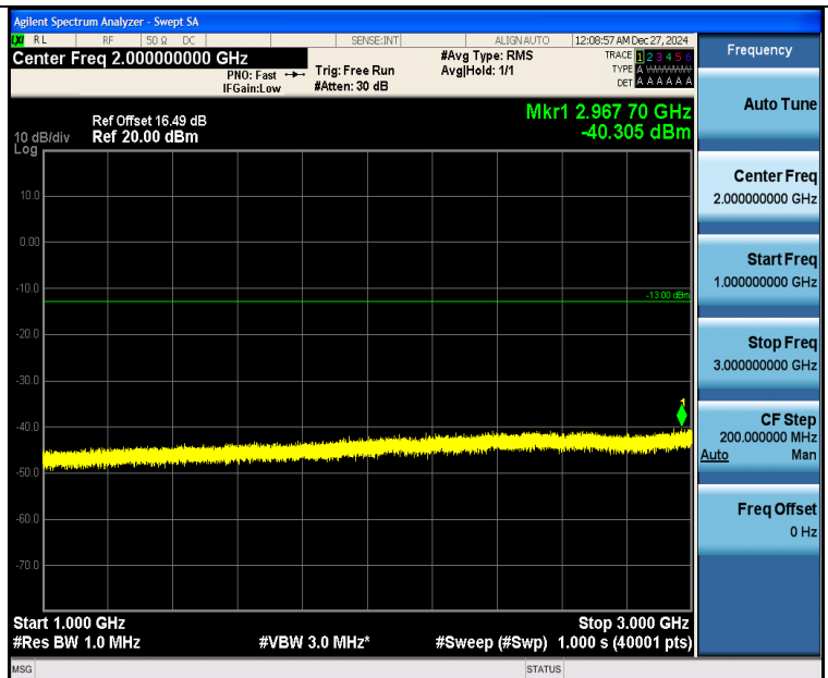
Band26_5MHz_QPSK_27015_1RB#0_1000~3000_1000~3000
