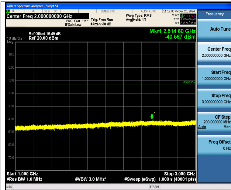
Band26 3MHz 16QAM 27025 1RB#0 1000~3000 1000~3000
