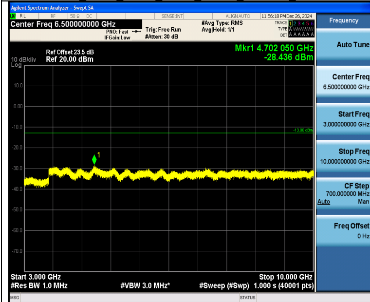
Band26_5MHz_QPSK_26815_1RB#0_3000~10000_3000~10000
