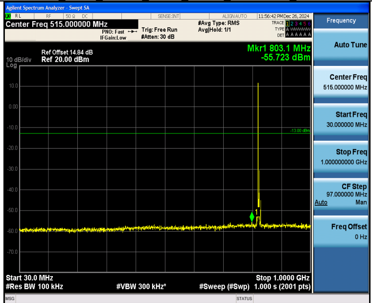
Band26_5MHz_16QAM_26815_1RB#0_30~1000_30~1000
