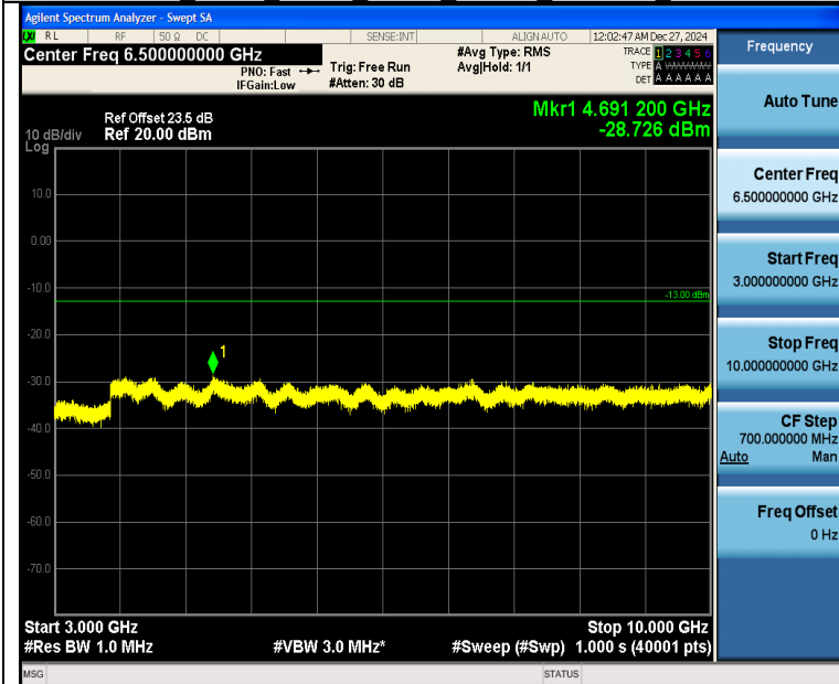
Band26_5MHz_QPSK_26915_1RB#0_3000~10000_3000~10000
