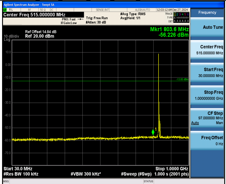
Band26_5MHz_16QAM_26915_1RB#0_30~1000_30~1000
