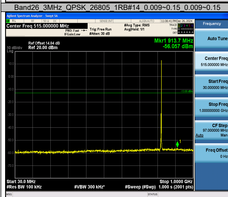
Band26_3MHz_QPSK_26805_1RB#14_30~1000_30~1000
