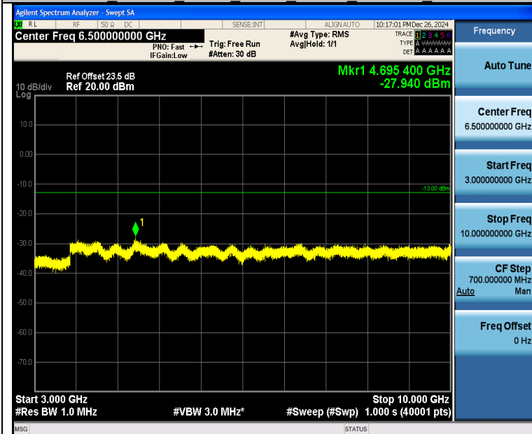
Band26 1.4MHz QPSK 26915 1RB#0 3000~10000 3000~10000
