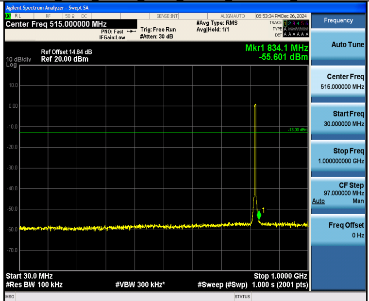
Band26_5MHz_16QAM_26765_25RB#0_30~1000_30~1000
