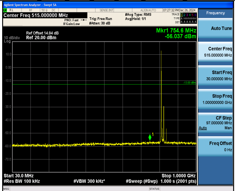
Band26 15MHz_QPSK_26765_1RB#0_30~1000_30~1000
