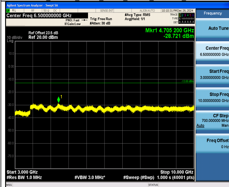
Band26 1.4MHz QPSK 26797 1RB#0 3000~10000 3000~10000
