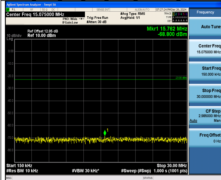
Band26 15MHz_QPSK_26765_1RB#0_0.15~30_0.15~30
