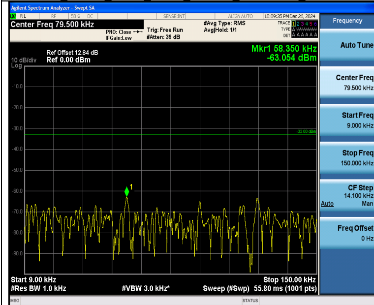
Band26 1.4MHz_QPSK_26797_1RB#0_0.009~0.15_0.009~0.15
