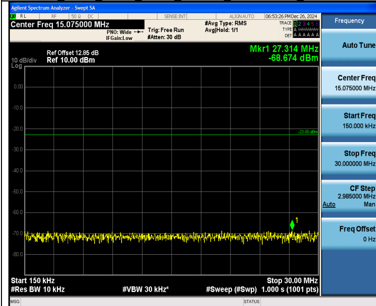
Band26_5MHz_16QAM_26765_25RB#0_0.15~30_0.15~30
