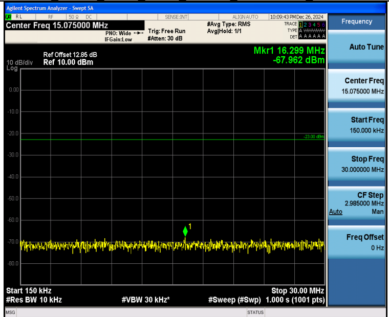
Band26 1.4MHz_QPSK_26797_1RB#0_0.15~30_0.15~30
