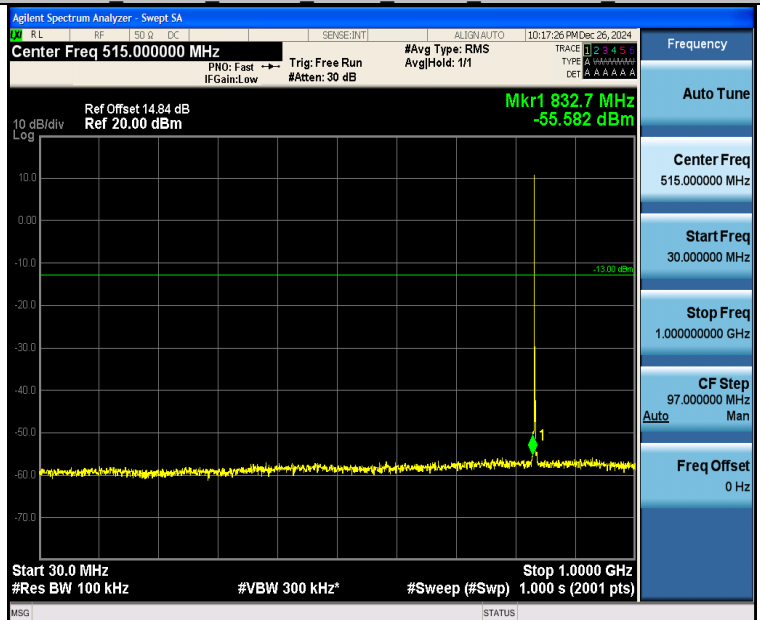
Band26 1.4MHz 16QAM 26915 1RB#0 30~1000 30~1000
