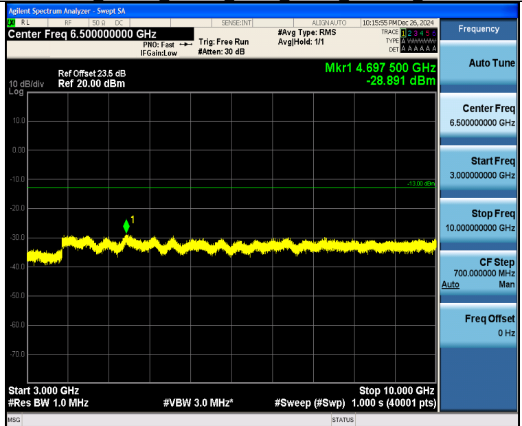
Band26 1.4MHz 16QAM 26797 6RB#0 3000~10000 3000~10000
