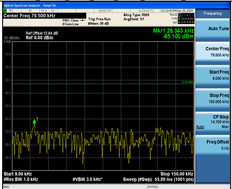
Band26 1.4MHz 16QAM 26797 1RB#0 0.009~0.15 0.009~0.15
