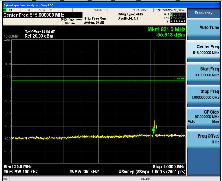
Band26 1.4MHz 16QAM 26797 1RB#0 30~1000 30~1000
