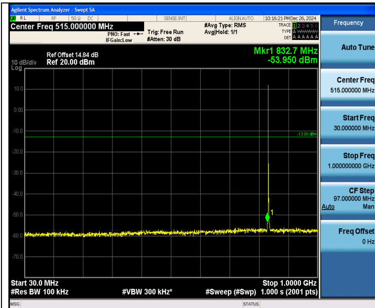
Band26 1.4MHz QPSK 26915 1RB#0 30~1000 30~1000
