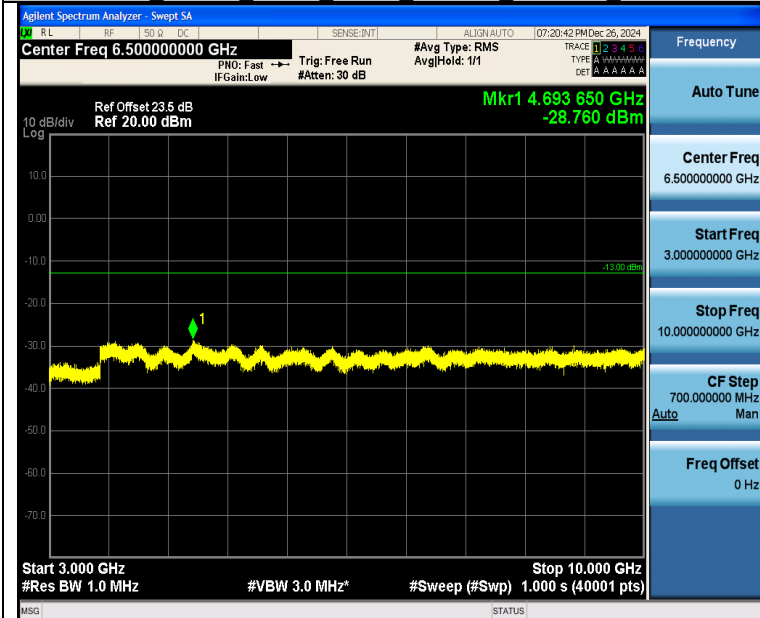
Band26 10MHz QPSK 26740 50RB#0 3000~10000 3000~10000
