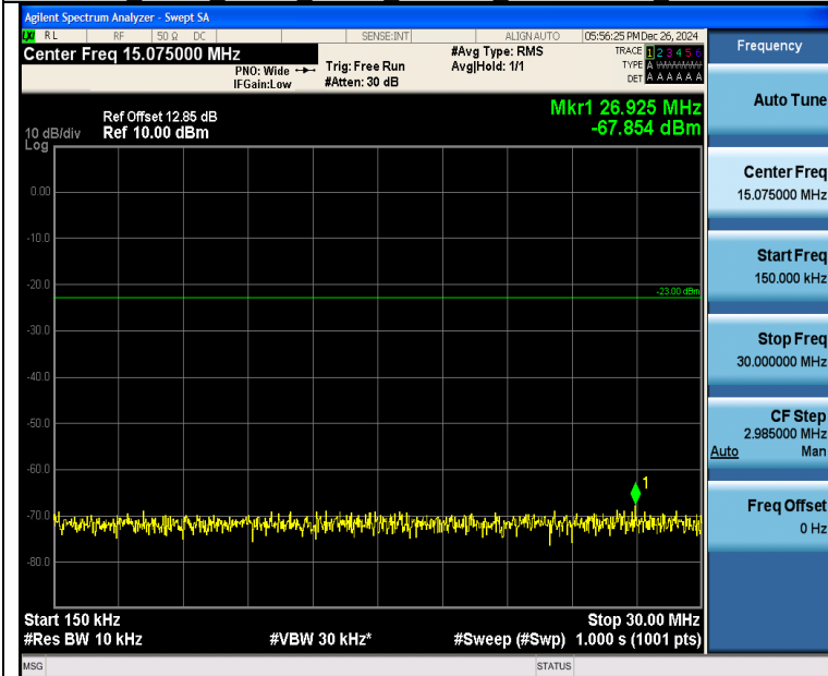
Band26_3MHz_16QAM_26740_15RB#0_0.15~30_0.15~30
