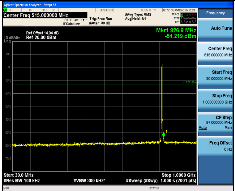
Band26_3MHz_16QAM_26740_15RB#0_30~1000_30~1000
