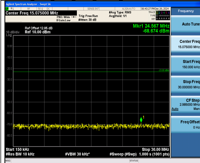
Band26_5MHz_16QAM_26715_25RB#0_0.15~30_0.15~30
