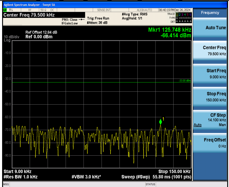
Band26 5MHz 16QAM 26715 25RB#0 0.009~0.15 0.009~0.15
