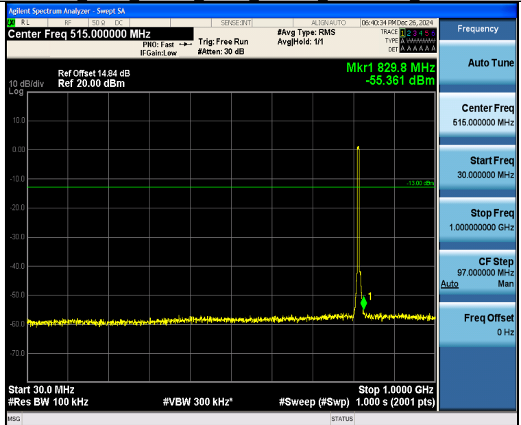
Band26_5MHz_16QAM_26715_25RB#0_30~1000_30~1000
