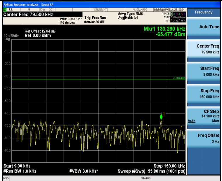
Band26 3MHz 16QAM 26740 15RB#0 0.009~0.15 0.009~0.15
