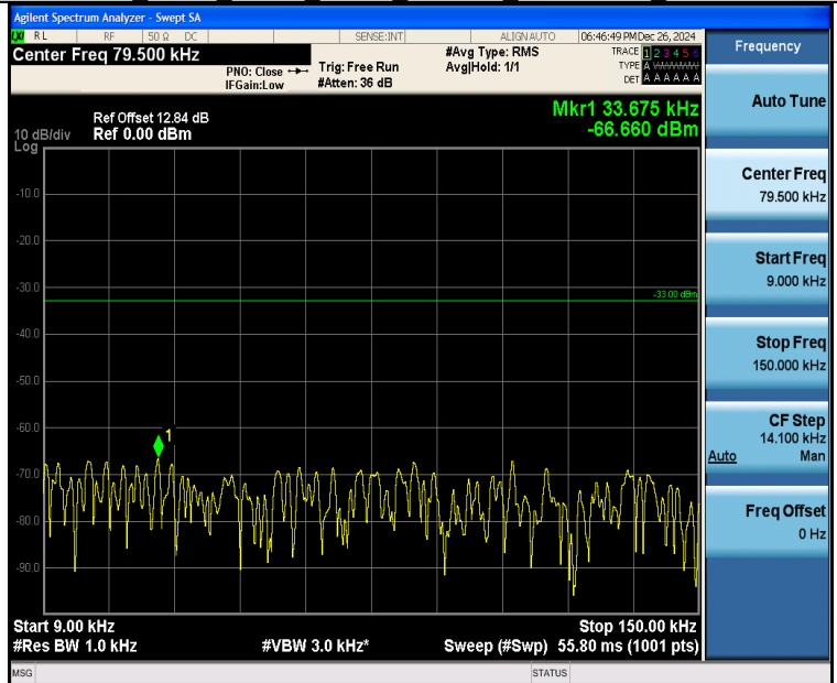
Band26 5MHz 16QAM 26740 25RB#0 0.009~0.15 0.009~0.15
