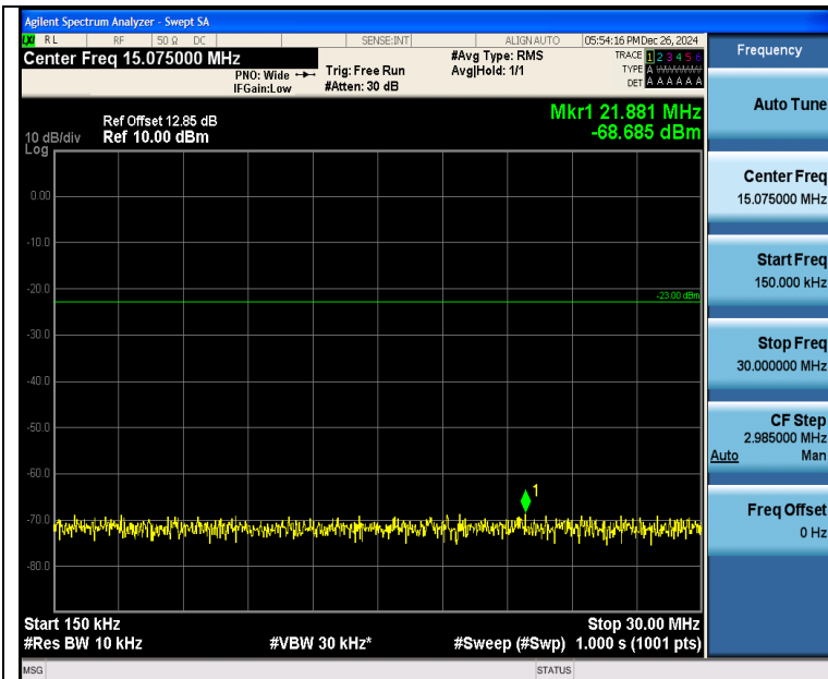
Band26 3MHz 16QAM 26740 1RB#14 0.15~30 0.15~30
