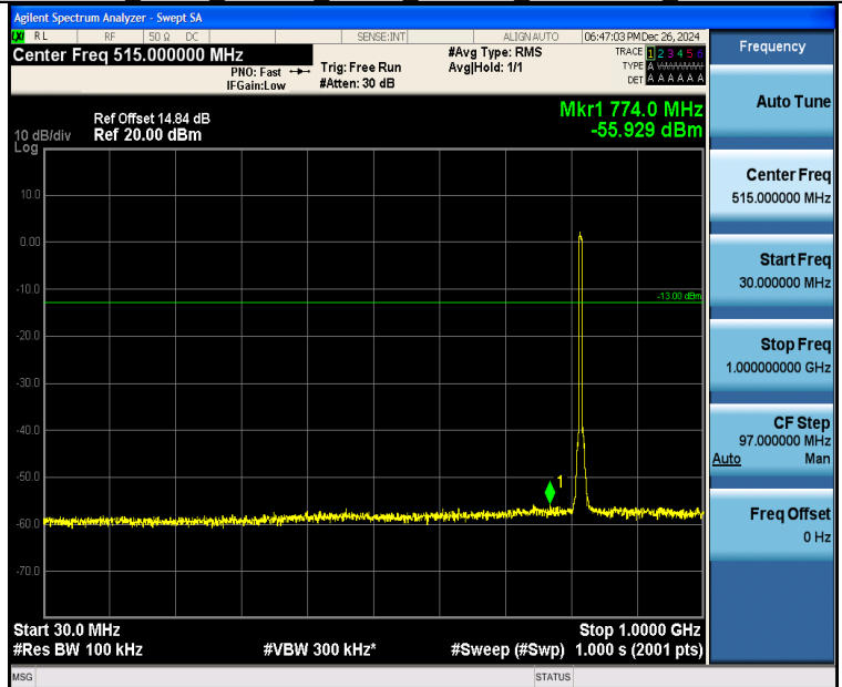
Band26_5MHz_16QAM_26740_25RB#0_30~1000_30~1000
