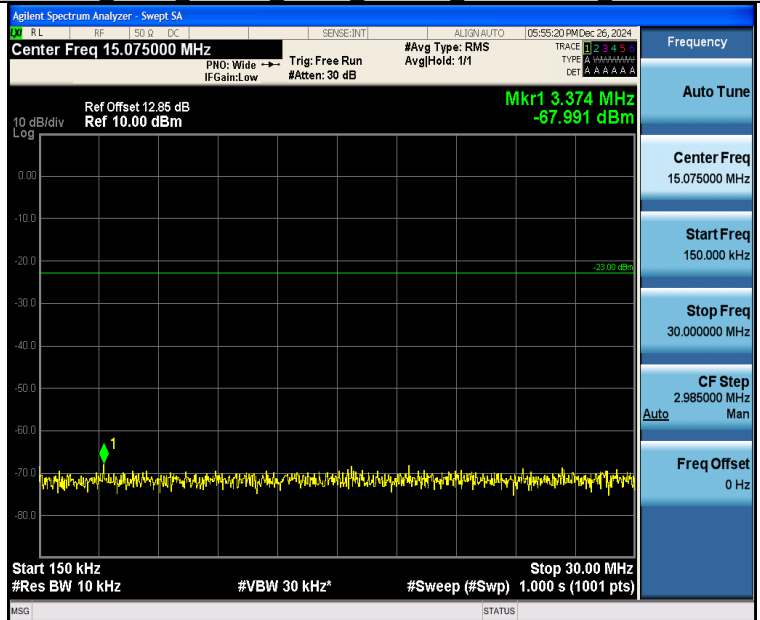
Band26 3MHz_QPSK 26740 15RB#0 0.15~30 0.15~30
