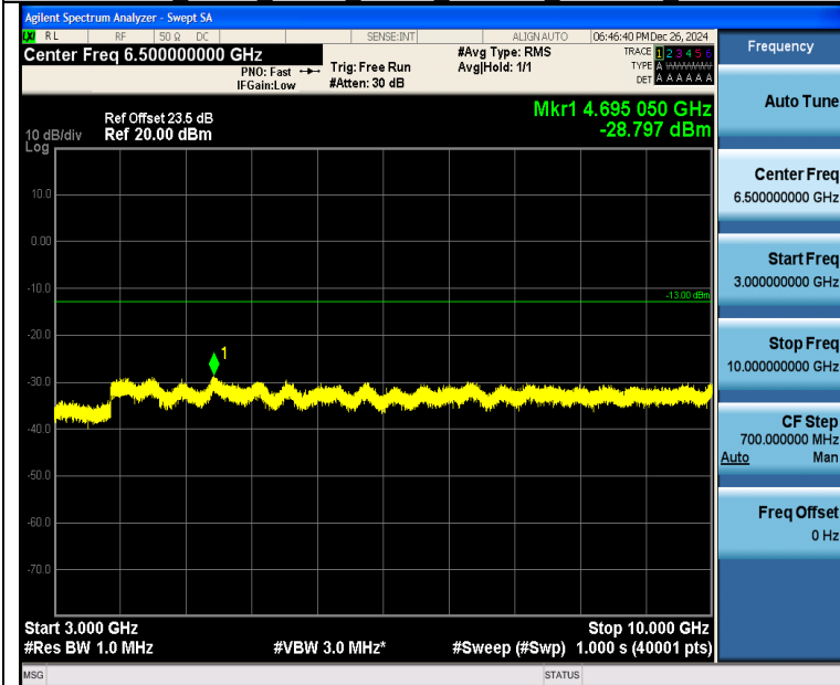
Band26 5MHz QPSK 26740 25RB#0 3000~10000 3000~10000
