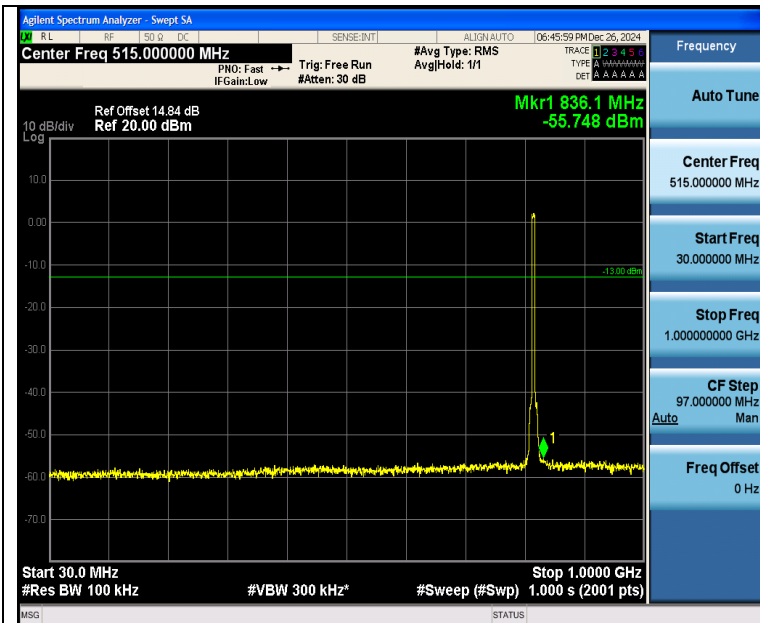
Band26 5MHz QPSK 26740 25RB#0 30~1000 30~1000
