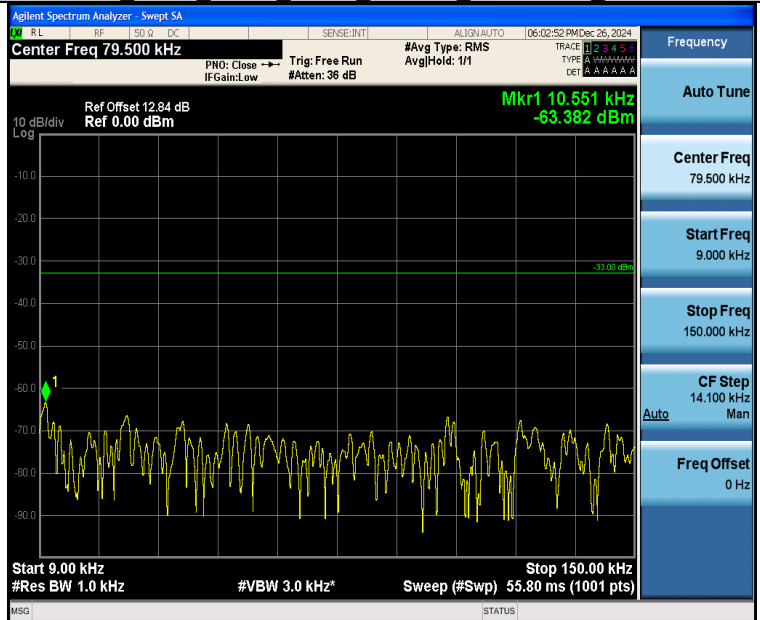
Band26 3MHz 16QAM 26775 15RB#0 0.009~0.15 0.009~0.15
