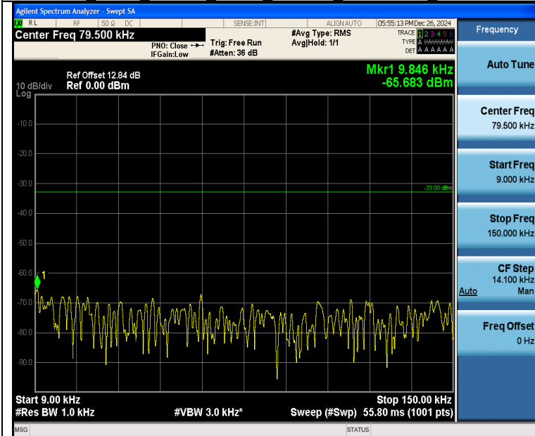
Band26 3MHz_QPSK 26740 15RB#0 0.009~0.15 0.009~0.15
