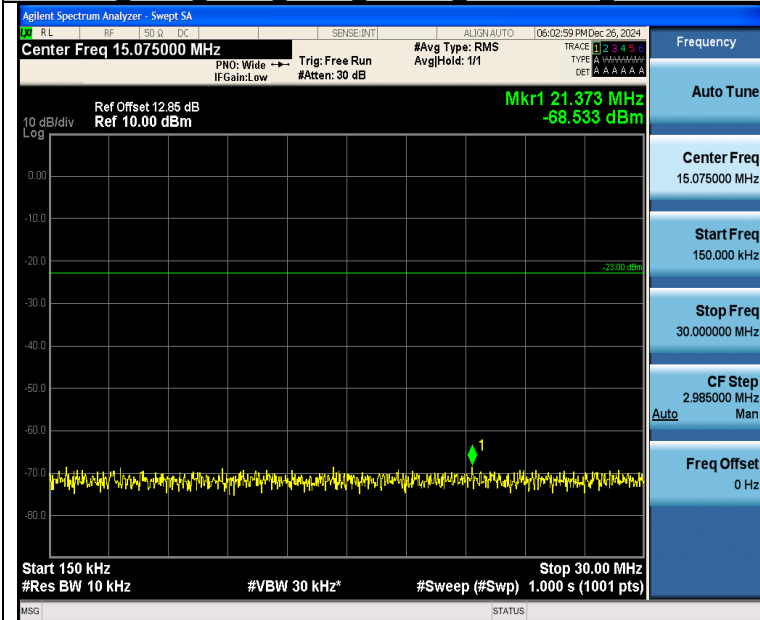
Band26_3MHz_16QAM_26775_15RB#0_0.15~30_0.15~30
