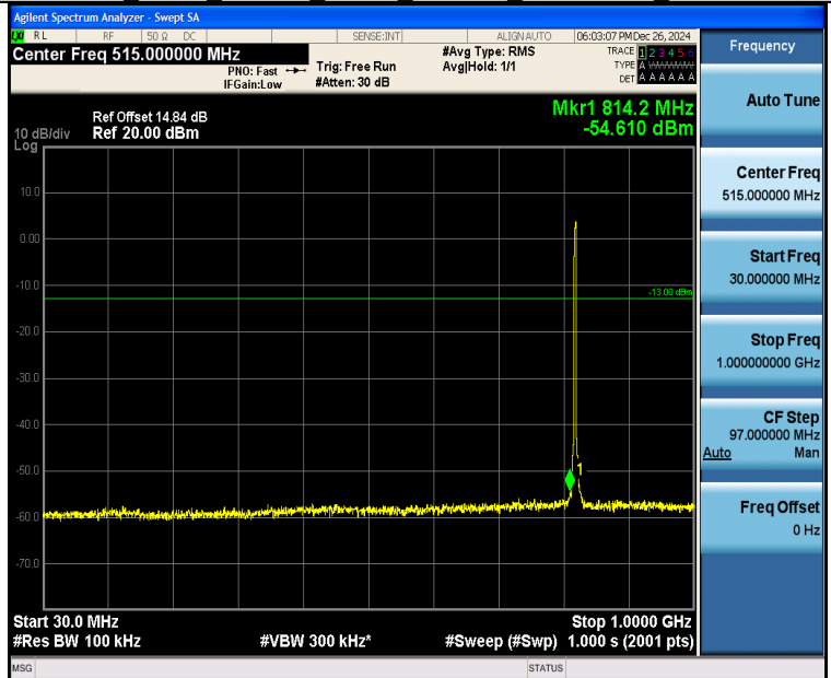
Band26_3MHz_16QAM_26775_15RB#0_30~1000_30~1000
