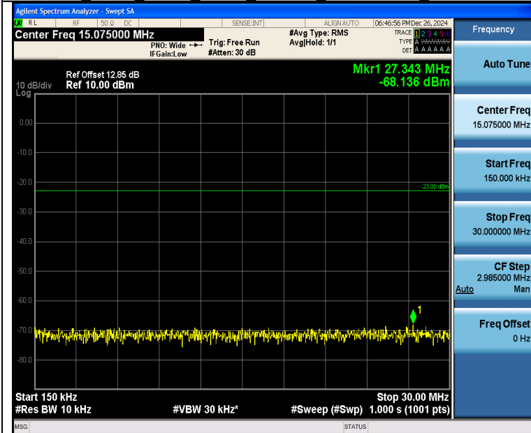
Band26_5MHz_16QAM_26740_25RB#0_0.15~30_0.15~30
