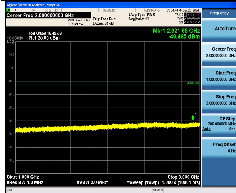
Band26 3MHz 16QAM 26740 1RB#14 1000~3000 1000~3000
