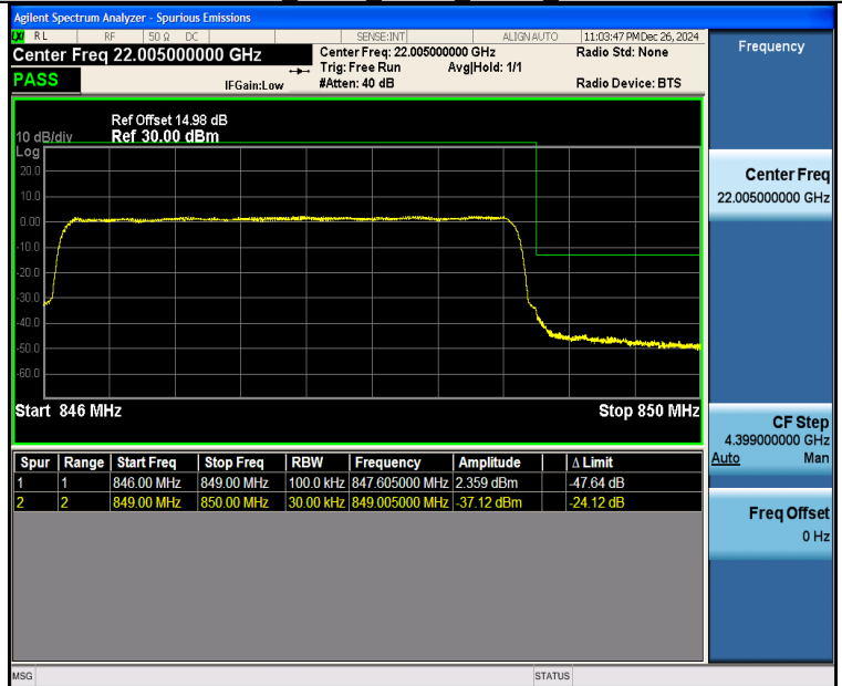
Band26 3MHz QPSK 27025 15RB#0
