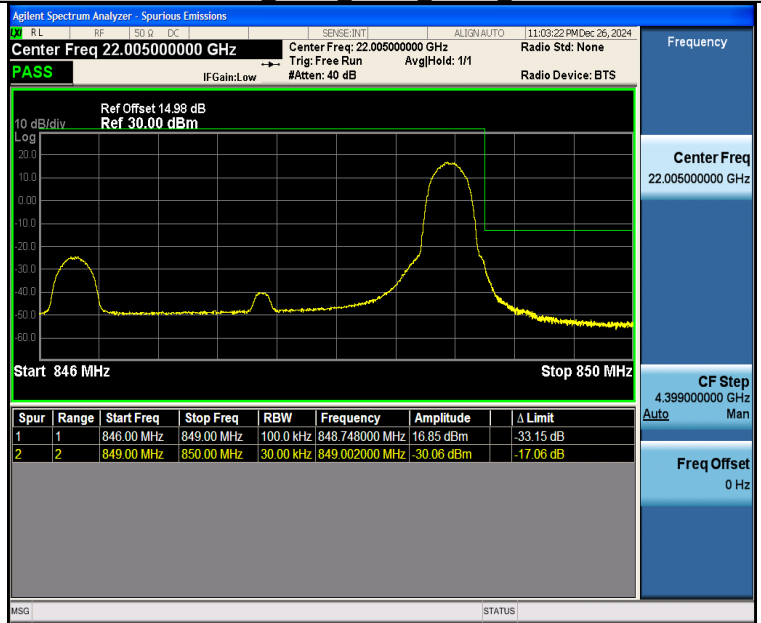
Band26 3MHz QPSK 27025 1RB#14
