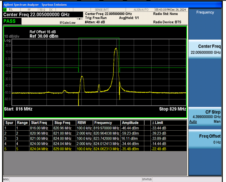
Band26_3MHz_QPSK_26775_1RB#14
