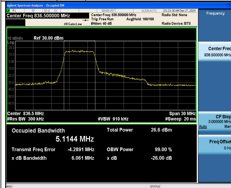
Band26(824-849)-15MHz-16QAM-26915-27RB#0-PASS
