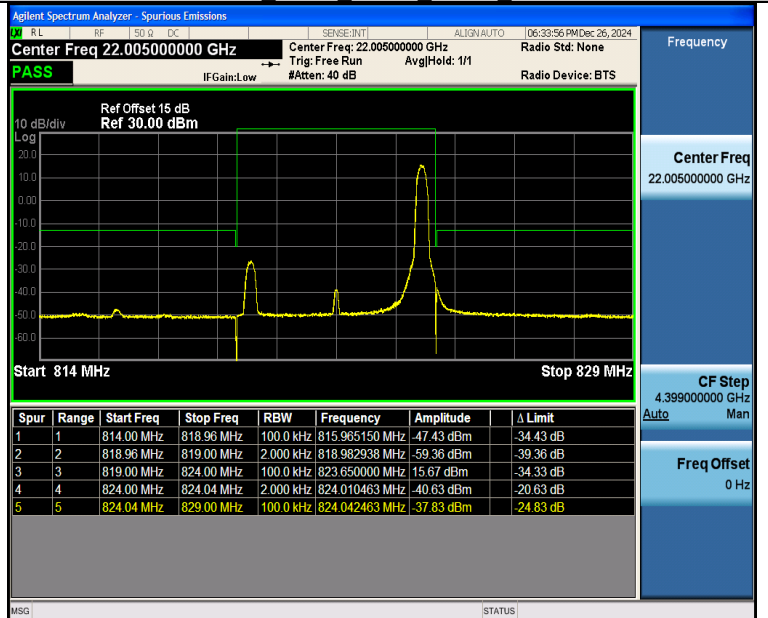
Band26_5MHz_QPSK_26765_1RB#24
