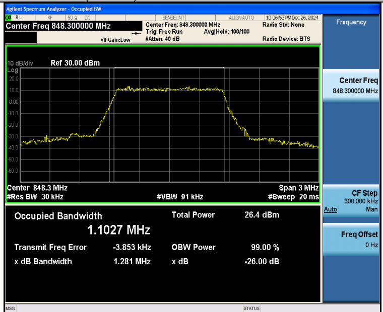
Band26(824-849)-1.4MHz-16QAM-27033-6RB#0-PASS
