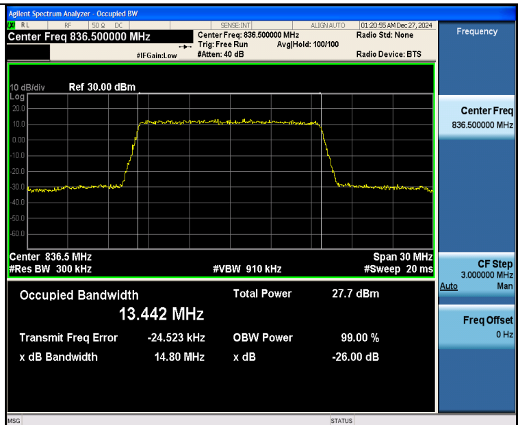
Band26(824-849)-15MHz-QPSK-26915-75RB#0-PASS
