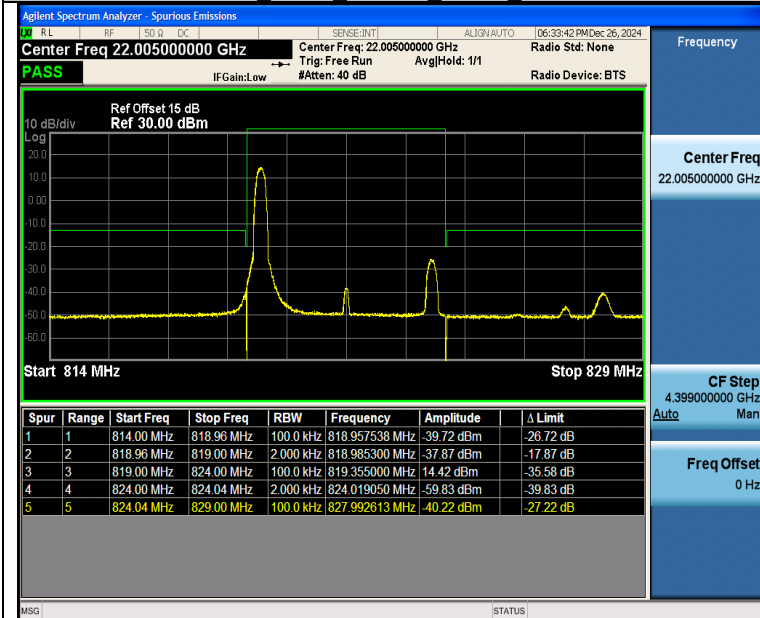
Band26_5MHz_16QAM_26765_1RB#0
