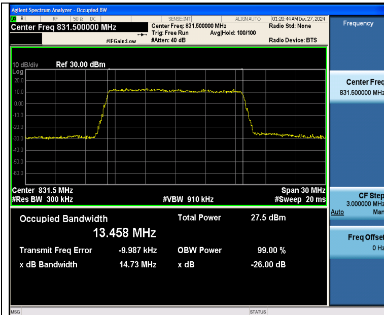
Band26(824-849)-15MHz-QPSK-26865-75RB#0-PASS
