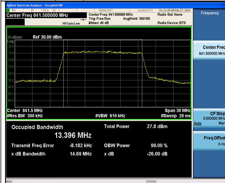
Band26(824-849)-15MHz-QPSK-26965-75RB#0-PASS
