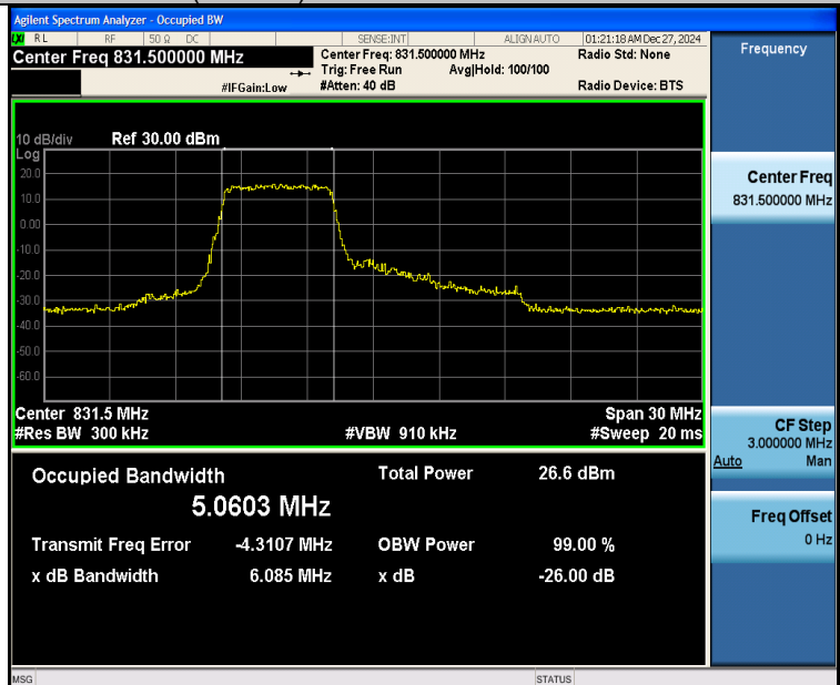
Band26(824-849)-15MHz-16QAM-26865-27RB#0-PASS
