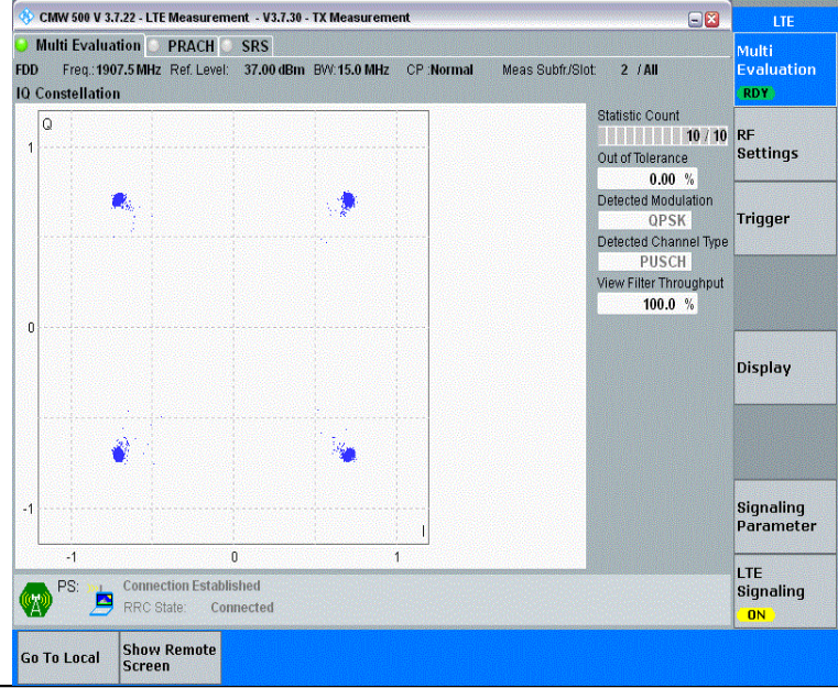
Band25-15MHz-QPSK-26615-75RB#0-PASS
