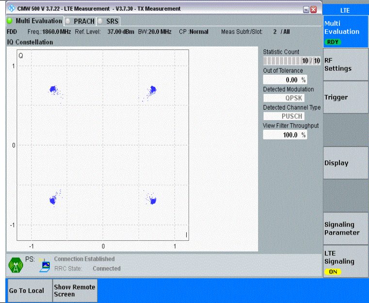
Band25-20MHz-QPSK-26140-100RB#0-PASS
