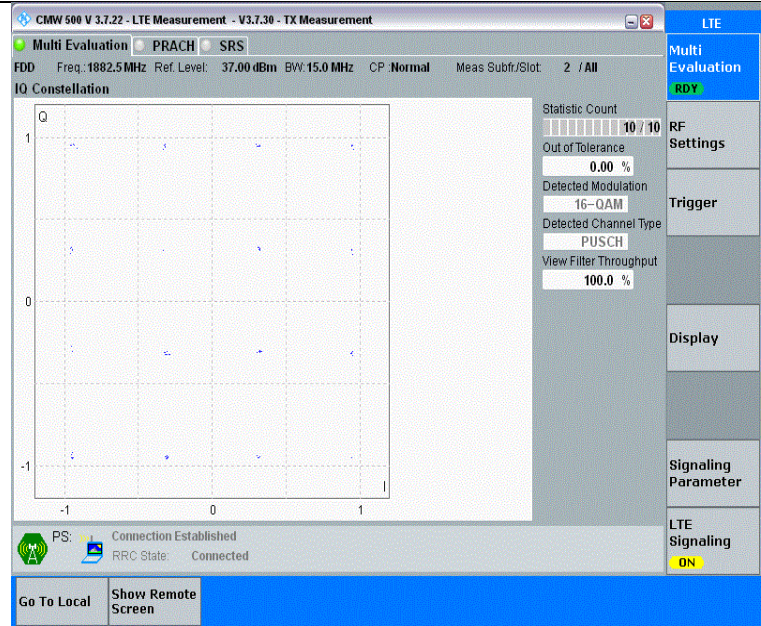
Band25-15MHz-16QAM-26365-1RB#0-PASS
