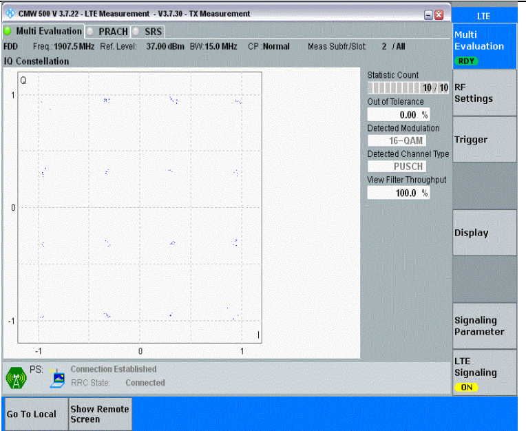
Band25-15MHz-16QAM-26615-1RB#0-PASS
