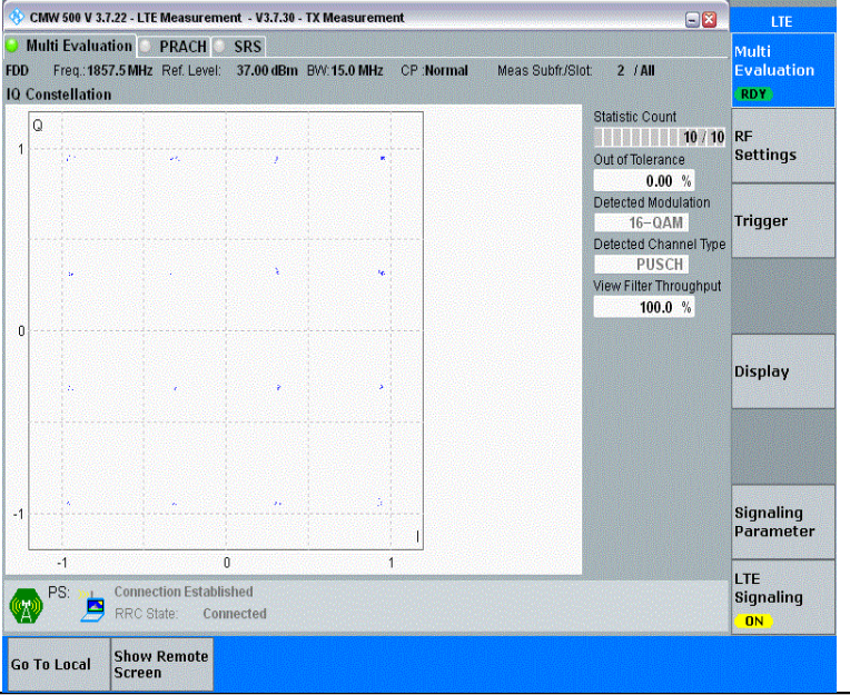
Band25-15MHz-16QAM-26115-1RB#0-PASS
