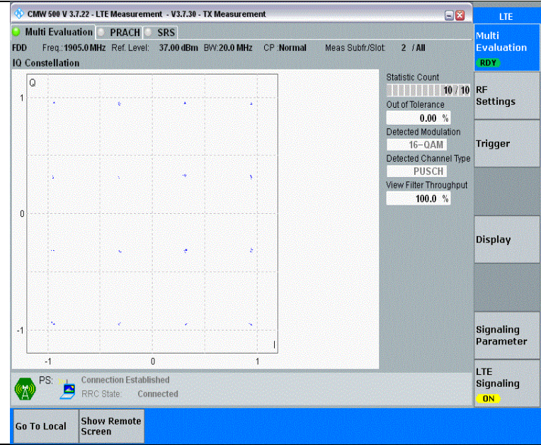
Band25-20MHz-16QAM-26590-1RB#0-PASS
