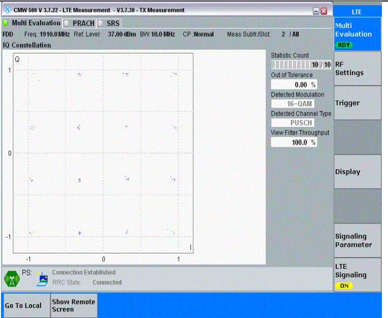
Band25-10MHz-16QAM-26640-1RB#0-PASS
