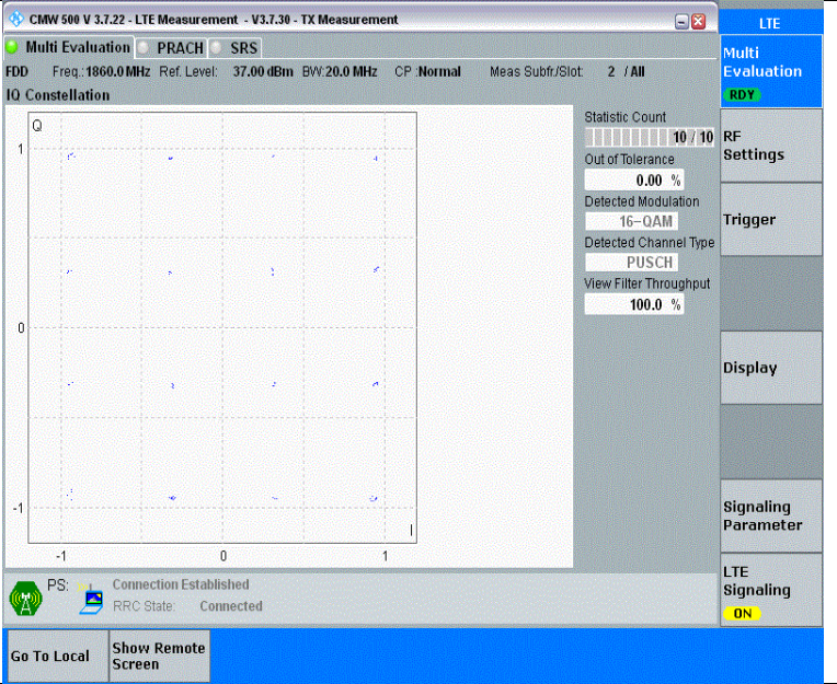
Band25-20MHz-16QAM-26140-1RB#0-PASS
