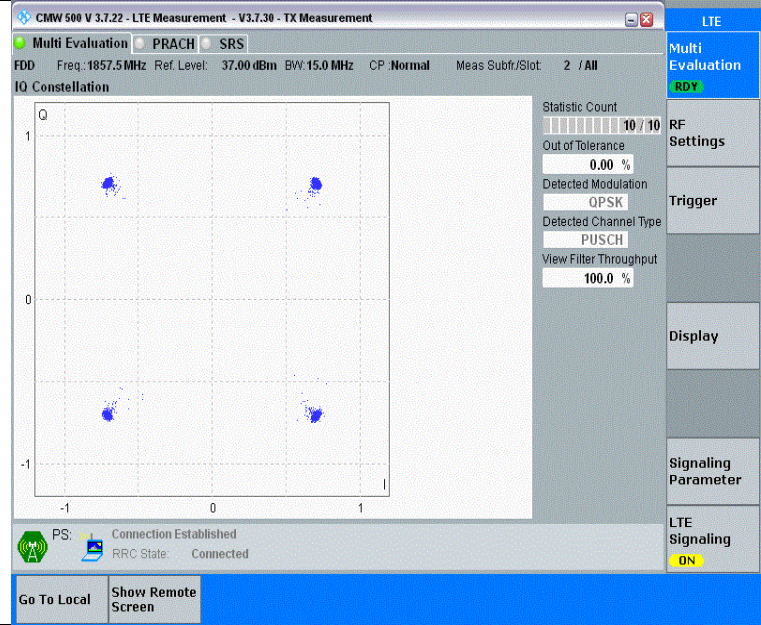
Band25-15MHz-QPSK-26115-75RB#0-PASS
