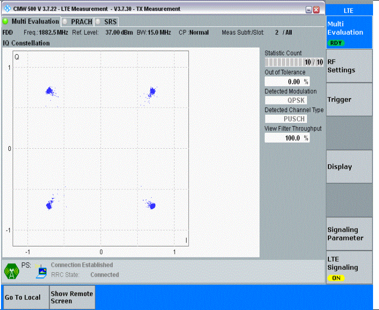
Band25-15MHz-QPSK-26365-75RB#0-PASS
