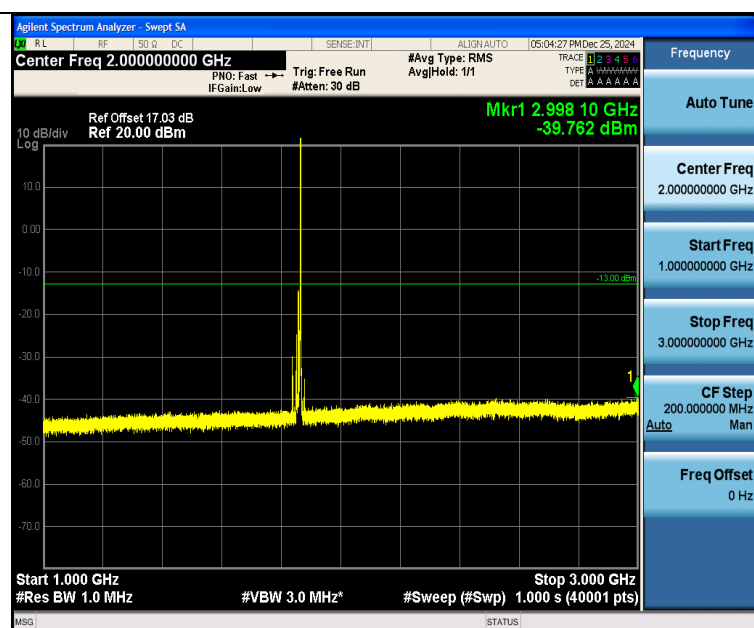
Band25_15MHz_QPSK_26115_1RB#74_1000~3000_1000~3000
