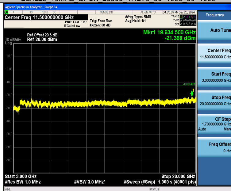
Band25_10MHz_QPSK_26365_1RB#0_3000~20000_3000~20000
