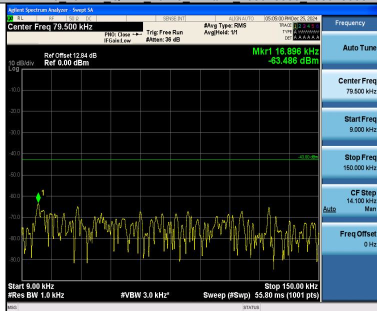
Band25_15MHz_16QAM_26115_1RB#74_0.009~0.15_0.009~0.15
