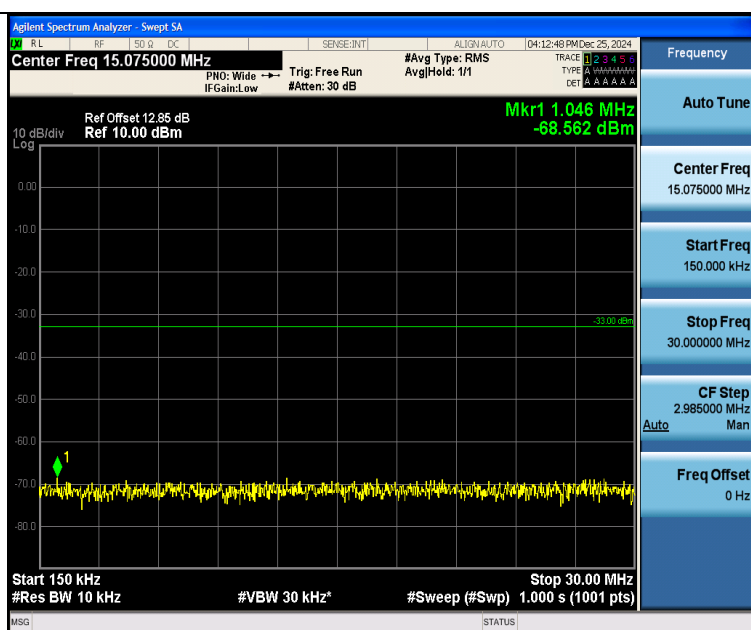
Band25_5MHz_QPSK_26665_25RB#0_0.15~30_0.15~30
