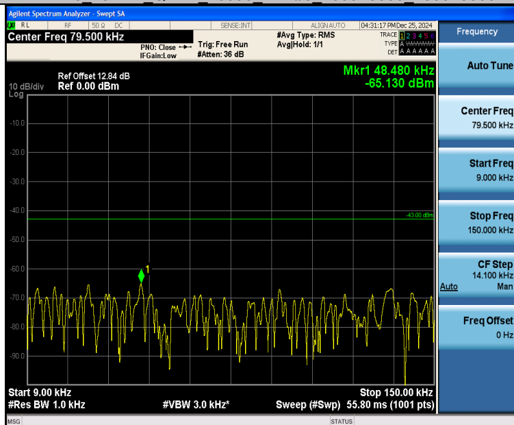
Band25_10MHz_16QAM_26090_1RB#0_0.009~0.15_0.009~0.15
