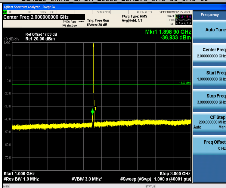
Band25_5MHz_QPSK_26665_25RB#0_1000~3000_1000~3000
