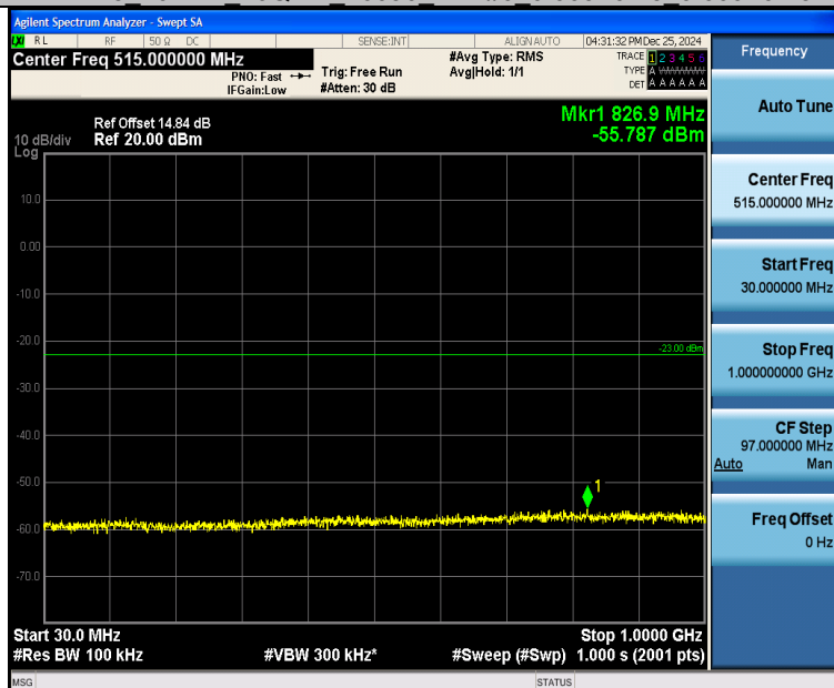
Band25_10MHz_16QAM_26090_1RB#0_30~1000_30~1000
