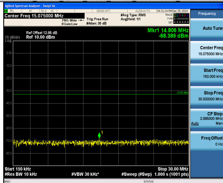
Band25_10MHz_16QAM_26090_1RB#0_0.15~30_0.15~30
