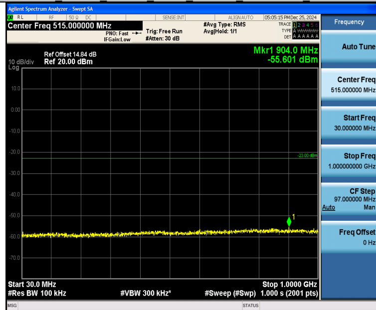
Band25_15MHz_16QAM_26115_1RB#74_30~1000_30~1000
