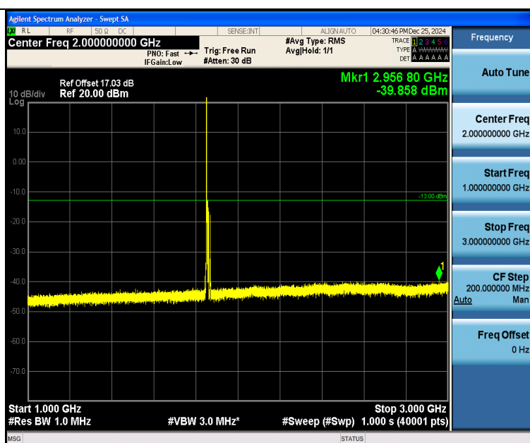
Band25_10MHz_QPSK_26090_1RB#0_1000~3000_1000~3000
