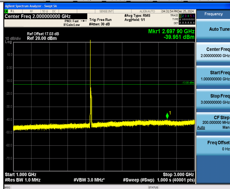
Band25_10MHz_16QAM_26090_1RB#0_1000~3000_1000~3000
