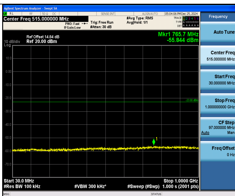
Band25_15MHz_QPSK_26115_1RB#74_30~1000_30~1000
