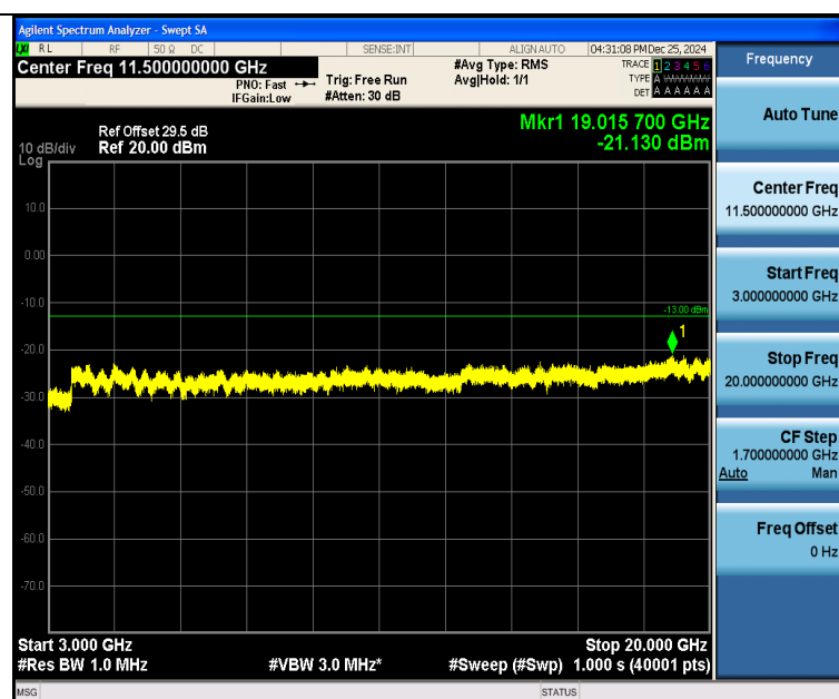
Band25_10MHz_QPSK_26090_1RB#0_3000~20000_3000~20000
