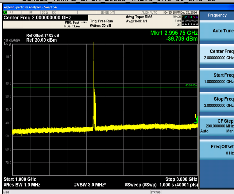
Band25_10MHz_QPSK_26365_1RB#0_1000~3000_1000~3000
