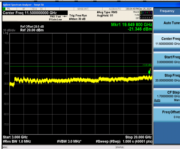
Band25_15MHz_QPSK_26115_1RB#74_3000~20000_3000~20000
