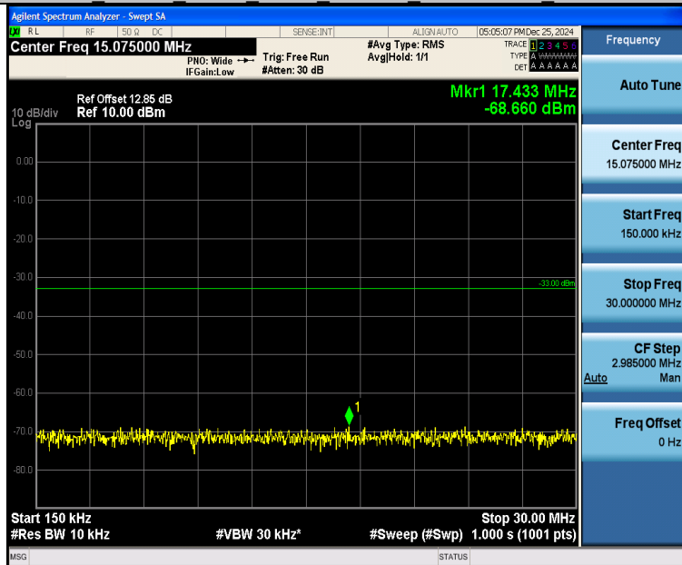
Band25_15MHz_16QAM_26115_1RB#74_0.15~30_0.15~30
