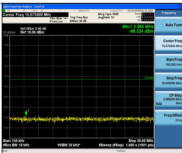
Band25_10MHz_QPSK_26365_1RB#0_0.15~30_0.15~30
