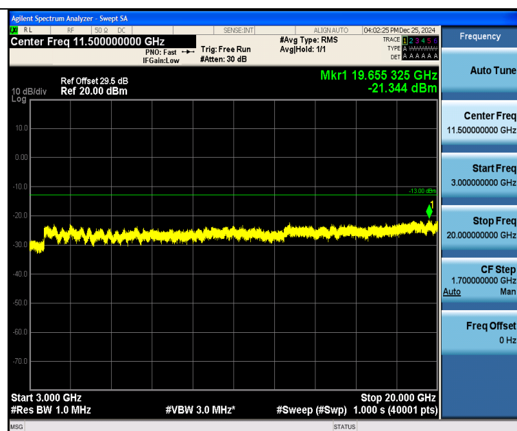
Band25_5MHz_QPSK_26365_1RB#0_3000~20000_3000~20000
