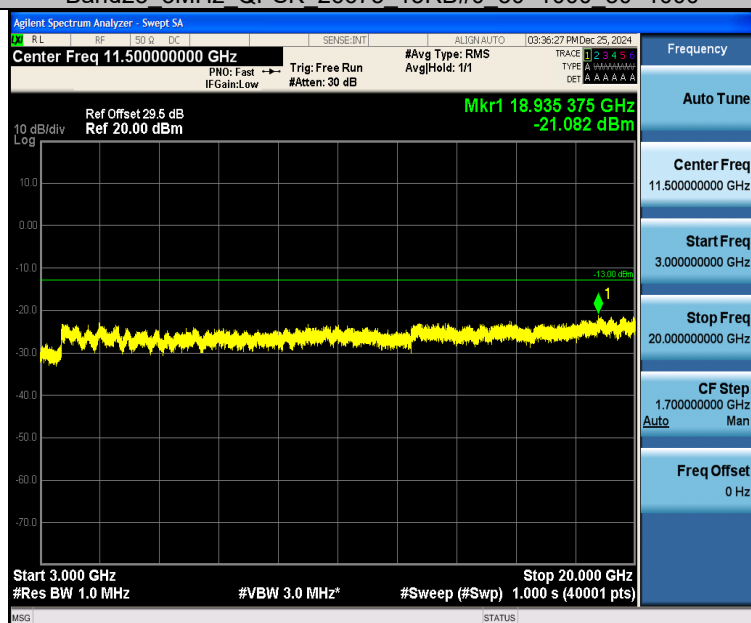
Band25_3MHz_QPSK_26675_15RB#0_3000~20000_3000~20000
