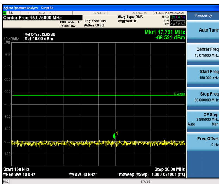
Band25_5MHz_QPSK_26365_25RB#0_0.15~30_0.15~30
