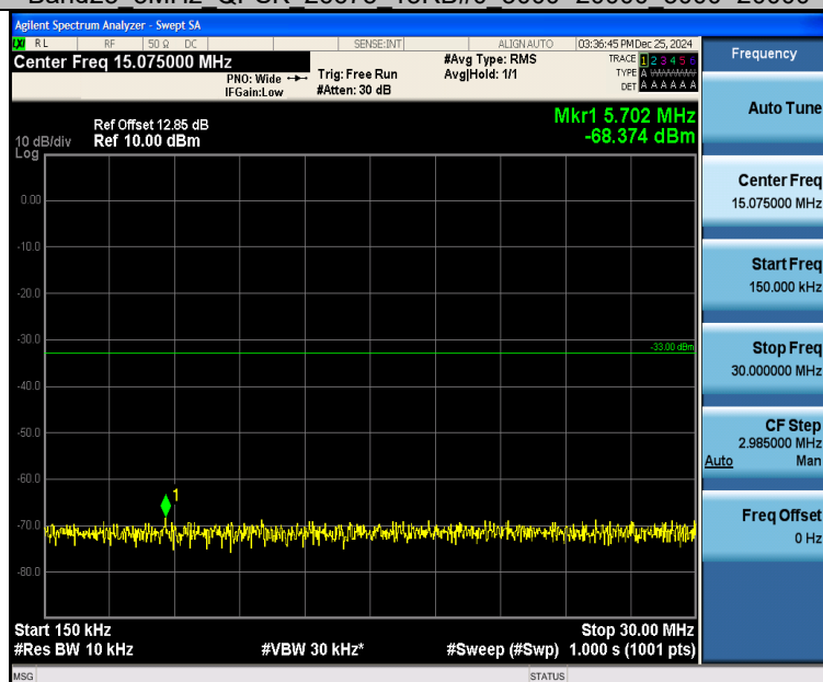
Band25_3MHz_16QAM_26675_15RB#0_0.15~30_0.15~30
