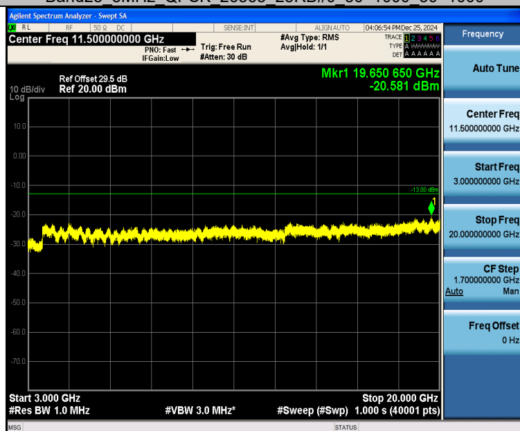
Band25_5MHz_QPSK_26365_25RB#0_3000~20000_3000~20000
