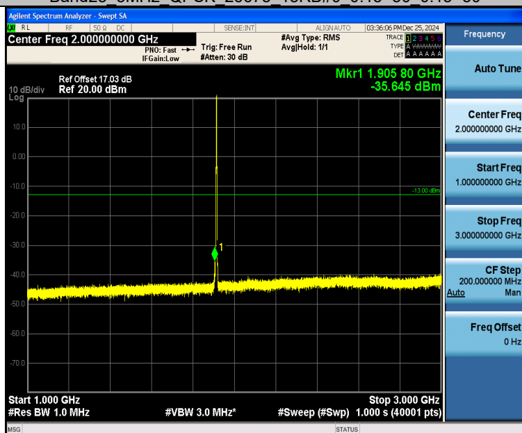
Band25_3MHz_QPSK_26675_15RB#0_1000~3000_1000~3000
