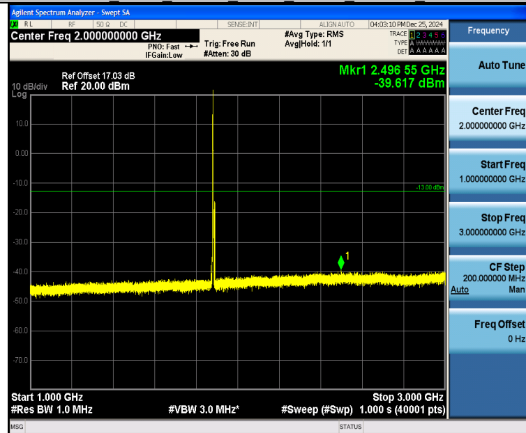
Band25_5MHz_16QAM_26365_1RB#0_1000~3000_1000~3000
