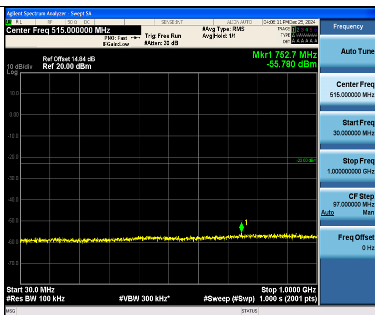
Band25_5MHz_QPSK_26365_25RB#0_30~1000_30~1000
