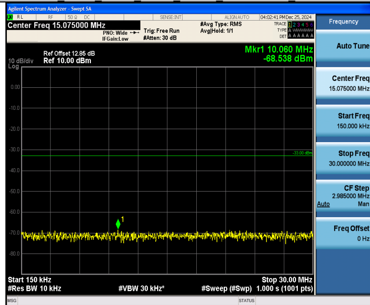
Band25_5MHz_16QAM_26365_1RB#0_0.15~30_0.15~30
