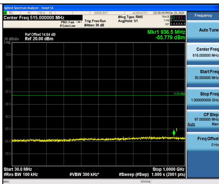
Band25 1.4MHz QPSK 26683 6RB#0 30~1000 30~1000
