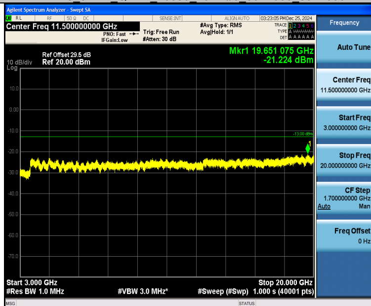
Band25_3MHz_QPSK_26055_15RB#0_3000~20000_3000~20000
