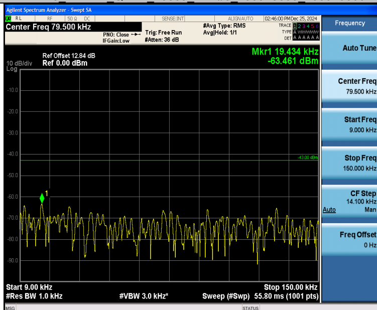
Band25 1.4MHz 16QAM 26365 1RB#0 0.009~0.15 0.009~0.15
