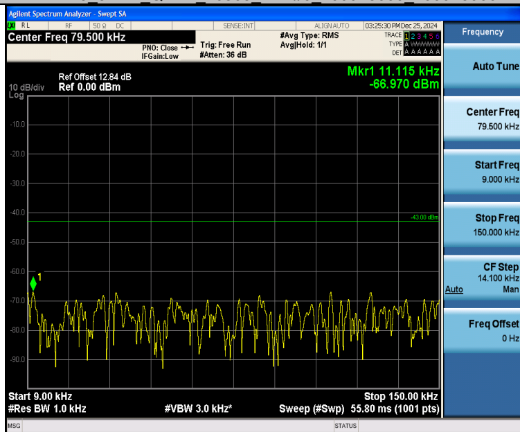
Band25 3MHz 16QAM 26365 1RB#0 0.009~0.15 0.009~0.15
