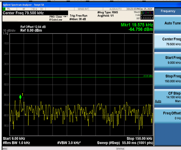
Band25_3MHz_16QAM_26055_15RB#0_0.009~0.15_0.009~0.15
