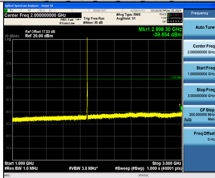
Band25 3MHz 16QAM 26365 1RB#0 1000~3000 1000~3000
