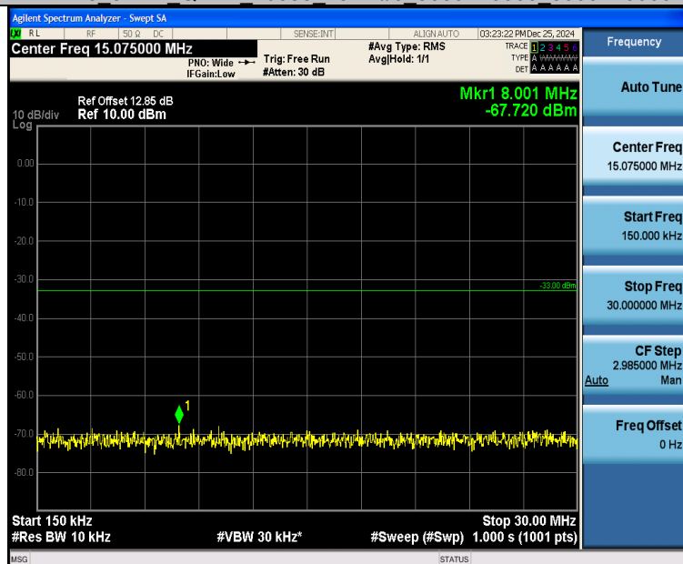
Band25_3MHz_16QAM_26055_15RB#0_0.15~30_0.15~30
