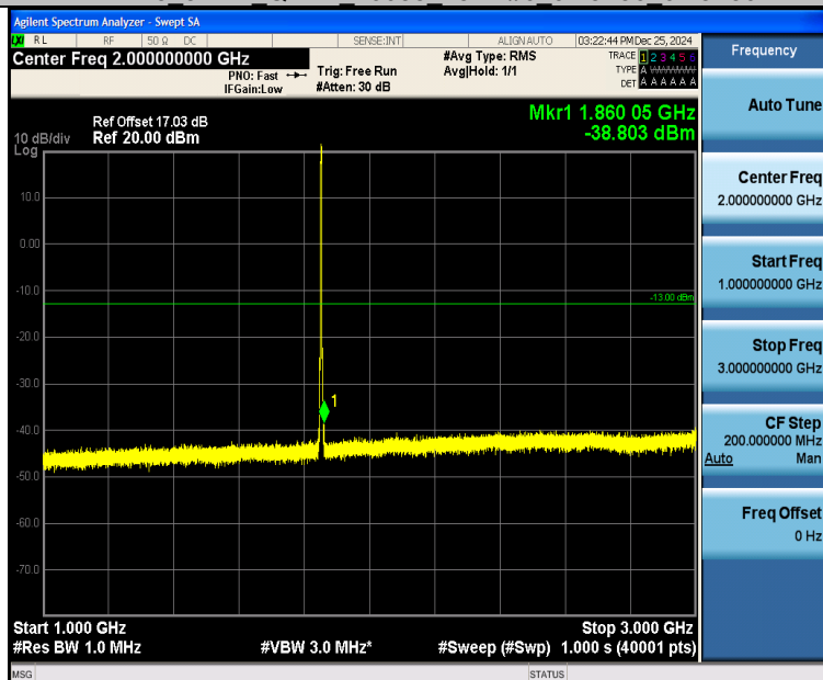
Band25_3MHz_QPSK_26055_15RB#0_1000~3000_1000~3000
