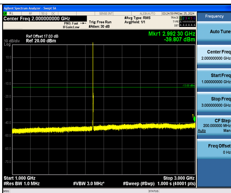
Band25 3MHz QPSK 26365 1RB#0 1000~3000 1000~3000
