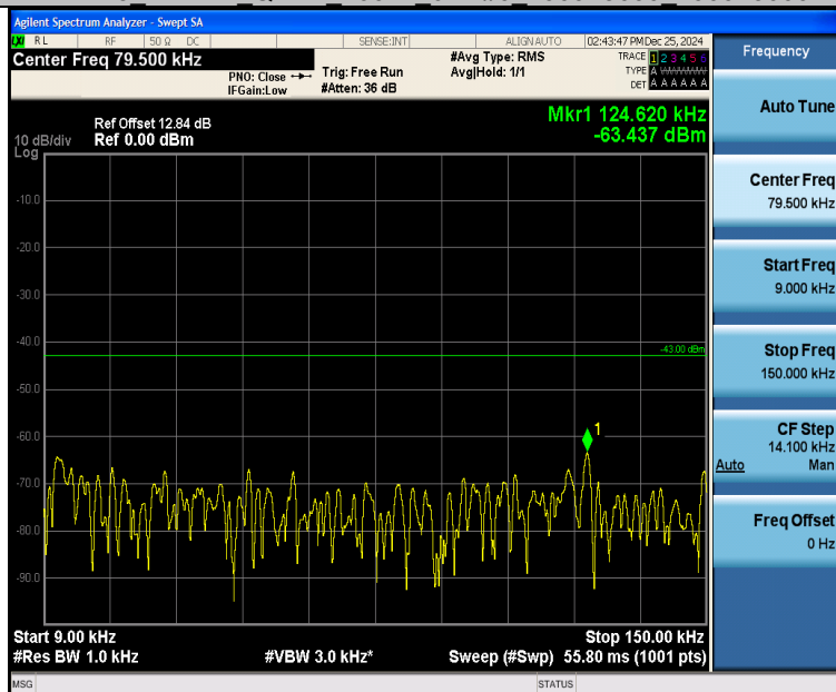
Band25 1.4MHz 16QAM 26047 6RB#0 0.009~0.15 0.009~0.15
