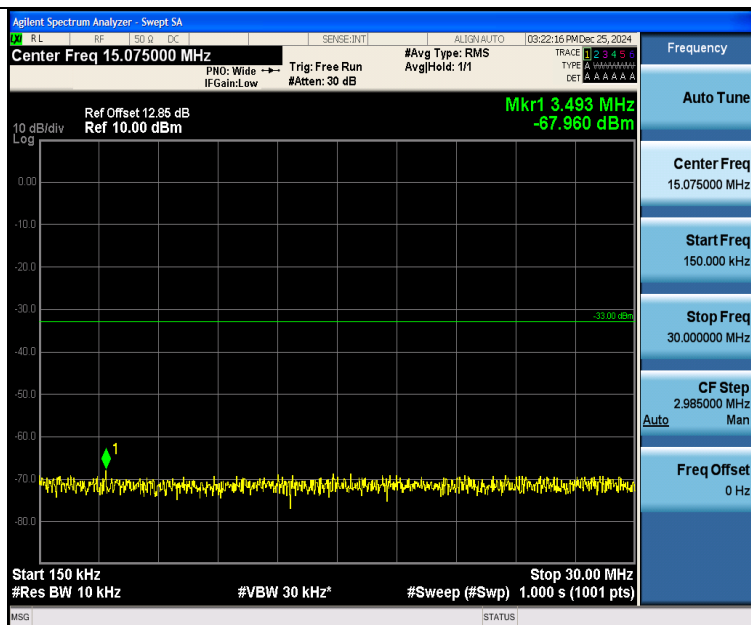
Band25_3MHz_QPSK_26055_15RB#0_0.15~30_0.15~30
