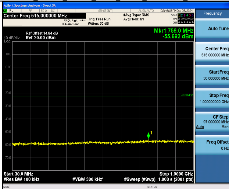
Band25 1.4MHz 16QAM 26365 1RB#0 30~1000 30~1000
