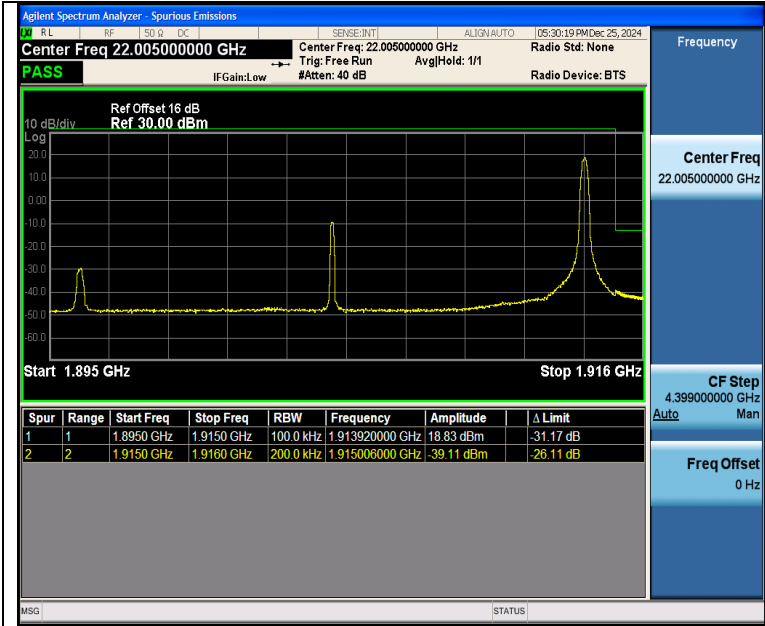
Band25_20MHz_16QAM_26590_1RB#99
