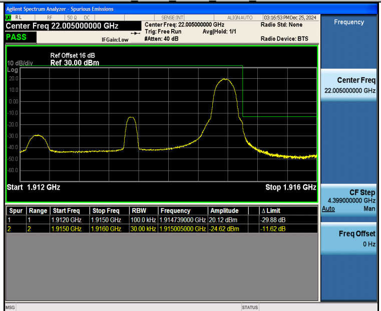
Band25_3MHz_QPSK_26675_1RB#14
