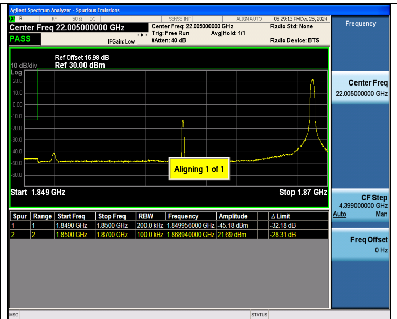
Band25_20MHz_QPSK_26140_1RB#99
