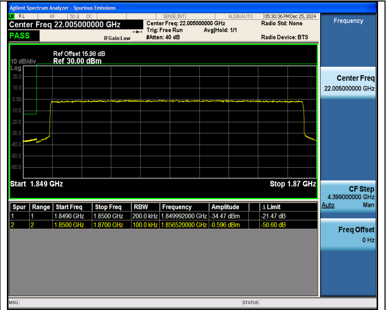
Band25_20MHz_QPSK_26140_100RB#0
