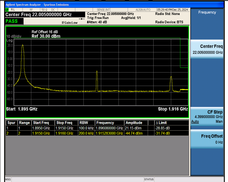
Band25_20MHz_QPSK_26590_1RB#0
