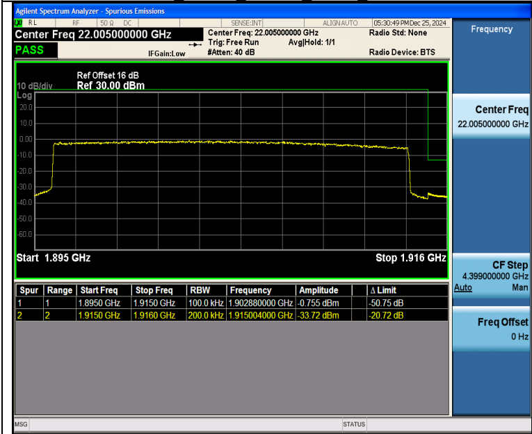
Band25_20MHz_QPSK_26590_100RB#0
