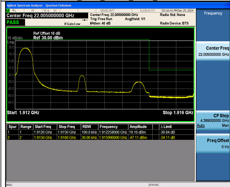
Band25_3MHz_16QAM_26675_1RB#0
