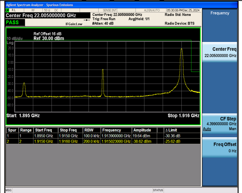
Band25_20MHz_QPSK_26590_1RB#99
