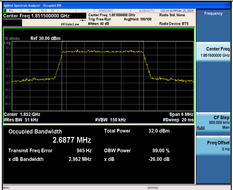
Band25-3MHz-16QAM-26055-15RB#0-PASS
