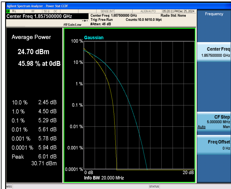
Band25-15MHz-QPSK-26115-75RB#0-PASS
