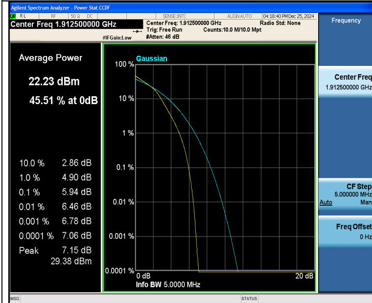
Band25-5MHz-16QAM-26665-25RB#0-PASS
