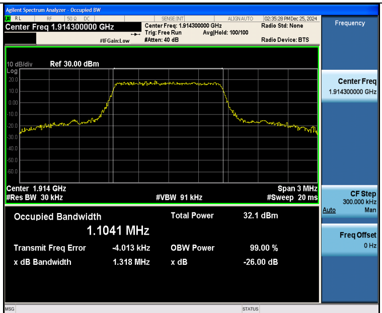
Band25-1.4MHz-16QAM-26683-6RB#0-PASS
