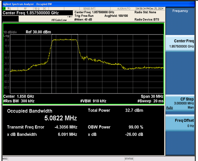
Band25-15MHz-16QAM-26115-27RB#0-PASS
