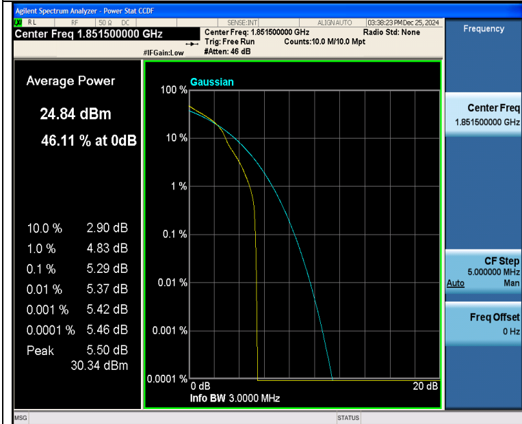
Band25-3MHz-16QAM-26055-1RB#0-PASS
