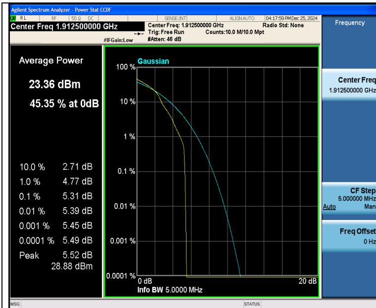
Band25-5MHz-16QAM-26665-1RB#0-PASS
