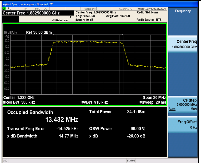
Band25-15MHz-QPSK-26365-75RB#0-PASS
