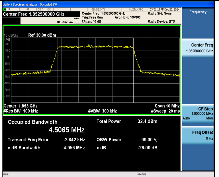
Band25-5MHz-16QAM-26065-25RB#0-PASS
