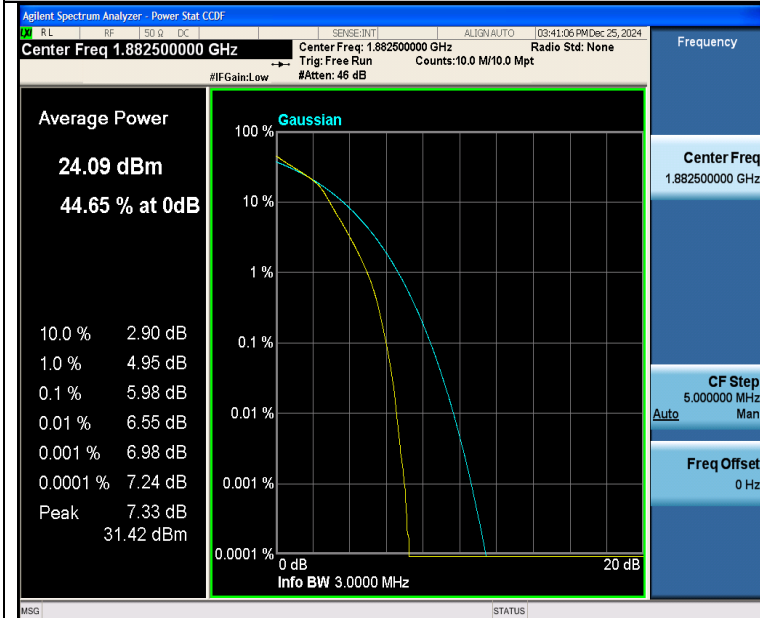
Band25-3MHz-16QAM-26365-15RB#0-PASS
