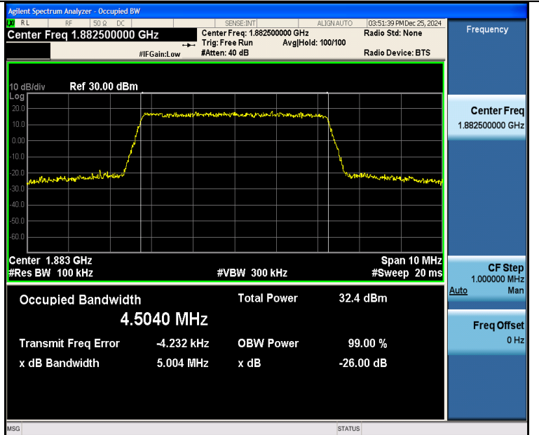
Band25-5MHz-16QAM-26365-25RB#0-PASS
