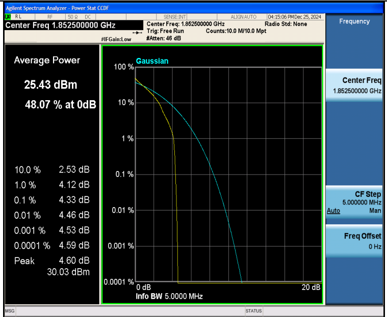
Band25-5MHz-QPSK-26065-1RB#0-PASS
