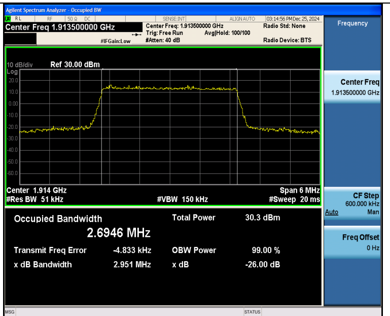
Band25-3MHz-16QAM-26675-15RB#0-PASS
