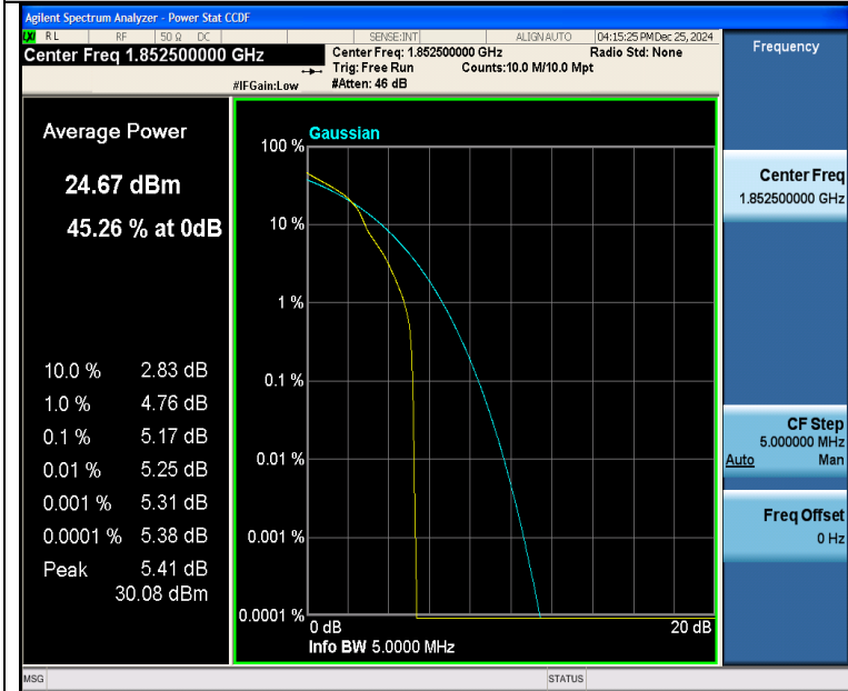
Band25-5MHz-16QAM-26065-1RB#0-PASS
