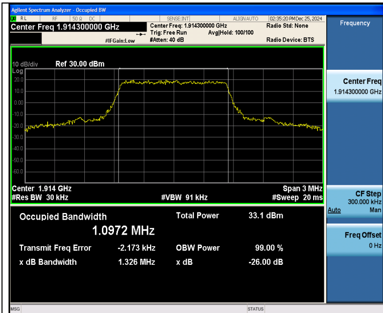
Band25-1.4MHz-QPSK-26683-6RB#0-PASS
