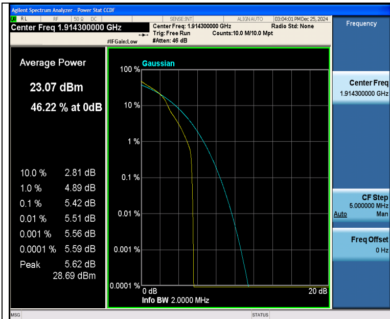
Band25-1.4MHz-16QAM-26683-1RB#0-PASS
