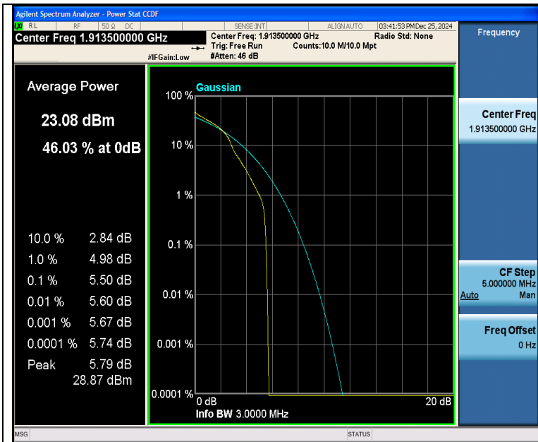
Band25-3MHz-16QAM-26675-1RB#0-PASS
