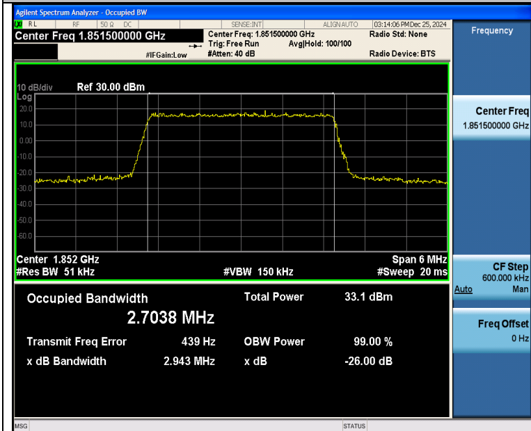
Band25-3MHz-QPSK-26055-15RB#0-PASS
