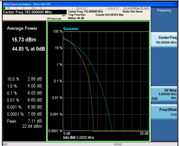
Band13-5MHz-16QAM-23230-25RB#0-PASS
