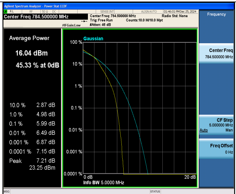
Band13-5MHz-16QAM-23255-25RB#0-PASS
