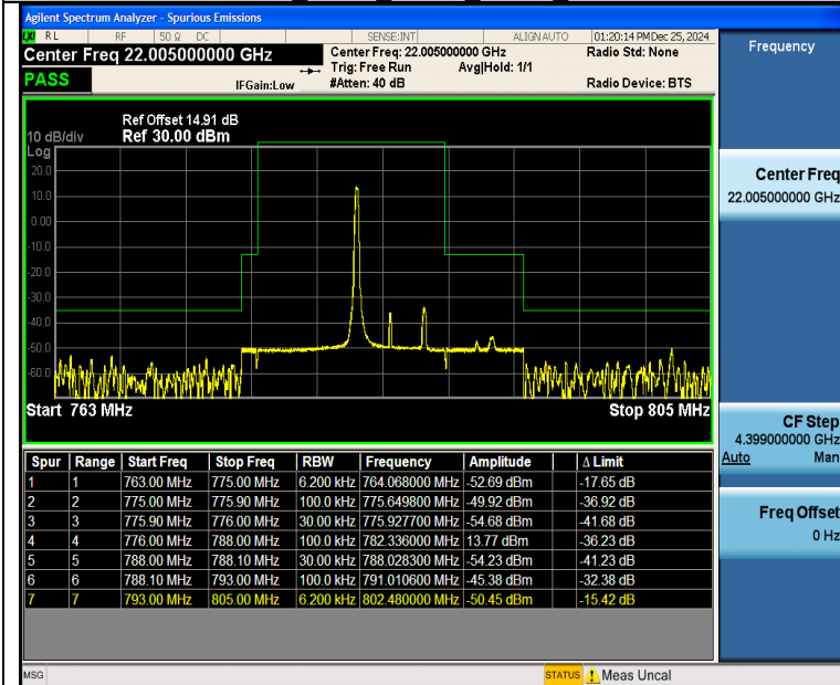
Band13_5MHz_QPSK_23255_1RB#0
