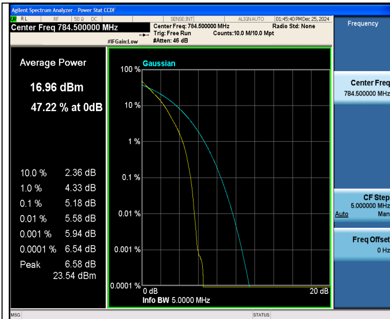
Band13-5MHz-QPSK-23255-25RB#0-PASS
