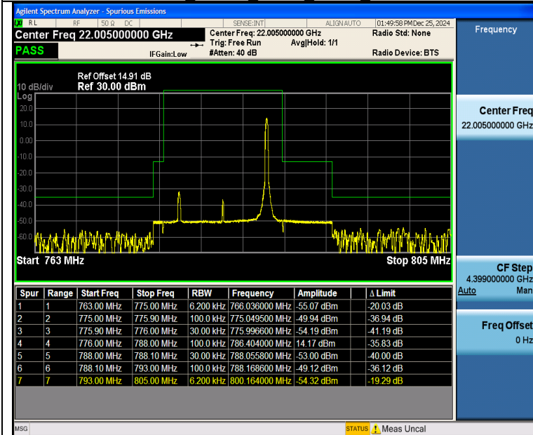
Band13 10MHz_QPSK_23230_1RB#49
