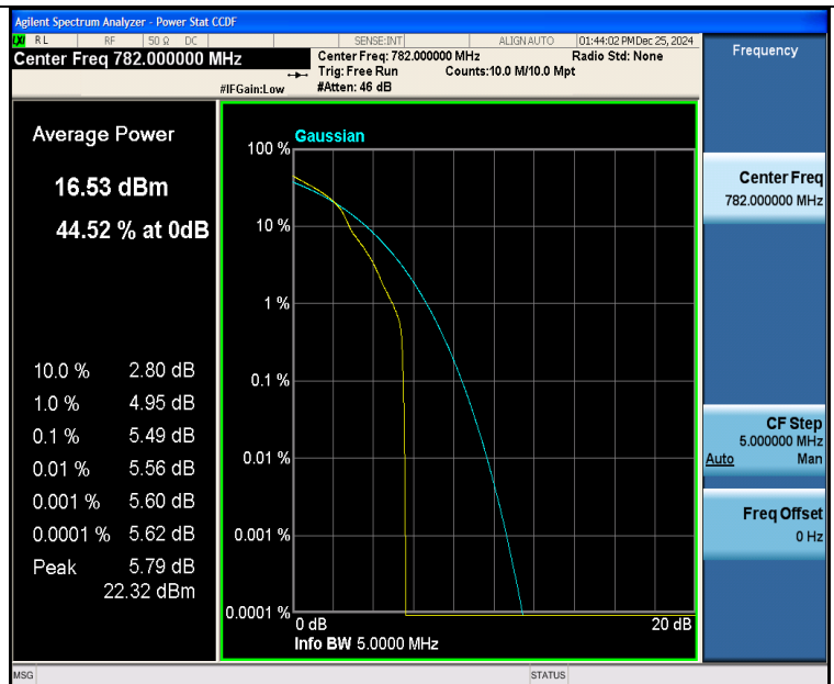
Band13-5MHz-16QAM-23230-1RB#0-PASS
