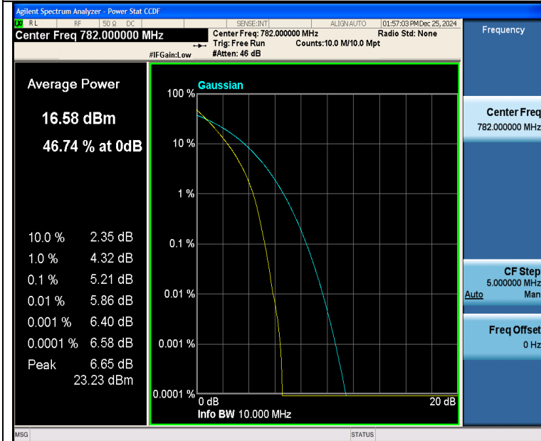
Band13-10MHz-QPSK-23230-50RB#0-PASS
