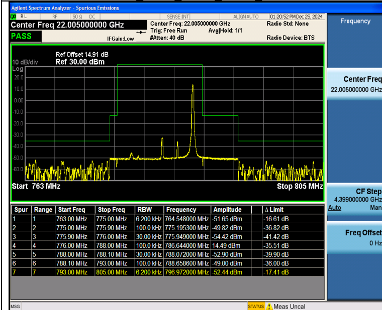
Band13_5MHz_QPSK_23255_1RB#24
