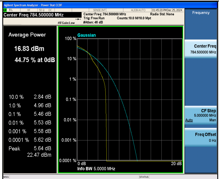
Band13-5MHz-16QAM-23255-1RB#0-PASS
