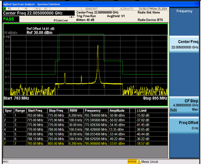
Band13 10MHz_16QAM_23230_1RB#49
