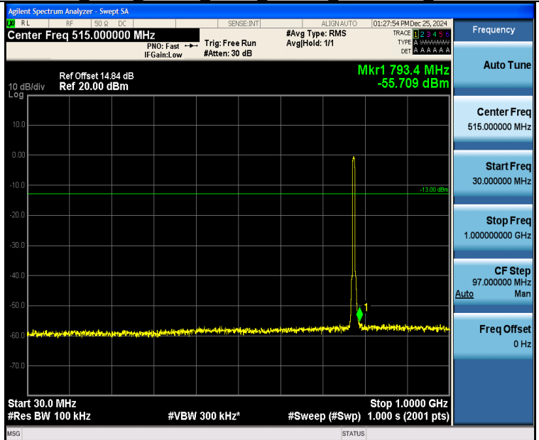
Band13_5MHz_16QAM_23205_25RB#0_30~1000_30~1000
