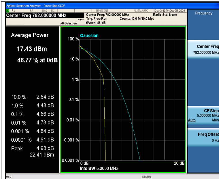
Band13-5MHz-QPSK-23230-1RB#0-PASS
