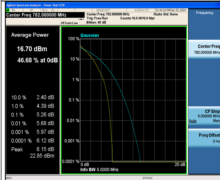
Band13-5MHz-QPSK-23230-25RB#0-PASS
