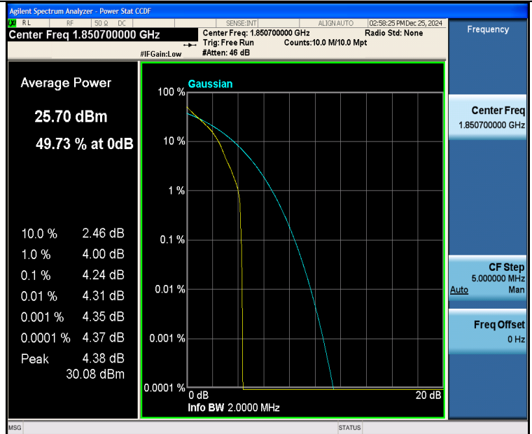
Band25-1.4MHz-QPSK-26047-1RB#0-PASS
