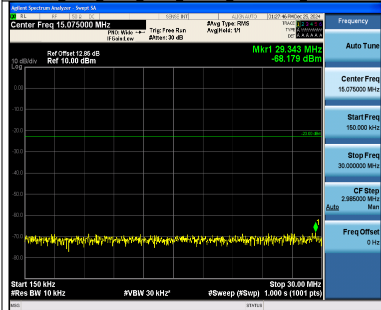
Band13_5MHz_16QAM_23205_25RB#0_0.15~30_0.15~30
