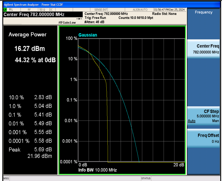
Band13-10MHz-16QAM-23230-1RB#0-PASS
