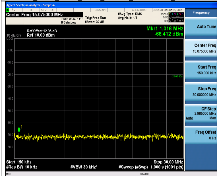
Band13_5MHz_16QAM_23230_25RB#0_0.15~30_0.15~30
