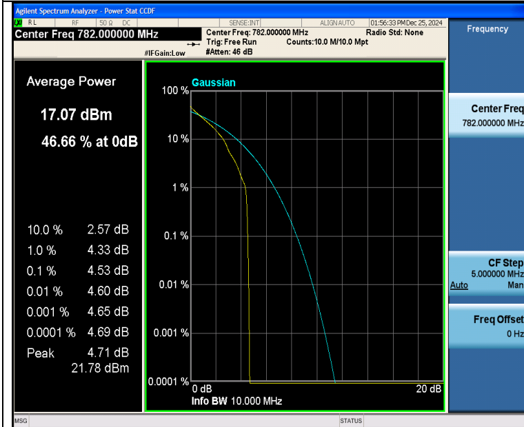
Band13-10MHz-QPSK-23230-1RB#0-PASS
