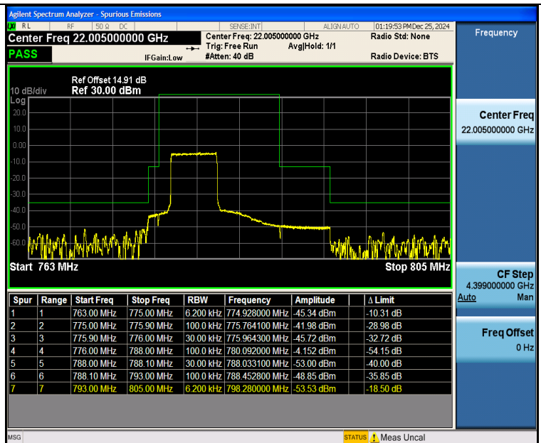
Band13_5MHz_16QAM_23205_25RB#0
