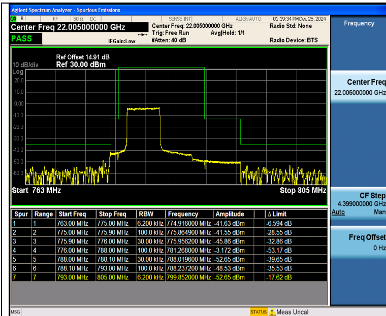
Band13_5MHz_QPSK_23205_25RB#0
