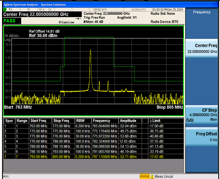
Band13_5MHz_16QAM_23255_1RB#0
