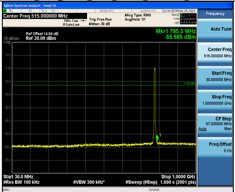
Band13_5MHz_16QAM_23230_25RB#0_30~1000_30~1000
