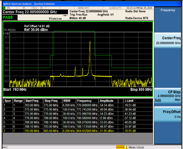
Band13_5MHz_16QAM_23255_1RB#24
