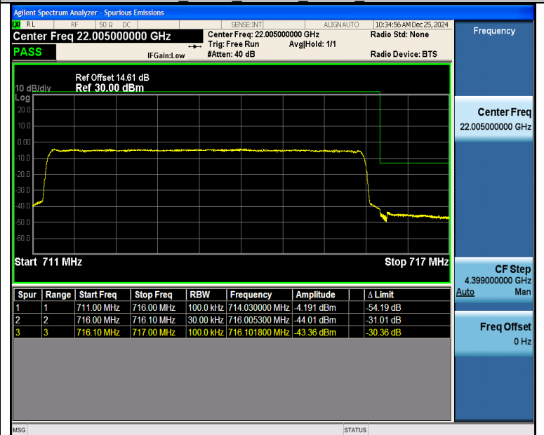
Band12_5MHz_16QAM_23155_25RB#0
