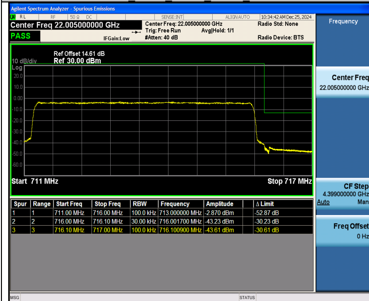
Band12_5MHz_QPSK_23155_25RB#0
