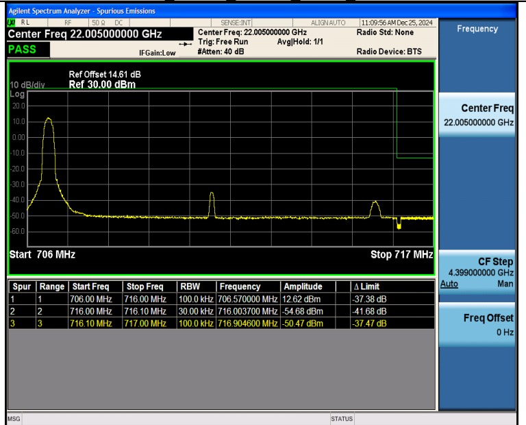
Band12_10MHz_16QAM_23130_1RB#0
