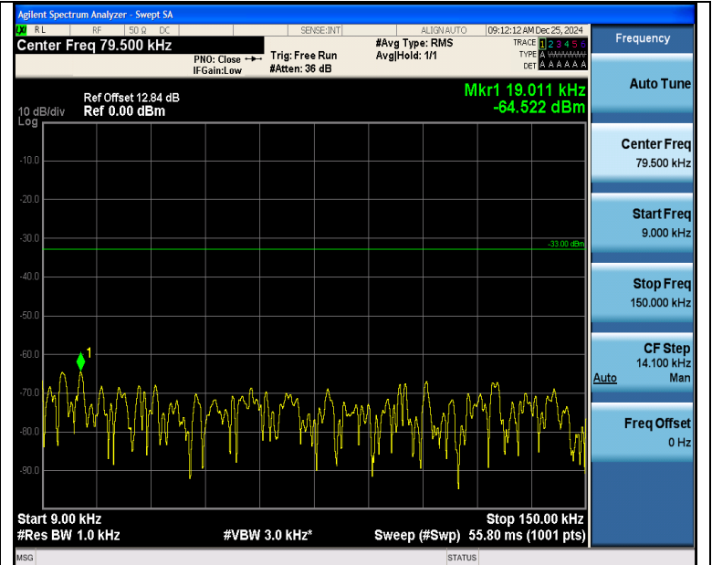
Band12_1.4MHz_QPSK_23017_1RB#0_0.009~0.15_0.009~0.15
